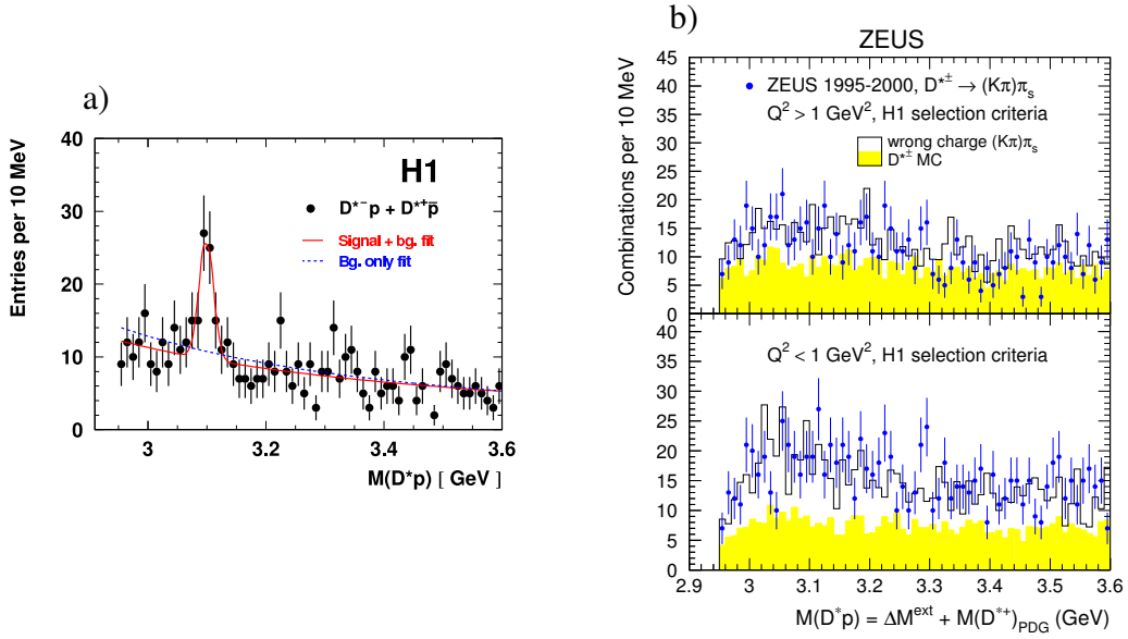
FIGURE 2. a) M(D^*p) mass distribution from opposite-charge D^*p combinations together with a fit of a background (dashed) and a background plus signal function (full line) measured by H1. b) M(D^*p) mass distribution observed by ZEUS for DIS (top) and \gamma p (bottom) events in the K\pi\pi_s decay channel.
