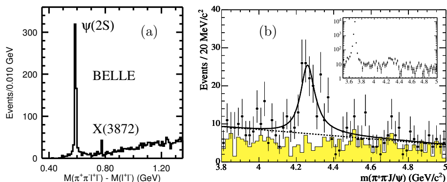
Fig. 5. (a) Distribution of M(\pi^+\pi^-l^+l^-) - M(l^+ - l^-) as observed by Belle for B -decay candidates. (b) The \pi^+\pi^-J/\psi invariant mass spectrum as observed in ISR events at BaBar. The inset shows the same spectrum over a wider range including the \psi(2S) resonance.
