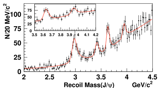
Fig. 4. The mass of the system recoiling against the reconstructed J/\psi .
