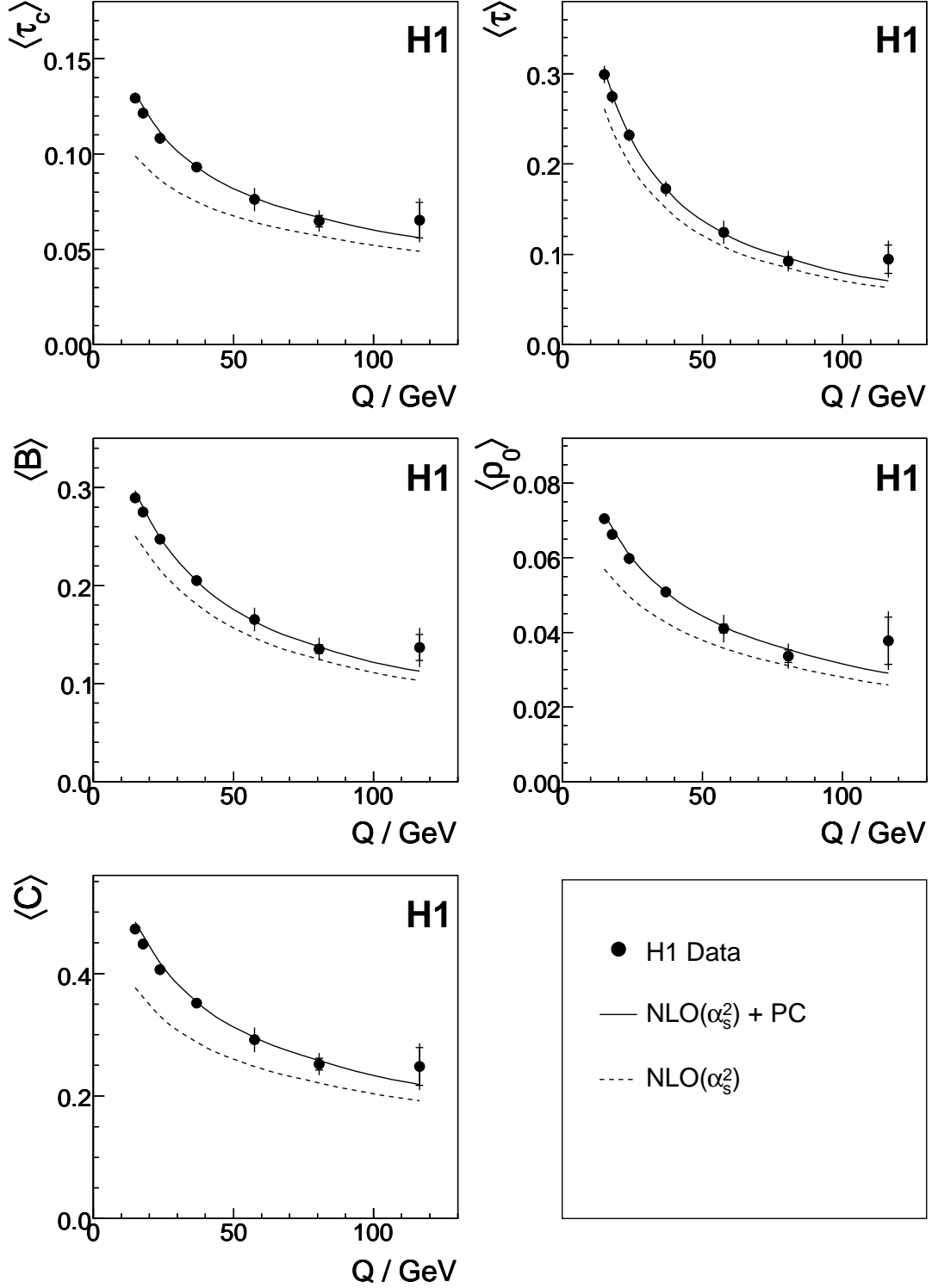
Figure 3: Mean values of event shape variables corrected to the hadron level as a function of the scale Q . The data, presented with statistical errors (inner bars) and total errors (outer bars), are compared with the results of NLO QCD fits including power corrections (PC). The dashed curves show the NLO QCD contribution to the fits.
