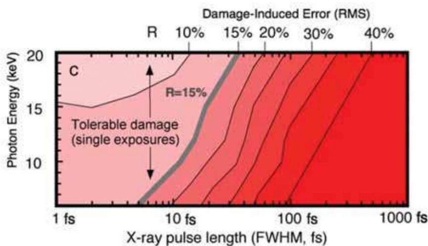
Figure 6.4.66 The landscape of damage tolerance as a function of x-ray energy and pulse length. The figure shows contour plots of expected damage-induced errors ( R ) as a function of x-ray energy when the total number of elastic scattering events per Carbon atom is held constant ( I_{\text{tot}} = 1.33 \times 10^{12} for 6 keV; 1.85 \times 10^{12} for 8 keV; 2.36 \times 10^{12} for 10 keV; 3.0 \times 10^{12} for 12 keV; 3.96 \times 10^{12} for 15 keV; and 6.0 \times 10^{12} for 20 keV x-ray photons/100 nm diameter). The weighted average R -factor describes the extent to which the information content of elastically scattered x-rays is degraded due to radiation damage during the exposure. We regard damage as acceptable if R \leq 15\% , and this value is shown as a grey contour line in the figure.
