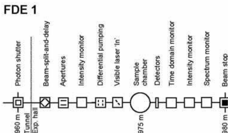
Figure 6.4.62 Schematic layout of the FDE 1 instrument at the SASE 1 beamline. Distances are given in relation to the end of the undulator.
