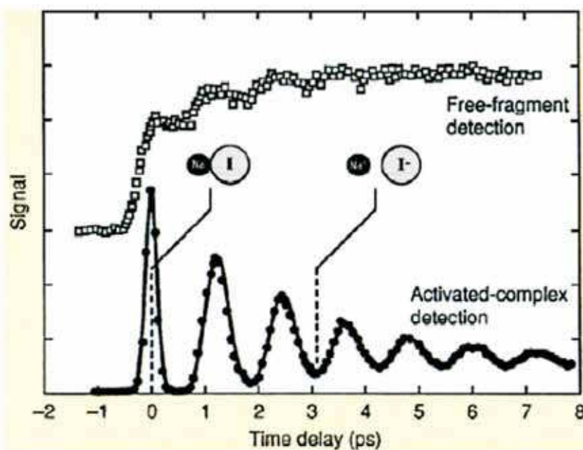
Figure 6.4.39 Wave packet dynamics evolution on the excited state adiabatic potential of NaI (black dots), observed in a pump-probe experiment. Atomic Sodium fragments detected on the dissociative channel of the ground state adiabatic potential curve (Figure 6.4.38). After [6-194].
