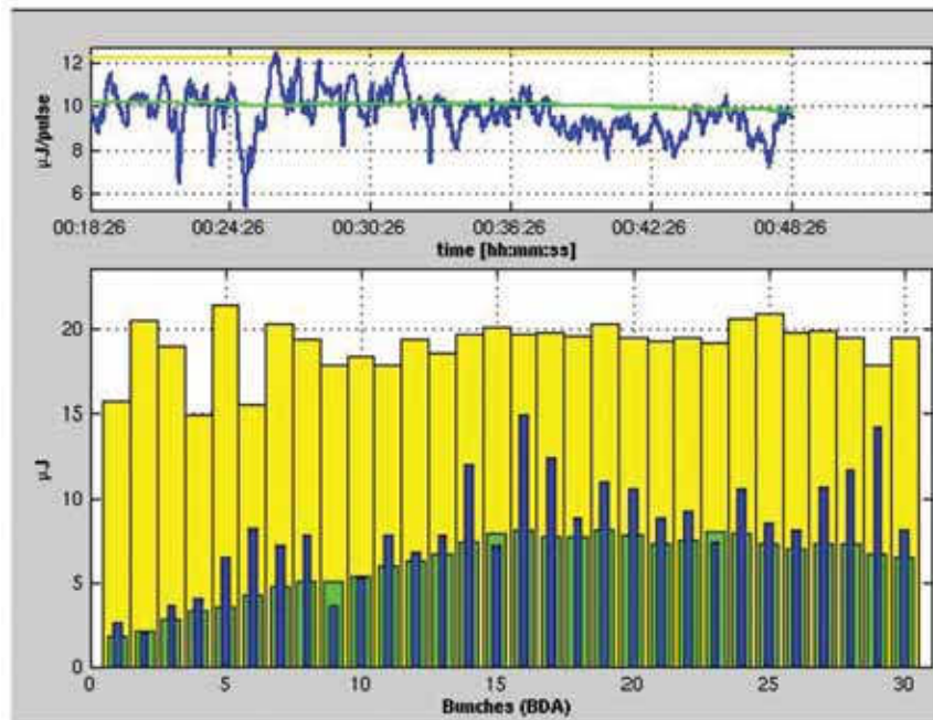
Figure 6.3.3 Diagnostic panel in the control system of FLASH showing the yield of the gas-monitor detector. Top: Averaged ion signal. Bottom: Pulse-resolved electron signal for 30 FEL pulses at 1 MHz repetition rate within one pulse train.
