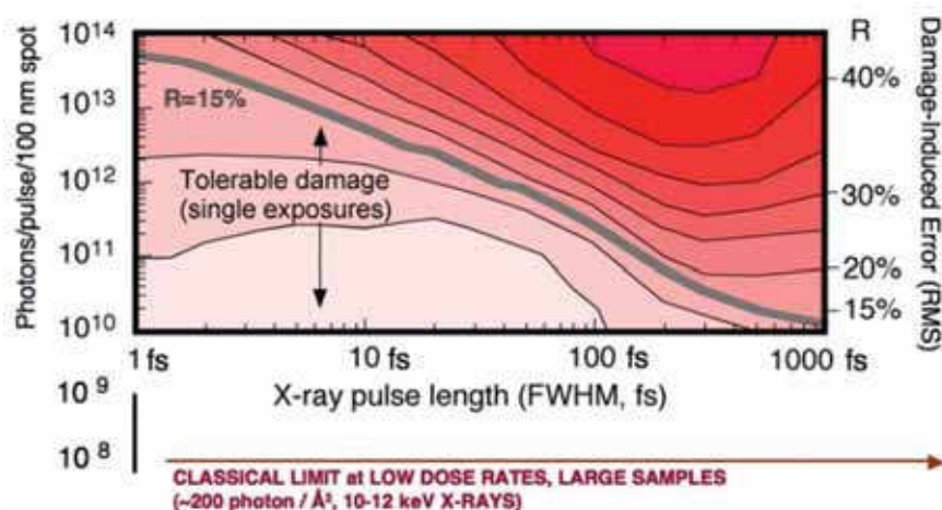
Figure 6.4.65 The landscape of damage tolerance as a function of pulse length and intensity. The figure shows contour plots of the expected damage-induced errors ( R ) in integrated diffraction patterns as a function of pulse duration and photon intensity for 12 keV x-rays. The weighted average R -factor describes the extent to which the information content of elastically scattered x-rays is degraded due to radiation damage during the exposure (0% = no change in the structure, 67% = structure randomised). We regard damage as acceptable if R \leq 15\% , and this value is shown as a grey contour line in the figure.
