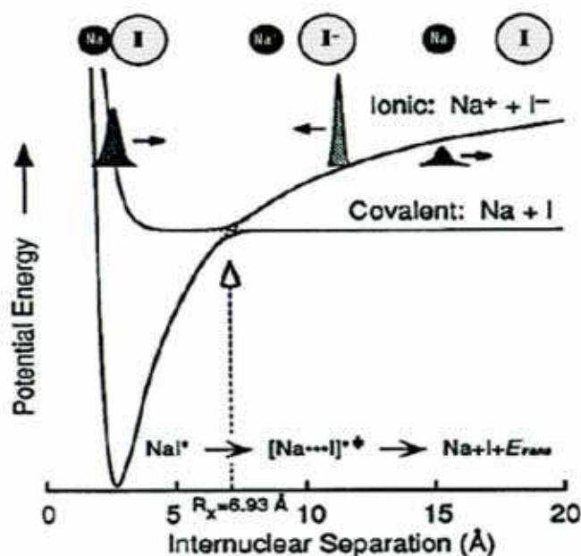
Figure 6.4.38 Potential curves of the NaI molecule and principle of the pump-probe experiment. Femtosecond excitation creates a vibrational wave packet (Gaussian on the left) in the excited state, which will then evolve between the left and right turning points. In so doing, the wave packet passes by the point of crossing and part of it leaks via the dissociative channel giving Sodium and Iodine neutral fragments. After ref [6-194].
