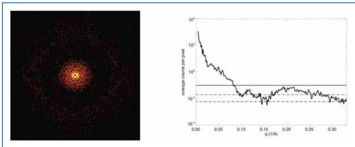
Figure 6.4.77 Simulated diffraction data from the (CPMV test object, for a beam waist diameter of 0.2\ \mu\text{m} . Total photon number in the incident beam was 10^{12} . The array is 422 \times 422 pixels, corresponding to s=2 , and a resolution of 1/(0.3\ \text{nm}) . The central 4 \times 4 pixels were blocked. Total integrated photons are 7.3 \times 10^4 . The intensities are displayed on a logarithmic greyscale. Away from the centre most pixels have one or no photons. The maximum photon count is 1,530. The plot shows the radial average of the photon counts. The solid line is at 0.1 counts, the minimum counts needed to classify [6-331], and the dotted lines denote the noise level for 10 and 100 averages, for a detector noise of 0.06.
