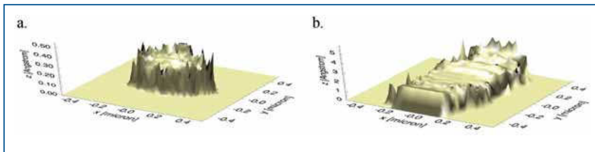
Figure 6.2.2 Ray-tracing of focus and wave front deformation for the case of extreme focusing using KB-mirrors in front of the sample. 0.01\ \mu\text{rad} (a) and 0.1\ \mu\text{rad} (b) rms slope errors have been assumed for the double-mirror system at 500 m.
