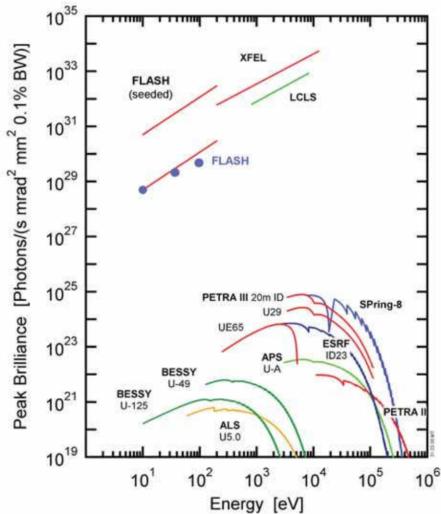
Figure 1.2.2 Peak brilliance of XFELs versus third generation SR light sources. Blue spots show experimental performance of the FLASH at the DESY.
