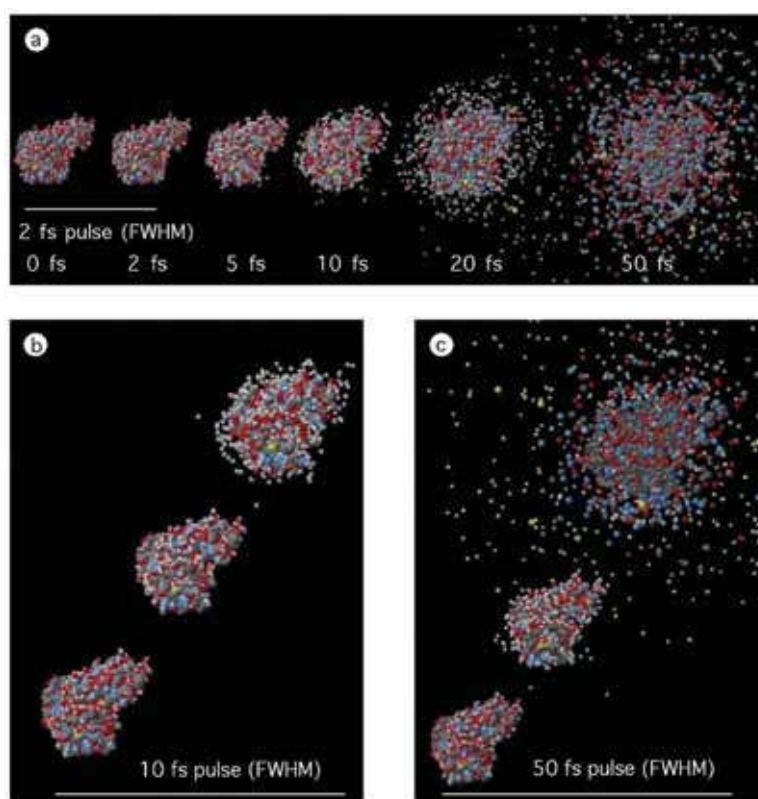
Figure 6.4.64 MD simulation of radiation-induced Coulomb explosion of a small protein (lysozyme). White balls: H, Grey: C, Blue: N, Red: O, Yellow: S. Integrated x-ray intensity: 3 \times 10^{12} (12 keV) photons/100 nm diameter spot (corresponding to 3.8 \times 10^8 photons/nm 2 , or 3.8 \times 10^6 photons/Å 2 on the sample) in all cases. (a) Protein exposed to a 2 fs FWHM x-ray pulse, and disintegration followed in time. The atomic positions in the first two structures (before and after the pulse) are practically identical at this pulse length due to an inertial delay in the explosion. (b) Lysozyme exposed to the same number of photons as in (a) but the pulse FWHM is now 10 fs. The images show the structure at the beginning, in the middle and near the end of the x-ray pulse. (c) Behaviour of the protein during a 50 fs FWHM x-ray pulse. It is also apparent from the figure that during the Coulomb explosion, Hydrogen ions and highly ionised sulphurs are the first to escape the immediate vicinity of the protein (at 12 keV, the photoelectric cross-section for Sulphur is about 50 times larger than that for Carbon). Based on [6-319].
