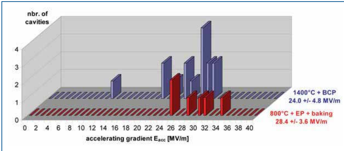
Figure 4.2.5 Comparison of the accelerating gradients at Q_0=10^{10} in the first performance test after the full preparation sequences using etching with post-purification at 1,400 °C (blue) and EP with 800 °C annealing (red).
