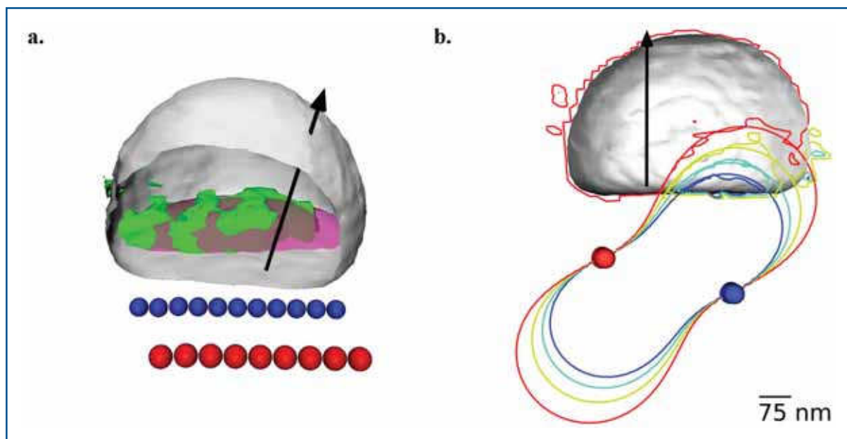
Figure 6.4.19 (a) Single isosurface of the phase and the best fit superimposed on a cut-away image of the crystal density. The point defect lines used to generate the fit (dots) and the direction of Q (arrow) are also illustrated; (b) contour map of the cross section of the reconstructed phase of the complex density function on a plane passing through the middle of the nanocrystal. Smooth lines are the corresponding contours of the projection function \vec{Q} \cdot \vec{u}(r) , where u(r) is the strain field calculated for two rows of point defects (balls) of opposite sign. Both sets of contours have spacing of 0.24 rad.
