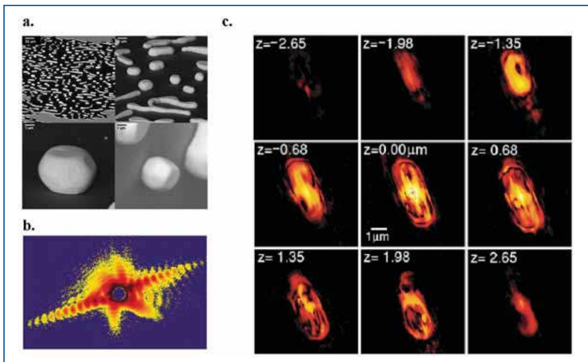
Figure 6.4.17 (a) Scanning Electron Microscope (SEM) image of Gold particles that are obtained after annealing at 950^\circ\text{C} for 70 hours; (b) coherent x-ray diffraction pattern from one of these crystals; (c) the 2-D slices through the best fit 3-D reconstructed density, separated as labelled.
