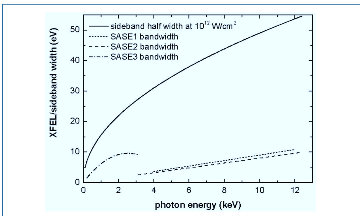
Figure 6.3.5 Calculated spectral sideband half-width at 10^{12} \text{ W/cm}^2 laser intensity in comparison with expected bandwidths of various XFEL branches.
