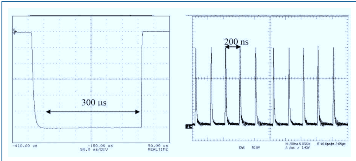
Figure 4.7.4 Left: Pulse current of the flat-top kicker with an amplitude stability of better than 1% over a pulse length of 300 \mu\text{s} . The fall-time is only 5 \mu\text{s} . Right: Pulse form of 5 MHz single-bunch kicker.
