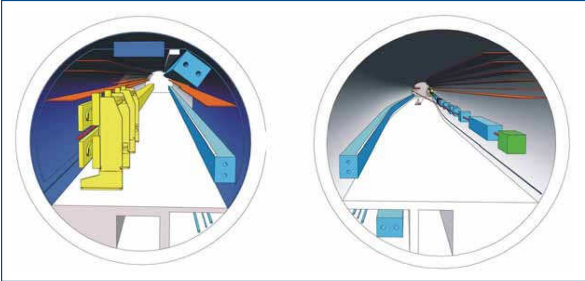
Figure 7.1.16 Cross sectional view of the tunnel in the region of the SASE undulators as viewed in the beam direction. The diameter of the tunnel is determined by the transport path for a replacement undulator module and the necessary emergency pathway (see position A-A in Figure 7.1.15).
