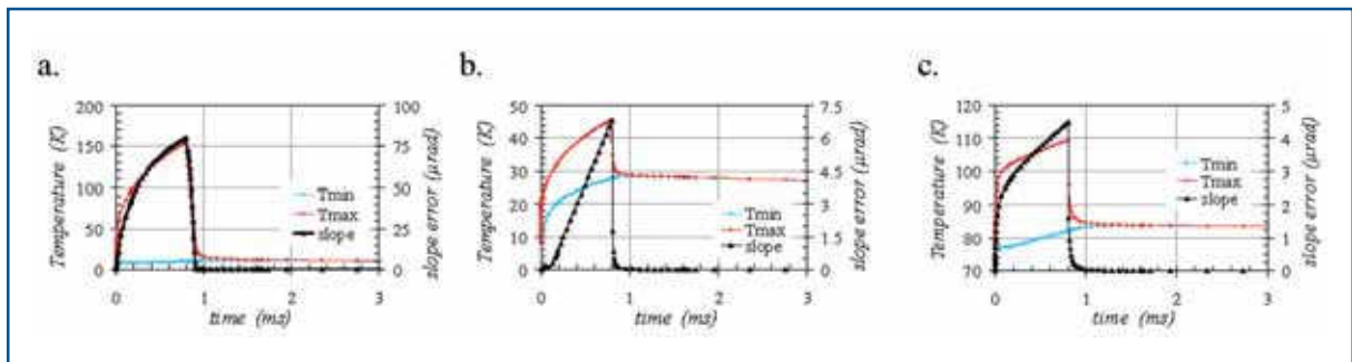
Figure 6.2.5 Temperature and slope error variation during the course of a pulse train for (a) ^{\text{nat}}\text{Si} , (b) ^{28}\text{Si} , and (c) Diamond crystals ( Q=2 \text{ J} ).
