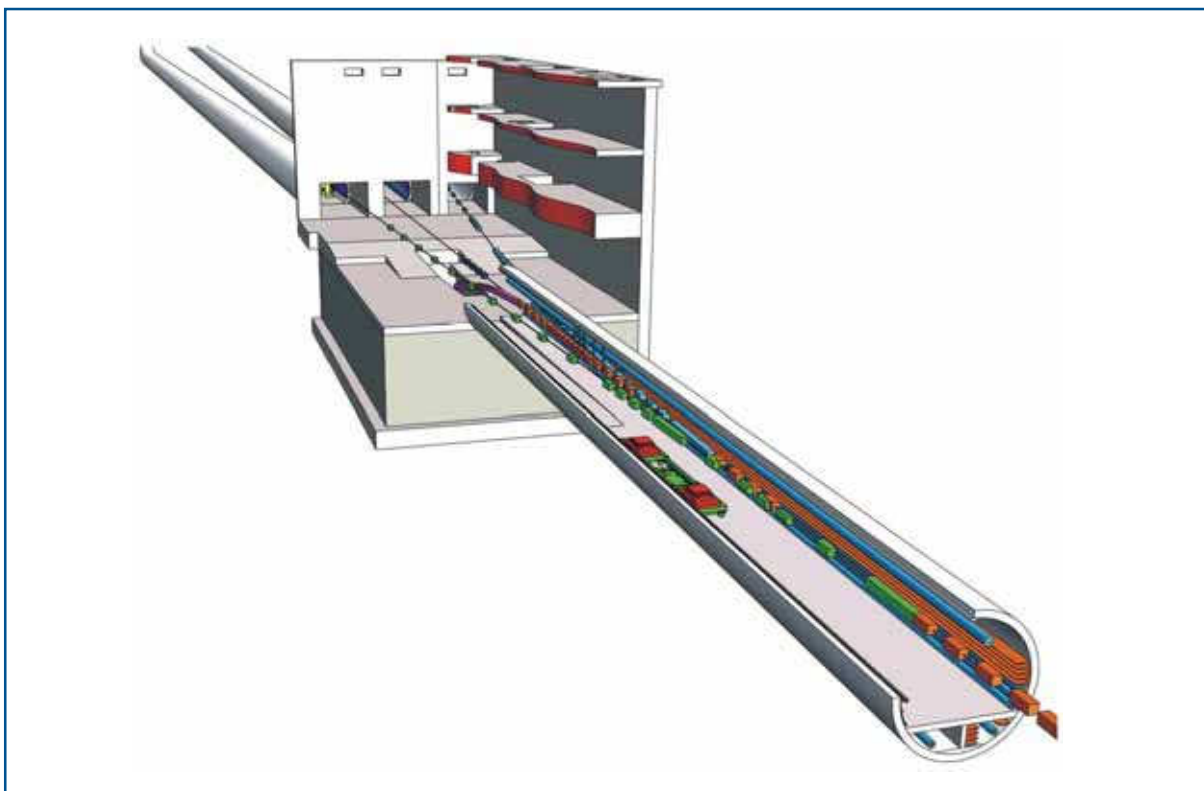
Figure 7.1.13 Beam distribution at the end of the tunnel XTL. The three-dimensional drawing shows the distribution of the electron beam to the three distribution tunnels XTD1, XTD2 and XTD20 in the horizontal plane. In addition, the vertical deflection of the beam down to the emergency and commissioning beam dump is shown.
