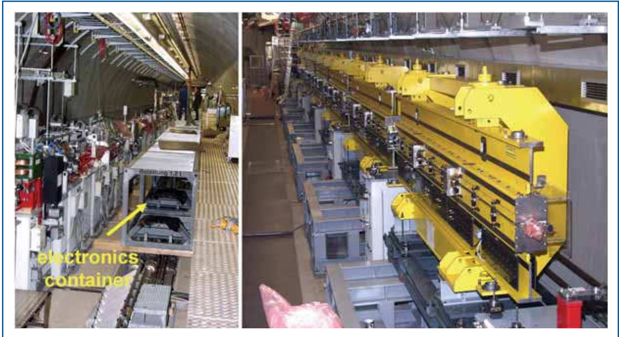
Figure 2.3.2 Left: FLASH accelerator tunnel with part of the collimator section and an electronics container visible. Right: The undulator consists of six segments, each 4.5 m long.
