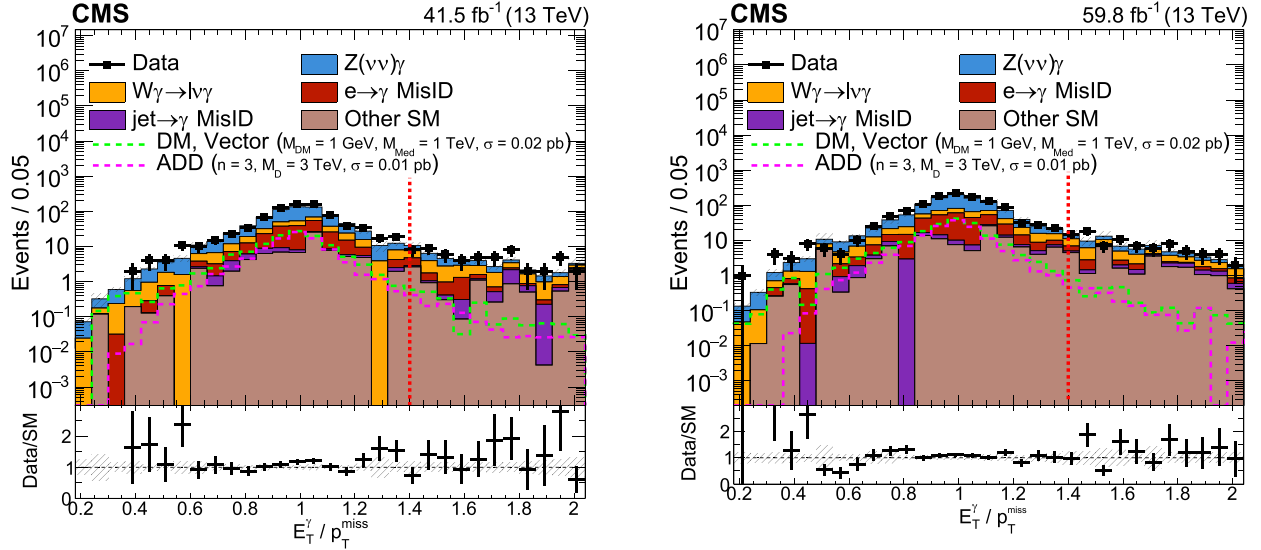
FIG. 2. Distribution of E_T^\gamma / p_T^{\text{miss}} for the 2017 (left) and 2018 (right) datasets. Templates for signal hypotheses are shown overlaid as light green and magenta dashed lines along with their cross section values. The cross hatched band represents the total systematic and statistical uncertainties. Events to the right of the red dashed vertical line are excluded.
