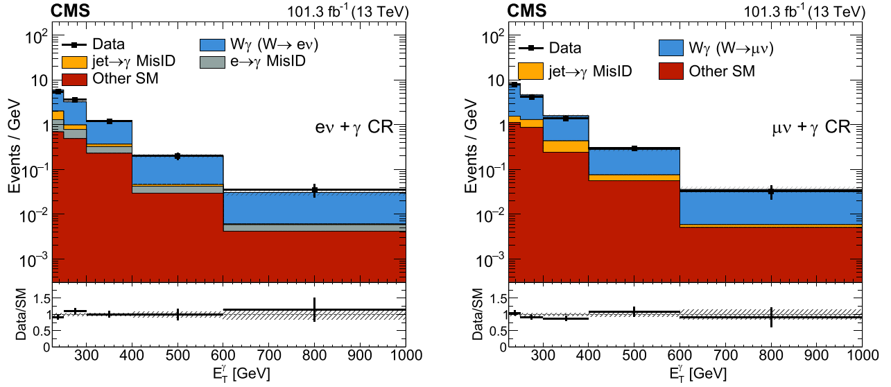
FIG. 4. Comparison of data and background postfit distributions in the e\nu + \gamma (left) and \mu\nu + \gamma (right) CRs for the combination of 2017 and 2018 datasets. The last bin of the distribution includes the overflow events. The ratios of data to the background predictions are shown in the lower panels, with the cross hatched uncertainty bands including the combination of all systematic uncertainties.
