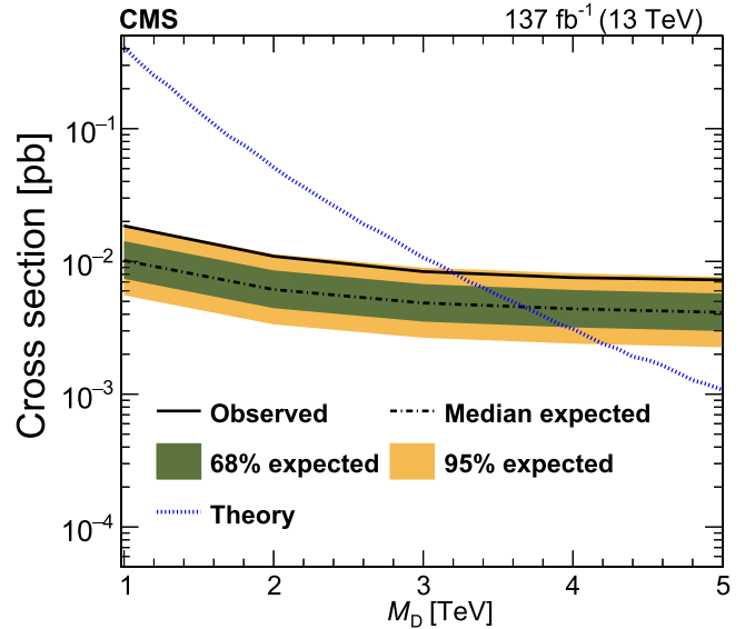
FIG. 10. The 95% CL upper limits on the ADD graviton production cross section as a function of M_D , for n = 3 extra dimensions.
