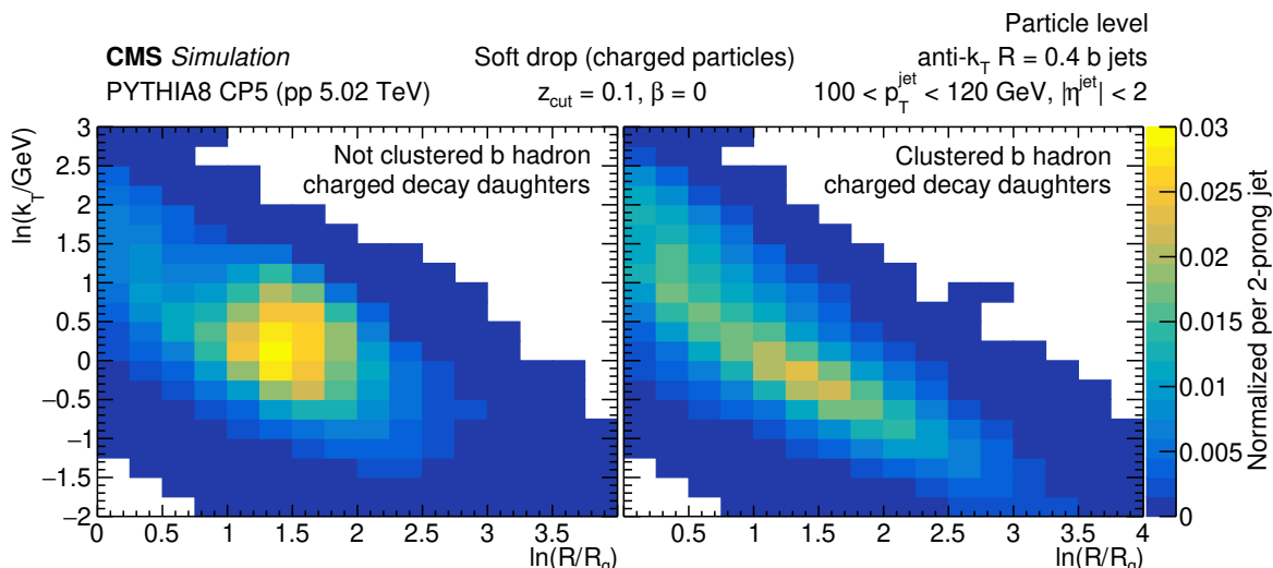
Figure 2. The Lund jet plane of the soft-drop emissions of b quark jets at the particle-level of the PYTHIA8 CP5 simulation. The vertical axis is the logarithm of the k_T /GeV of the emission, whereas the horizontal axis is the logarithm of R/R_g , such that large-angle emissions populate the left-hand side of the diagrams and small-angle emissions populate the right-hand side. On the left-hand side, the SD algorithm is applied to the charged-particle jet constituents including the b hadron decay daughters. On the right-hand side, the b hadron charged decay daughters have been clustered together prior to the SD grooming, i.e., the charged component of the b hadron remains intact. The effect of the decays can be observed in the yellow hotspot at small angles and low k_T on the left.
