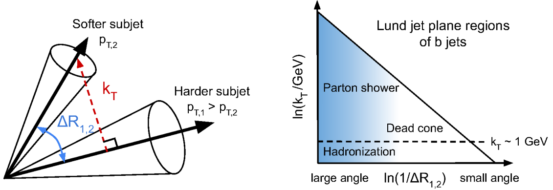
Figure 1. Left panel: A schematic diagram of two Cambridge-Aachen subjets, such as those found with the soft-drop grooming algorithm. The splitting angle \Delta R_{1,2} and the relative transverse momentum k_T between the two subjets are annotated. Right panel: The Lund jet plane regions of bottom quark jets. The vertical axis is the logarithm of the relative transverse momentum k_T/\text{GeV} of the softer subjet with respect to the harder subjet. The horizontal axis is the logarithm of the inverse of the opening angle between the softer and harder subjets, \Delta R_{1,2} . The Lund jet plane is expected to be dominated by hadronization effects for k_T below the GeV scale. Above the GeV scale, the Lund jet plane provides information on the parton showering description. Emissions are suppressed at small angles due to the dead-cone effect. The b hadron decays (not depicted) populate the same region. The blue shading, fading from left to right, represents the density of emissions in the primary Lund jet plane for b quark jets.
