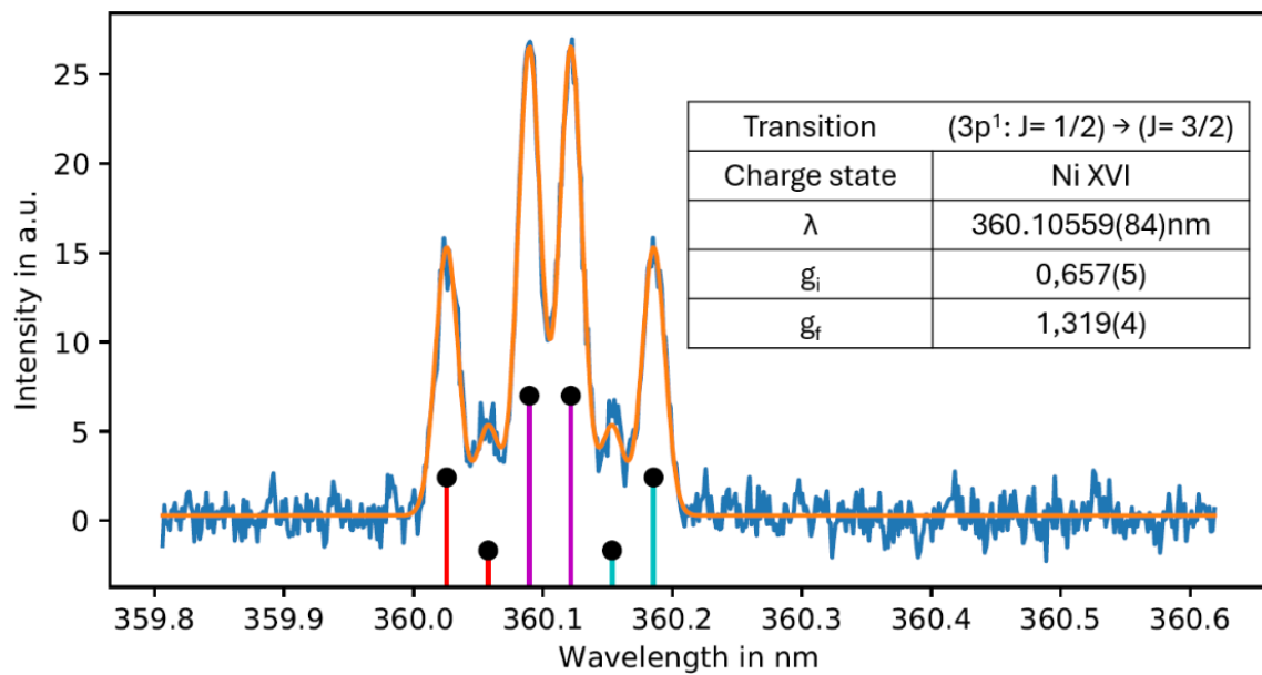
Figure 7.3.4: Zeeman fit (orange) for Ni 15+ line at 360.1 nm using 3600 grooves/mm grating and Fe-Ar calibration.
