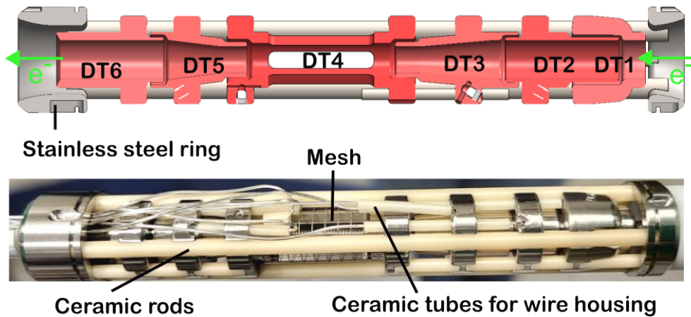
Figure 4.1.3: Cross-sectional CAD model (top) and photograph (bottom) of the mini-EBIT central region showing the six titanium drift tubes (DT1–DT6) aligned along the beam axis. The electron beam from the gun enters DT1 and propagates through to DT6 towards the collector.
