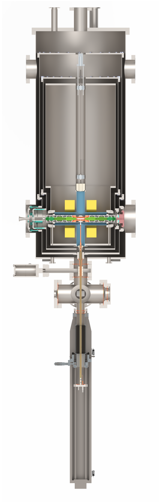
Figure B.1.3: HD-EBIT with the laser injection system
