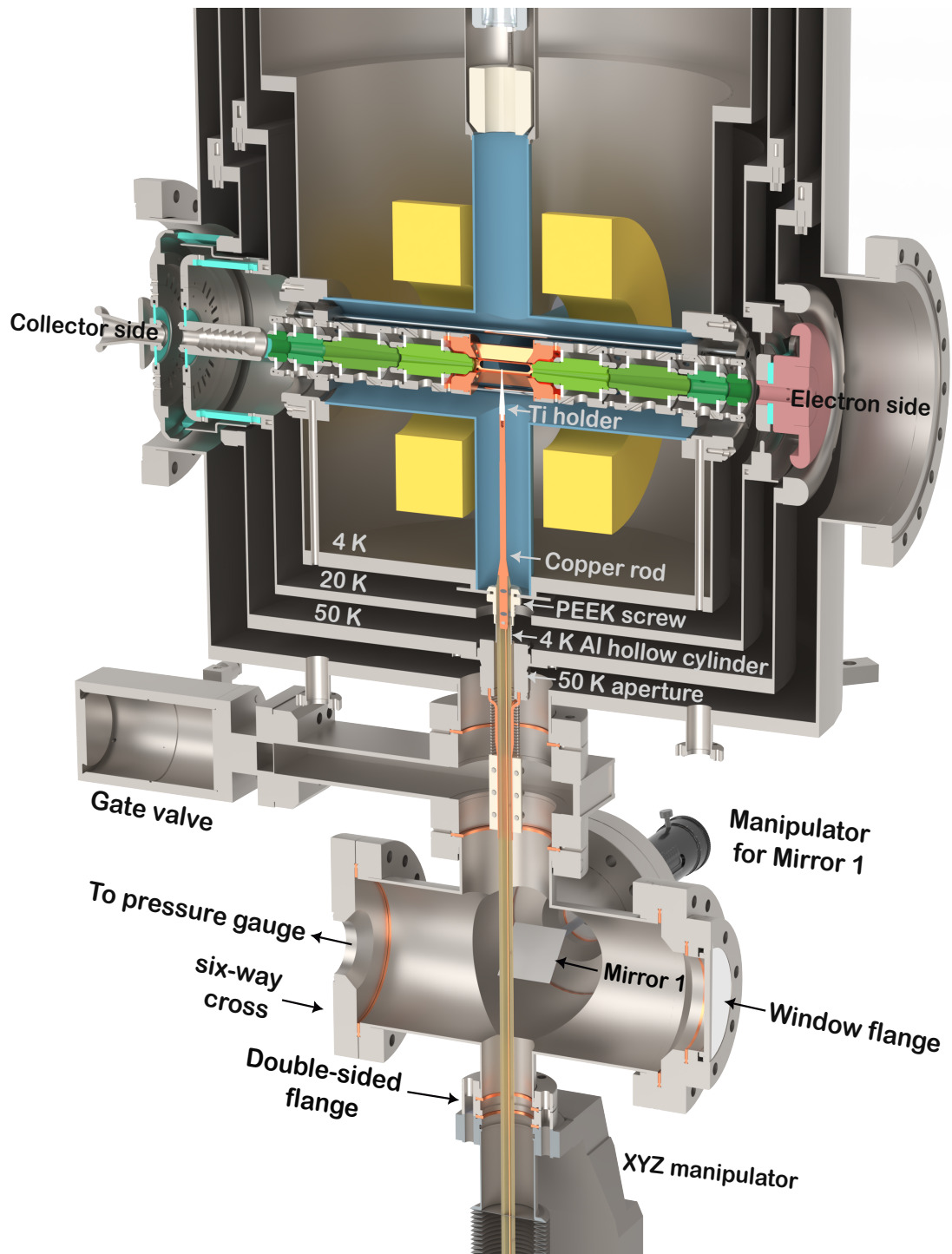
Figure 5.2.5: The manipulator-target system for the HD-EBIT, showing the locations of the parts highlighted in figures 5.2.1-5.2.4. Figure illustrates the titanium target holder at the middle of the drift tube. More pictures of HD-EBIT can be found in the Appendix B.
