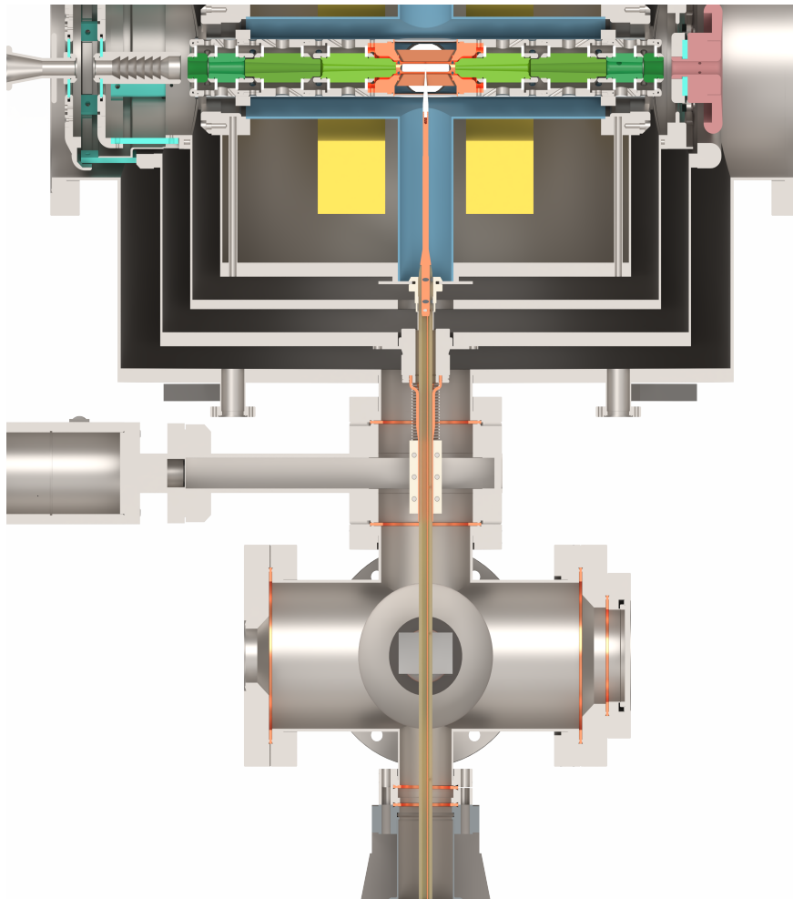
Figure B.1.1: Cross sectional view of the manipulator-target system
