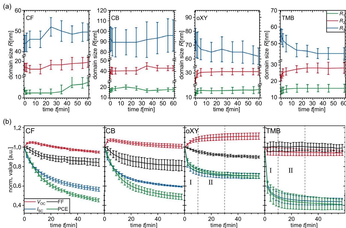
FIGURE 3 | (a) Evolution of domain sizes over time obtained from operando GISAXS fits of PTQ-2F:BTP-4F OSCs prepared from different solvents. (b) Evolution of photovoltaic parameters of PTQ-2F:BTP-4F OSCs during operando GISAXS normalized to the conditions at t = 0 . Areas labeled with roman numerals I and II indicate the timeframes of initial burn-in and subsequent stabilization, respectively.
