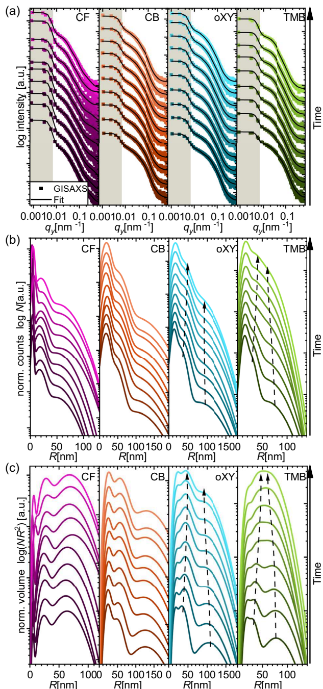
FIGURE 2 | (a) Horizontal line cuts through the Yoneda-region at q_z = 0.437 \text{ nm}^{-1} from operando GISAXS measurements performed on PTQ-2F: BTP-4F OSCs prepared from different solvents, including fits. The resolution limit defined by the beam width is highlighted in gray. (b) Domain size distribution obtained from operando GISAXS fits. (c) Volume-weighted domain size distribution obtained from operando GISAXS fits.
