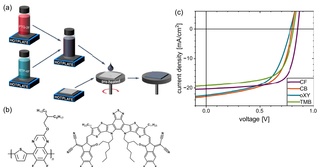
FIGURE 1 | (a) Schematic depiction of the hot spin-coating process. (b) Structural formula of the used materials PTQ-2F and BTP-4F. (c) J - V curves of champion devices of PTQ-2F:BTP-4F OSCs prepared from different solvents under an AM 1.5G, 100 mW cm -2 illumination.
