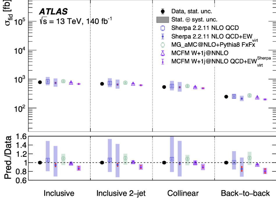
Figure 2: Measured fiducial cross-sections in each signal region are shown with total uncertainties (solid dots and error bands) and statistical uncertainties (small error bars). Various theoretical predictions (NLO, NLO+EWvirt, NNLO) are overlaid with their corresponding uncertainties: QCD scale and PDF for NLO, electroweak scheme variations for NLO+EWvirt, and MCFM-based uncertainties for NNLO. Shaded areas indicate total theoretical uncertainty, while error bars show electroweak correction uncertainties.
