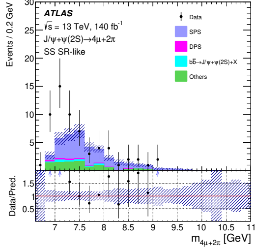
Figure 2: The J/\psi + \psi(2S) mass spectrum in the SS SR-like region of the 4\mu + 2\pi channel. The excess of data over the total background arises from the feed-up contribution.
