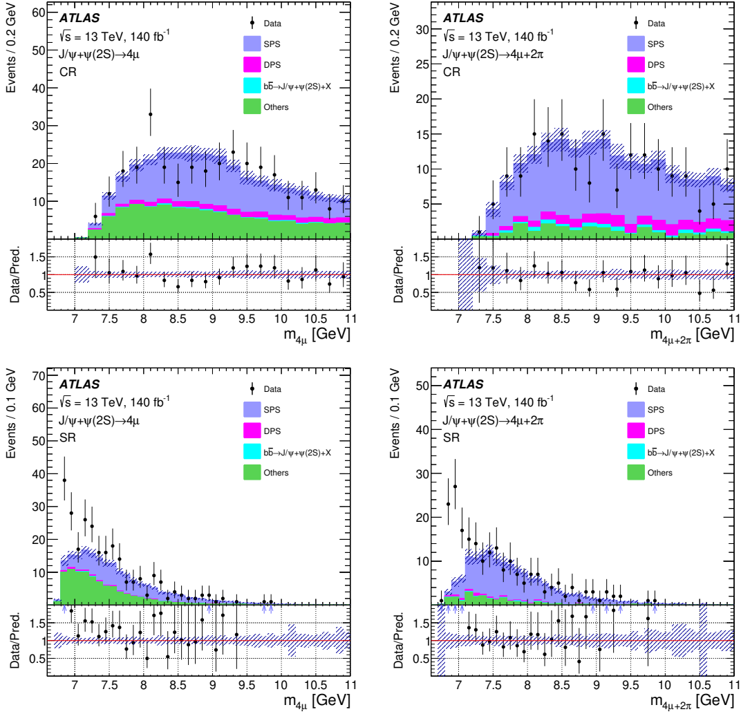
Figure 4: The J/\psi+\psi(2S) mass spectra in the CRs (top) and SRs (bottom) of the 4 \mu (left) and 4 \mu+2\pi (right) channels before the fit. The excesses observed in the signal regions arise from the signal contribution. b\bar{b} \rightarrow \text{charmonia} + X represents the Nonprompt background. The error bars (shaded areas) represent uncertainties in the data (background predictions) in each bin. Arrows in the lower panels indicate bins in which the ratio of data to the background prediction falls outside the displayed range.
