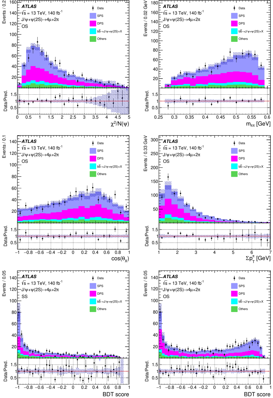
Figure 1: Distributions of the input variables (top and middle) and the BDT scores for SS (bottom left) and OS (bottom right) events in the global CR of the 4\mu + 2\pi channel. b\bar{b} \rightarrow \text{charmonia} + X represents the Nonprompt background. The error bars (shaded areas) represent uncertainties in the data (background predictions) in each bin. Arrows in the lower panels indicate bins in which the ratio of data to the background prediction falls outside the displayed range.
