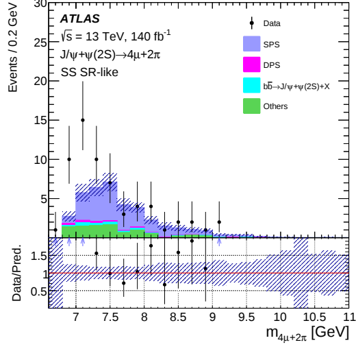
Figure 2: The J/\psi + \psi(2S) mass spectrum in the SS SR-like region of the 4\mu + 2\pi channel. The excess of data over the total background arises from the feed-up contribution.
