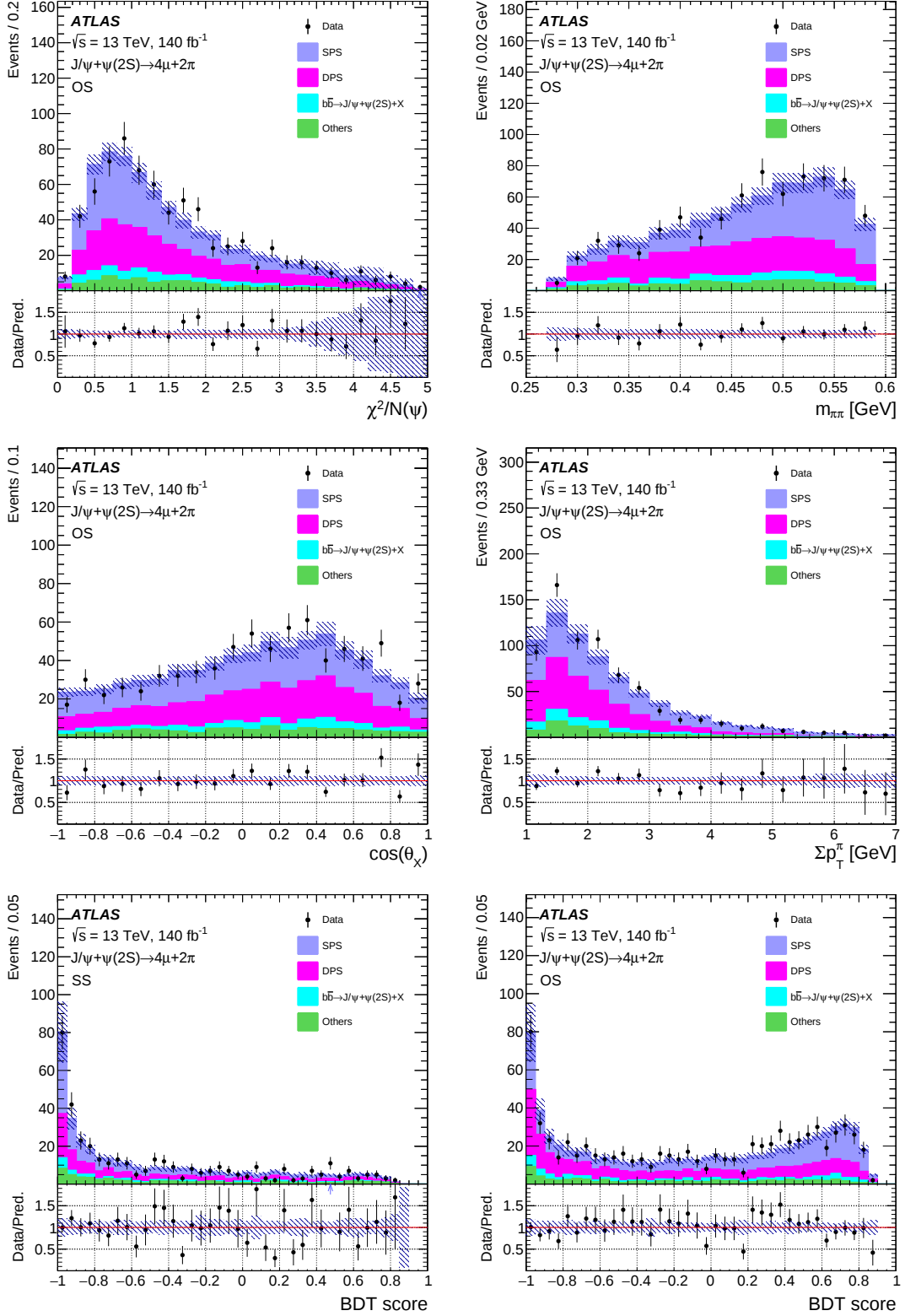
Figure 1: Distributions of the input variables (top and middle) and the BDT scores for SS (bottom left) and OS (bottom right) events in the global CR of the 4\mu + 2\pi channel. b\bar{b} \rightarrow charmonia + X represents the Nonprompt background. The error bars (shaded areas) represent uncertainties in the data (background predictions) in each bin. Arrows in the lower panels indicate bins in which the ratio of data to the background prediction falls outside the displayed range.
