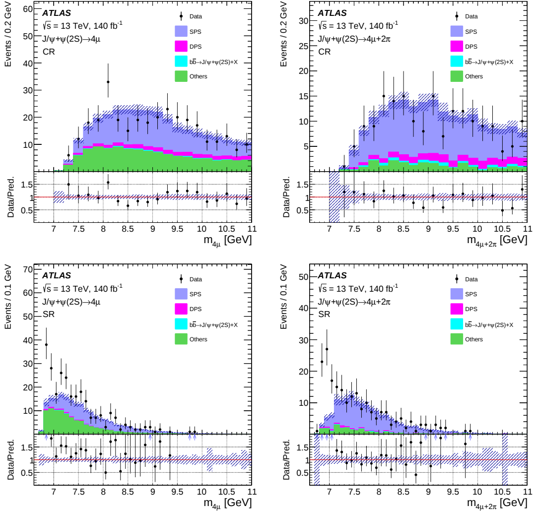
Figure 4: The J/\psi+\psi(2S) mass spectra in the CRs (top) and SRs (bottom) of the 4\mu (left) and 4\mu+2\pi (right) channels before the fit. The excesses observed in the signal regions arise from the signal contribution. b\bar{b} \rightarrow \text{charmonia} + X represents the Nonprompt background. The error bars (shaded areas) represent uncertainties in the data (background predictions) in each bin. Arrows in the lower panels indicate bins in which the ratio of data to the background prediction falls outside the displayed range.
