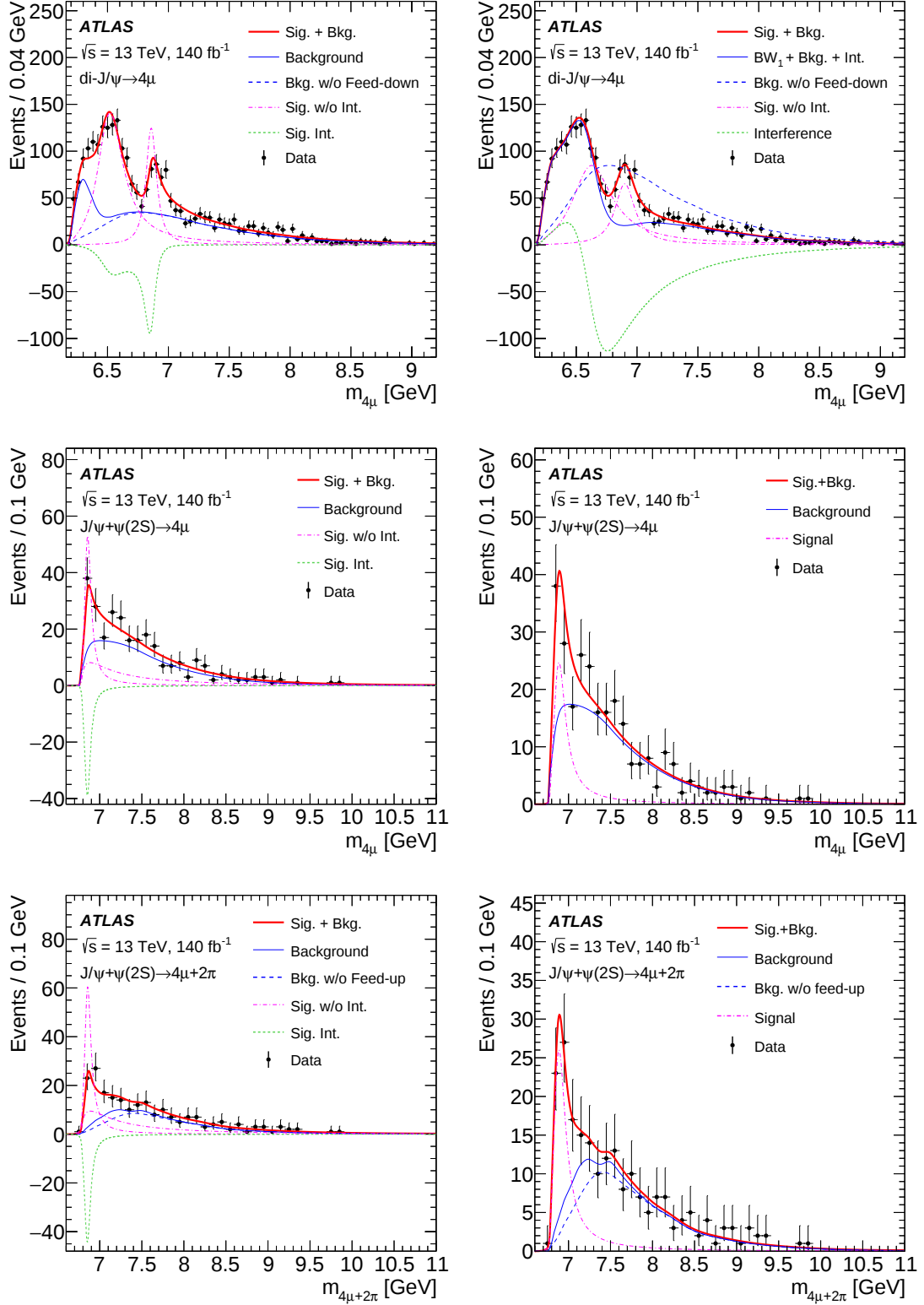
Figure 5: Fits to the di- J/\psi and J/\psi + \psi(2S) mass spectra in the SRs for model A (left) and model B (right). For each model, the di- J/\psi spectrum (top) and the J/\psi + \psi(2S) spectra in the 4\mu (middle) and 4\mu + 2\pi (bottom) channels are shown. The purple dash-dotted lines indicate the components of individual resonances, while the green short dashed ones represent the interferences. Note that no interference is present in the J/\psi + \psi(2S) channels for model B since X(6900) is standalone.
