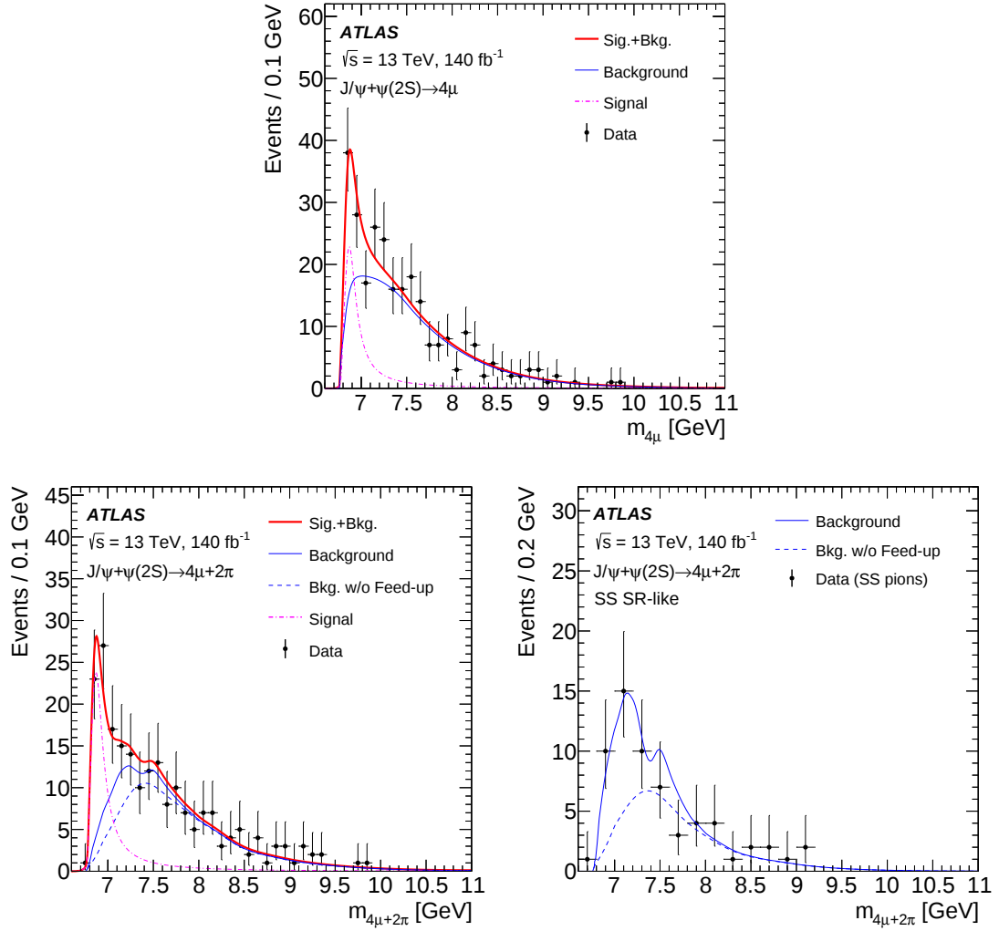
Figure 6: Fits to the J/\psi + \psi(2S) mass spectra with model C in the 4\mu SR (top), 4\mu + 2\pi SR (bottom left), and 4\mu + 2\pi SS SR-like region (bottom right). The purple dash-dotted lines represent the signal resonances.
