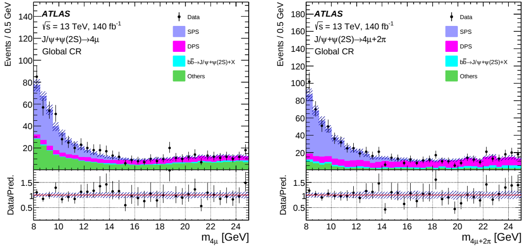
Figure 3: The J/\psi + \psi(2S) mass spectra in the global CR for the 4\mu (left) and 4\mu + 2\pi (right) channels. b\bar{b} \rightarrow \text{charmonia} + X represents the Nonprompt background. The error bars (shaded areas) represent uncertainties in the data (background predictions) in each bin. Arrows in the lower panels indicate bins in which the ratio of data to the background prediction falls outside the displayed range.
