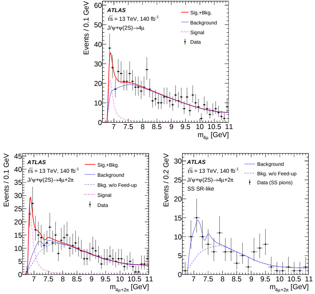
Figure 7: Fits to the J/\psi + \psi(2S) mass spectra with model C in the 4\mu (top), 4\mu + 2\pi (bottom left), and 4\mu + 2\pi SS SR-like region (bottom right), with SR and CR merged. The purple dash-dotted lines represent the signal resonances.
