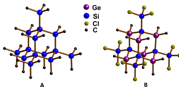
Fig. 1 Solid-state structures of the Si 10 adamantane A and the Si 4 Ge 6 adamantane B .
