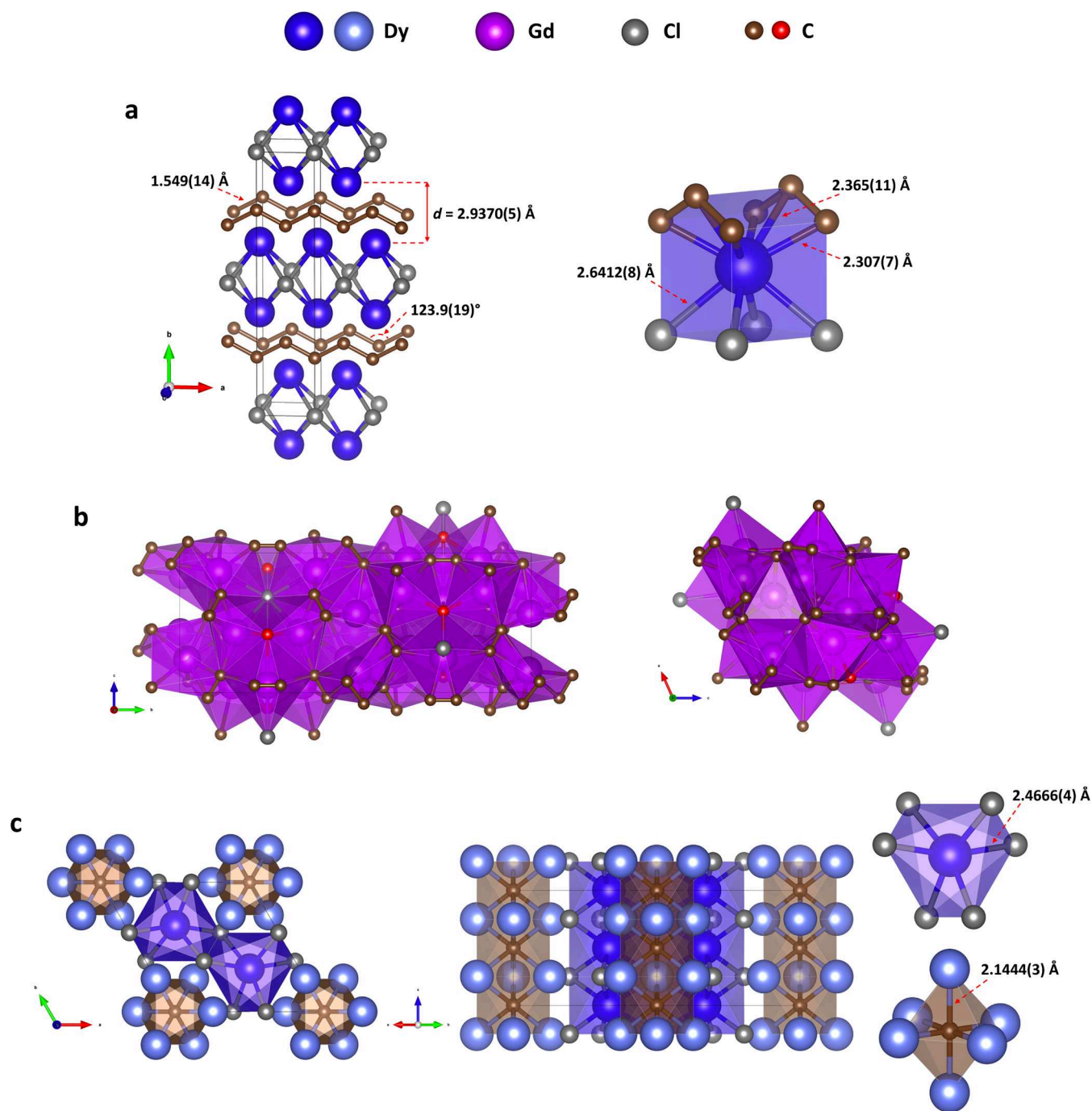
Figure 4. Crystal structures of rare-earth metal chloride carbides oC10 Dy 2 ClC 2 (and isostructural Gd 2 ClC 2 and Sm 2 ClC 2 ), mP76 Gd 19 ClC 18 (and isostructural Sm 19 ClC 18 ), and hP18 Dy 5 Cl 3 C. (a) oC10 Dy 2 ClC 2 at 76(3) GPa: stick-and-ball model (left) and coordination of Dy atoms (right). (b) mP76 Gd 19 ClC 18 at 45(2) GPa: polyhedral model as viewed along the a (left) and b (right) directions. (c) hP18 Dy 5 Cl 3 C at 122(3) GPa; from left to right: polyhedral model viewed along the c axis and [110] direction; C(Dy 2 ) 6 octahedron; DyCl 6 twisted trigonal prism. Dysprosium atoms in two crystallographically distinct positions are shown with different colors: Dy1—dark blue, Dy2—light blue; Gd—purple; Cl—gray; C catenated—brown; discrete C atoms—red.
