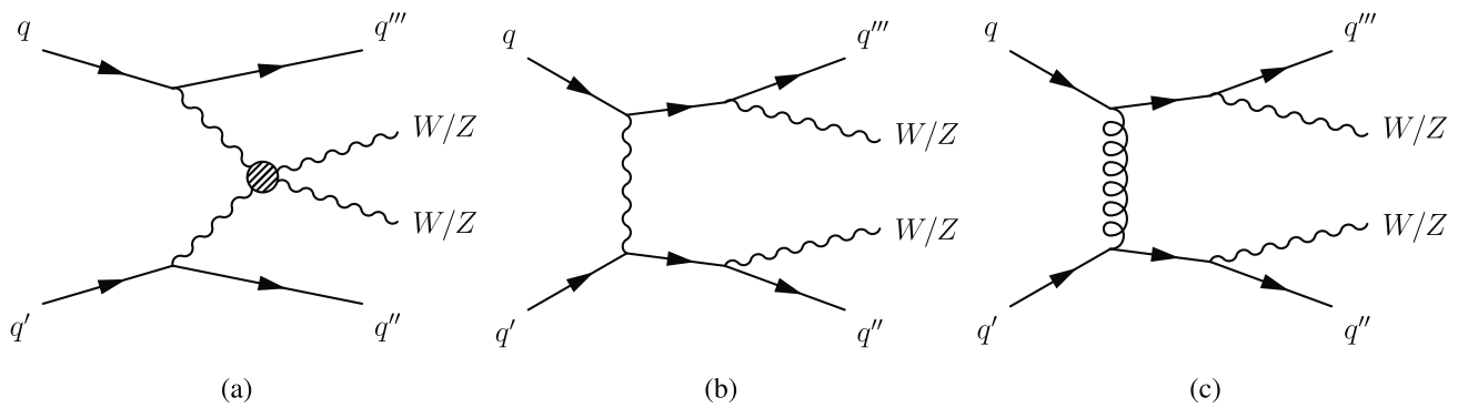
Fig. 1 Representative Feynman diagrams for a EWK VVjj production via VBS, b EWK VVjj production via a non-VBS contribution, and c QCD VVjj production
