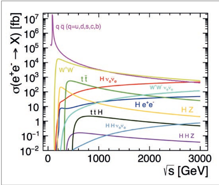
Figure 1 Production rates of various processes in electron-positron collisions as a function of the centre-of-mass energy. Between centre-of-mass energies of 200 and 1000 GeV, several processes involving Higgs bosons and top quarks become kinematically accessible. [CERN, https://clic.cern/physics-processes ]
