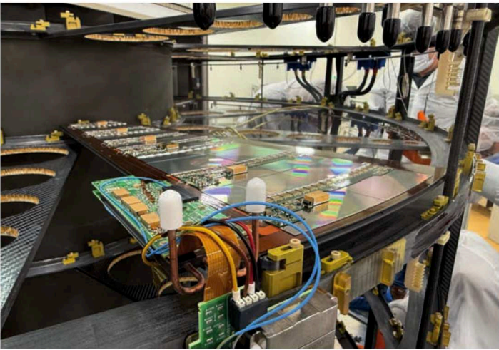
Figure 2 First full petal with silicon modules produced at both DESY sites, installed in the ATLAS endcap in the Detector Assembly Facility (DAF) at DESY
