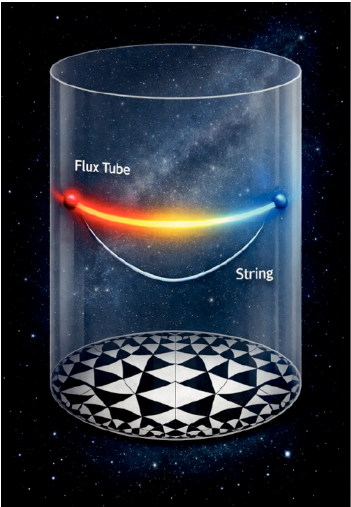
Figure 1 Holography offers an intriguing alternative to understand strongly coupled quantum systems in terms of some dual string theory. Typical features of the strongly coupled theory, such as the confining flux tube of QCD, are modelled by strings in some carefully chosen background. The latter is represented by the image at the bottom of the cylinder. For the first time, researchers at DESY were now able to engineer the string-theoretic background directly from correlations of some quantum theory that lives on the 1+1-dimensional mantle of the cylinder.
