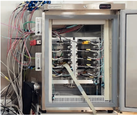
Figure 2 Burn-in test setup with modules to be tested on the support structure inside the refrigerator. The second setup is identical.
