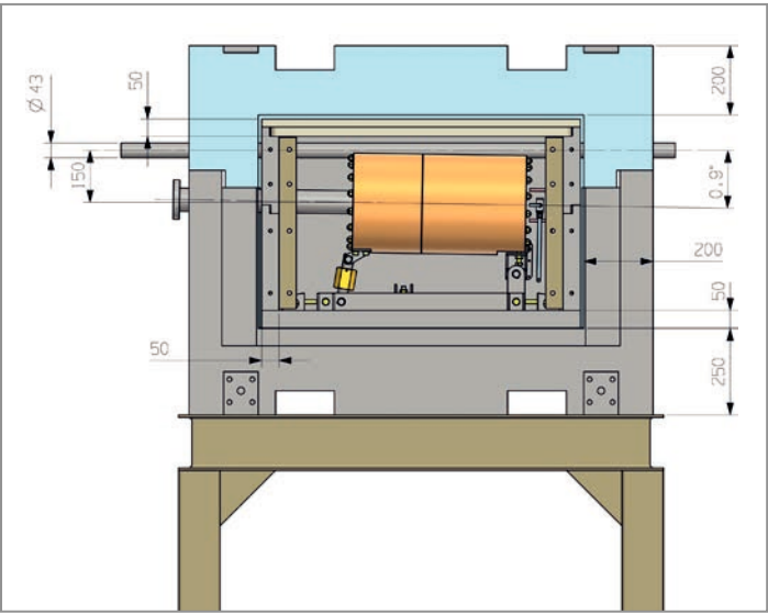
Figure 3 Design of the beam dump for the ELBEX beamline. The dump is mounted at a slight angle to point away from the rest of the tunnel. The dump will be enclosed in a concrete housing to shield the surrounding area.
