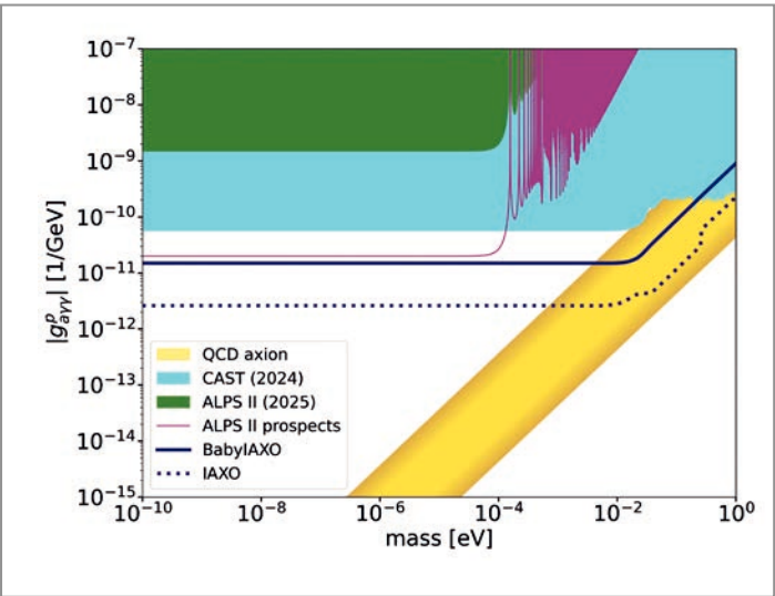
Figure 2 Sensitivity plot of BabylAXO (blue line) in the primary g_{\text{a}\gamma\gamma}-m_a parameter space, compared with the QCD axion (yellow) band and other current (filled) experimental limits. The IAXO prospects are displayed as a dotted line.
