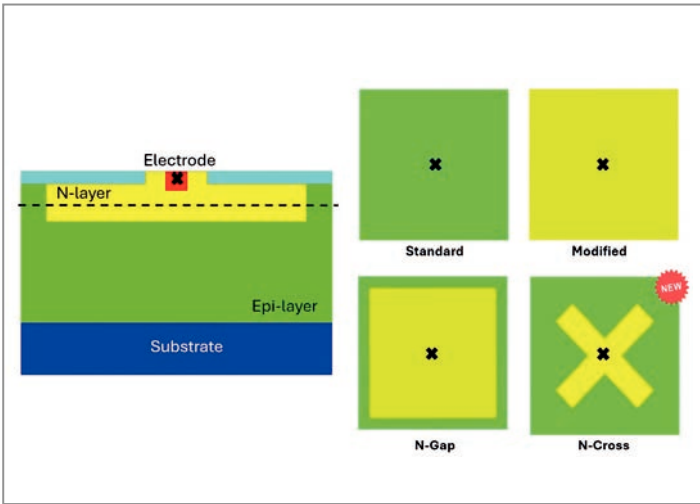
Figure 2 Left: Schematic cross section of a MAPS pixel. Right: Top view of pixel layout variations.
