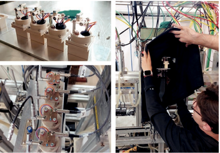
Figure 3 Top left: Containers made of PEEK, a material with excellent chemical resistance properties, in which the kidneywood solution was filled. Bottom left: Silicon photomultipliers on top of the containers, used to detect the scintillation light. Right: A light-tight cover is put over the setup at the beamline.
