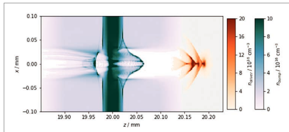
Figure 1 Snapshot of the beam and plasma densities from particle-in-cell simulation at the moment of injection
