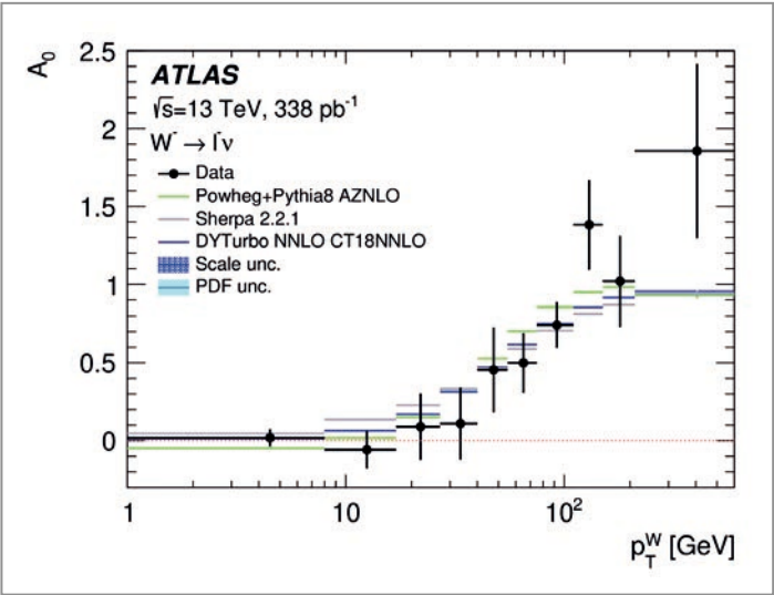
Figure 1 The W -boson angular coefficient A_0 as a function of the W -boson transverse momentum, measured for negatively charged W bosons and compared with modern theoretical predictions. Data points show total experimental uncertainties; shaded bands indicate theoretical uncertainties. From [1].
