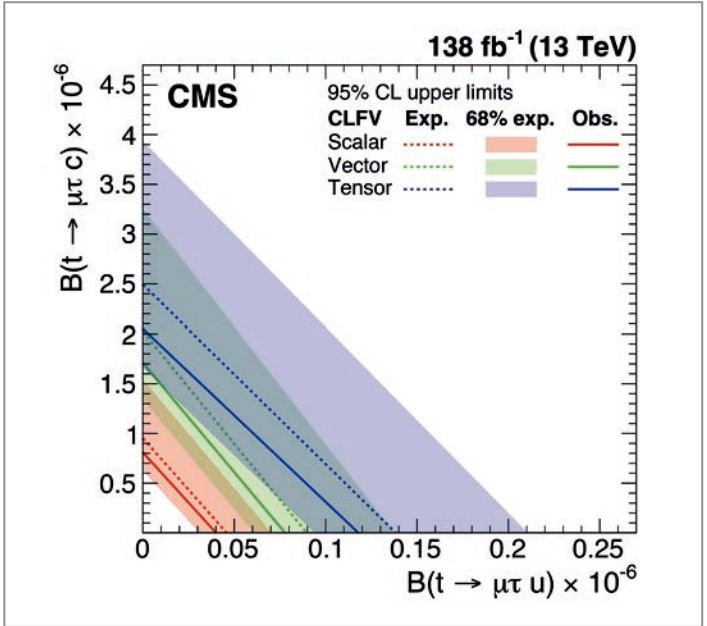
Figure 2 Observed and expected upper limit contours at 95% CL and central probability intervals containing 68% of the expected upper limits for the branching fractions
