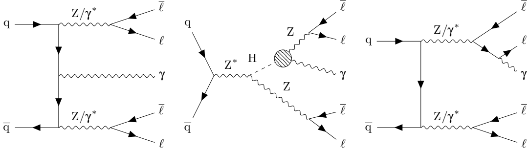
Figure 1: Representative tree-level standard model Feynman diagrams with four isolated leptons and a photon in the final state. From left to right, photon emitted from a quark line, associated ZH production, and final-state radiation.
