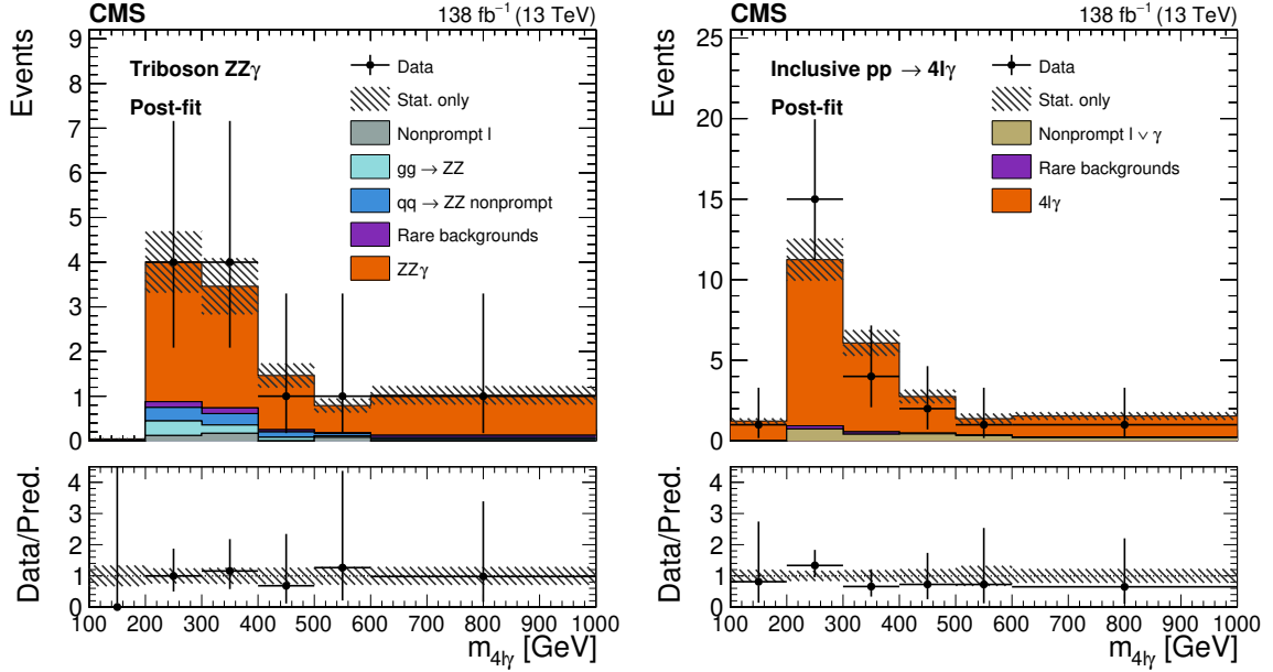
Figure 3: Post-fit mass distributions of the ZZ\gamma system in the triboson ZZ\gamma (left) and inclusive pp \rightarrow 4\ell\gamma (right) regions, obtained with the cutoff-based and multivariate photon identification, respectively. The last bin includes the events exceeding the upper bound of the x-axis. The vertical bars represent the statistical uncertainties in the data. The hatched area represents the statistical uncertainties in the simulation.
