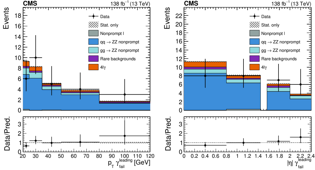
Figure 2: Transverse momentum (left) and pseudorapidity (right) of the leading photon passing the loose selection and failing the tight cutoff-based identification in the nonprompt photon application region with four tight leptons. The vertical bars represent the statistical uncertainties in the data. The hatched area represents the statistical uncertainties in the simulation.
