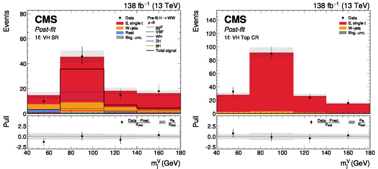
Figure 7: Post-fit m_j^V distributions in the VH channel, showing the predicted background with total uncertainty, observed data, and expected signal, split by production process. Left to right: VH SR and VH Top CR. The lower panel of each plot presents the pull distribution, as well as \sigma_{\text{fit}} normalized to the \sigma_{\text{stat}} . The predicted pre-fit signal is scaled for visibility.
