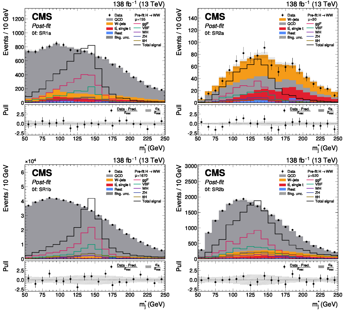
Figure 5: Post-fit m_j^* distributions in the 0\ell channel, showing the predicted background with total uncertainty, observed data, and the expected pre-fit signal scaled by the labeled strength \mu . From left to right, upper to lower, the plots correspond to SR_{1a} , SR_{2a} , SR_{1b} , and SR_{2b} . The lower panel of each plot presents the pull distribution, as well as the \sigma_{\text{fit}} normalized to the \sigma_{\text{stat}} .
