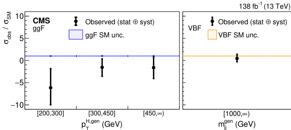
Figure 10: Unfolded measurement of the STXS cross sections in generator-level bins for three bins of Higgs boson p_T and one bin of m_{jj} in the 1\ell channel. Measured cross sections are divided by standard-model expectations. Blue and orange uncertainty bands include theoretical uncertainties affecting the signal acceptance.
