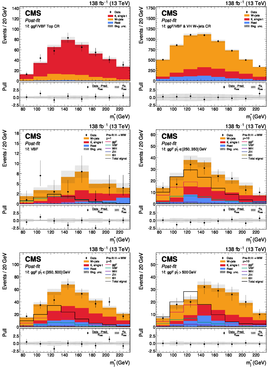
Figure 6: Post-fit m_j^* distributions in the 1\ell channel, showing the predicted background with total uncertainty, observed data, and the expected pre-fit signal scaled by the labeled strength \mu . Left to right and upper to lower: Top CR, W+jets CR, VBF SR, and the ggF SRs binned in p_T as [250, 350) , [350, 500) , and [500, +\infty) GeV, respectively. The lower panel of each plot presents the pull distribution, as well as \sigma_{\text{fit}} normalized to the \sigma_{\text{stat}} .
