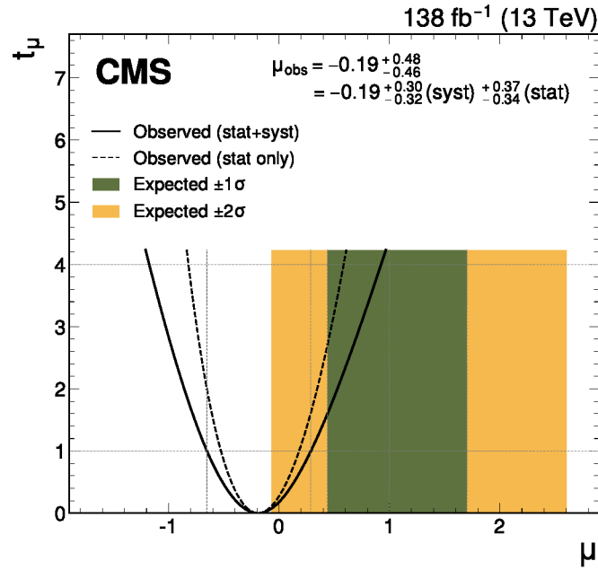
Figure 8: Observed scan of the profile likelihood test statistic t_\mu as a function of the signal strength \mu for the combination of all the channels. The solid lines correspond to profiling all statistical and systematic uncertainties, while the dashed lines correspond to profiling only the statistical uncertainties.
