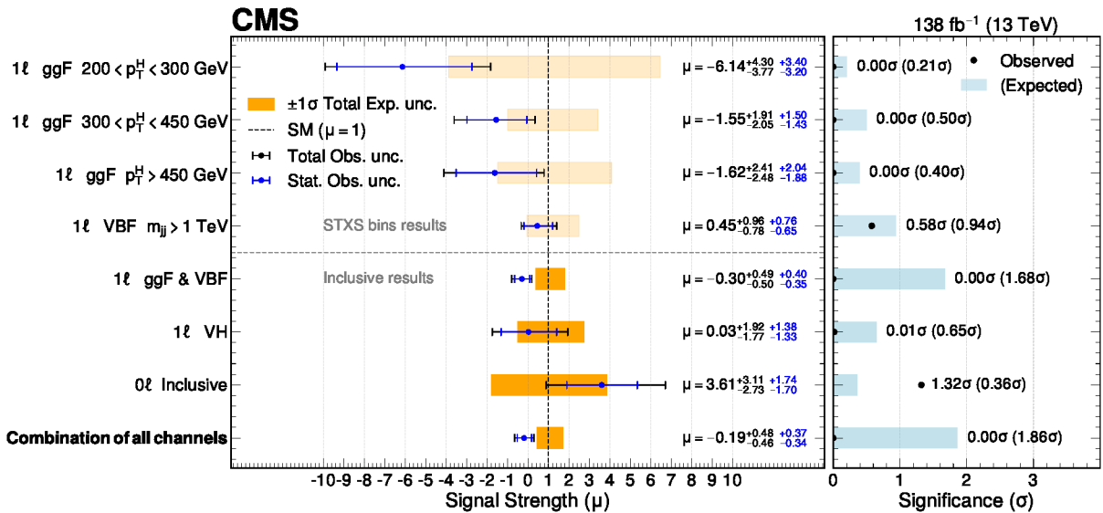
Figure 9: Observed and expected signal strength (left) and significance (right) for H \rightarrow WW in all the channels using the full data set. Combined results are presented alongside individual contributions from each channel. Total expected uncertainties are indicated by yellow bands, while signal strength significances are shown with light blue bars. Blue and black lines represent statistical and total observed uncertainties, respectively.
