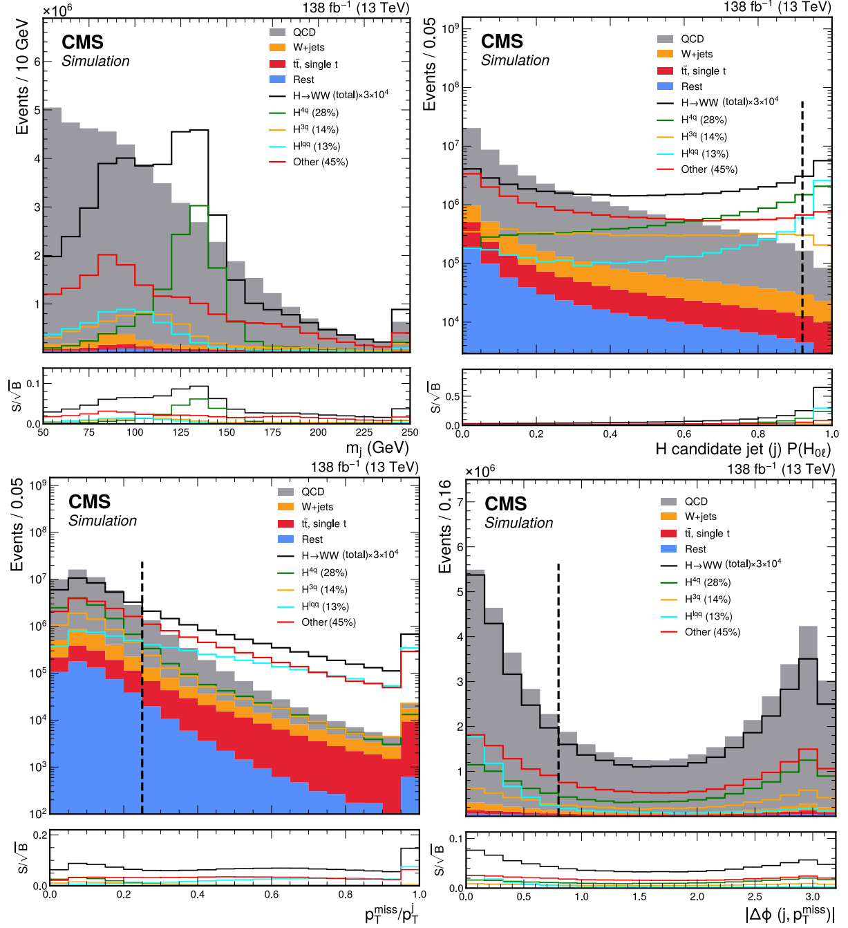
Figure 3: The distributions for the total simulated background and total signal (scaled by a factor of 3 \times 10^4 for visibility) passing event selection in the 0\ell channel. The signal is split into classes as defined in the text. The upper left and upper right panels show the soft-drop mass and PART score distributions for the H-candidate jet ( j ) P(H_{0\ell}) , respectively. The lower left and lower right panels display the p_T^{\text{miss}}/p_T^j ratio and the angle |\Delta\phi(j, \vec{p}_T^{\text{miss}})| , respectively. Vertical lines indicate the selection conditions imposed to define the SRs.
