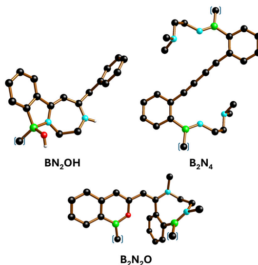
Fig. 6 Solid-state structures of \text{BN}_2\text{OH} (left), \text{B}_2\text{N}_4 (right), and \text{B}_2\text{N}_2\text{O} (bottom). H: white, B: green, C: black, N: cyan, O: red. For clarity, only the ipso -C atoms of the Mes substituents are shown; C–H atoms are omitted.
