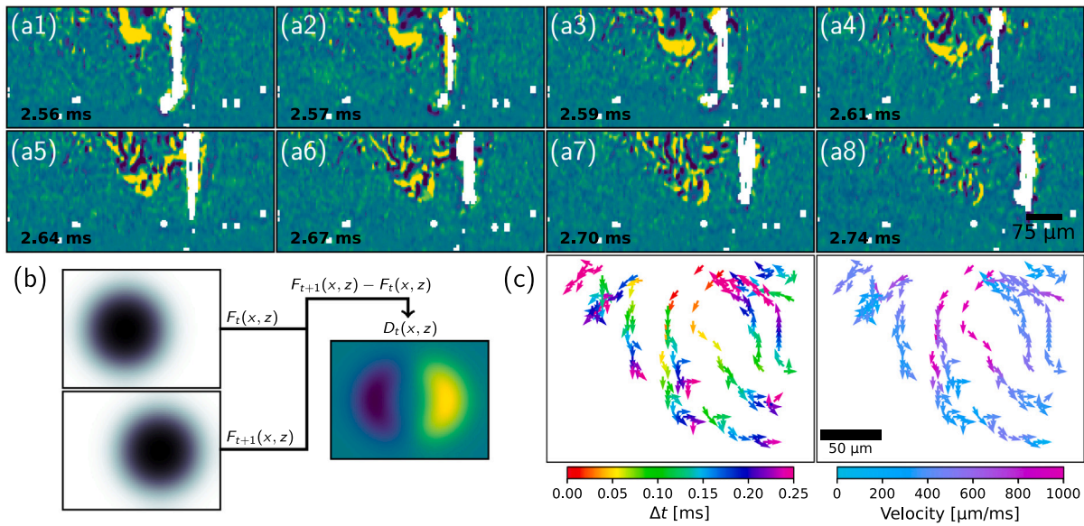
Fig. 3. Characterization of the dynamics and fragmentation of a Cu event during AM: (a) Snapshots of projected ( x - z ) image differencing during the printing of L4, the image differencing method is schematically presented in (b). (c) Projected relative times and velocities of Cu mixing discrete occurrence for L4 in the melt pool onto the x - z plane.
