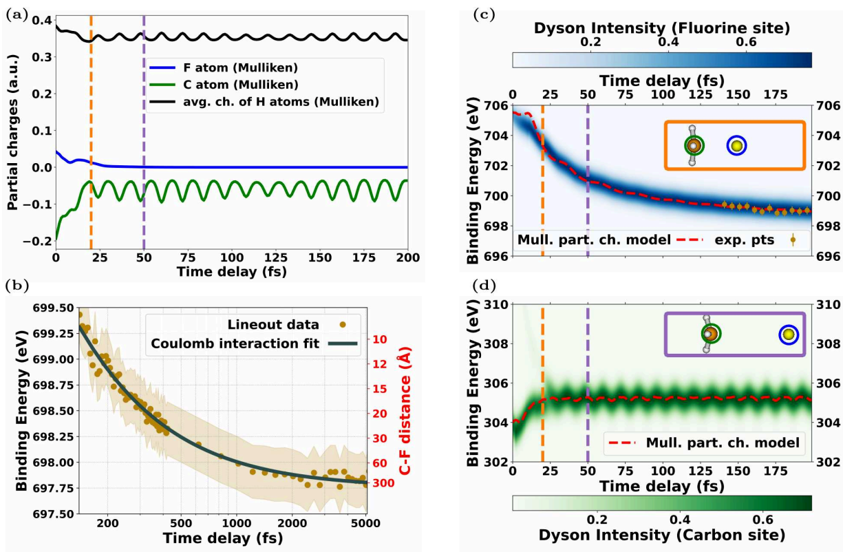
FIG. 2. Dynamical chemical shift during C-F bond elongation. a) Calculated partial charges (Mulliken charges) at the location of the F, C and H atoms, for a single C-F dissociation trajectory. b) Measured time-dependent chemical shift of atomic F (golden dots, shaded region corresponds to the standard deviation) and fitted function based on the Coulomb interaction model (grey line), described in the main text. (c) and (d) Calculated binding energy based on PC model applied with the calculated Mulliken charge (red line) and Dyson intensity (blue colorscale for F and green for C), calculated through the ab-initio model including core-hole states. A shift of 0.5 eV is applied to the calculations in panel (c) as explained in section S3-C of the SM. Dotted lines in (a), (c), and (d) mark the delays for the representative snapshots shown in the inset of (c) and (d). A weak satellite feature between 306 and 310 eV is observed in (d) for delays below 25 fs.
