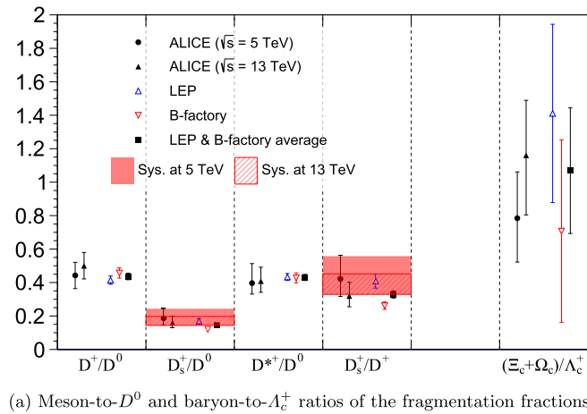
(a) Meson-to- D^0 and baryon-to- \Lambda_c^+ ratios of the fragmentation fractions.
