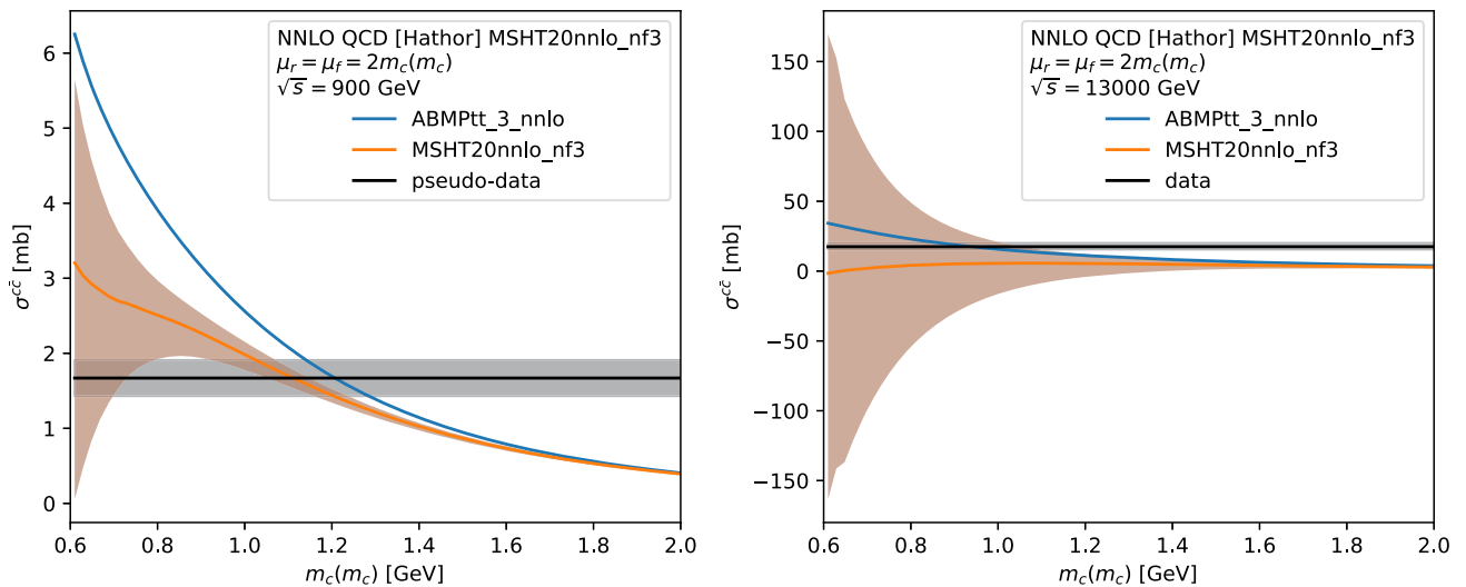
Fig. 16 The total charm cross sections at NNLO QCD at \sqrt{s} = 0.9 (left) and 13 TeV (right) computed using the ABMPtt_3_nnlo and MSHT20nnlo_nf3 PDF sets. The corresponding data values with their uncertainties are shown as horizontal bands
