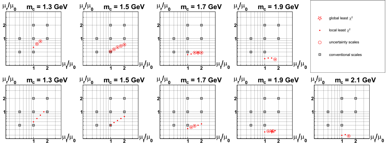
Fig. 7 The scales giving the best description of the D^0 measurements at \sqrt{s} = 5 TeV (the first row) and 13 TeV (the second row), respectively. The local least \chi^2 are shown by the circle point symbols while the global least \chi^2 for each \sqrt{s} is marked by the additional star symbol.
