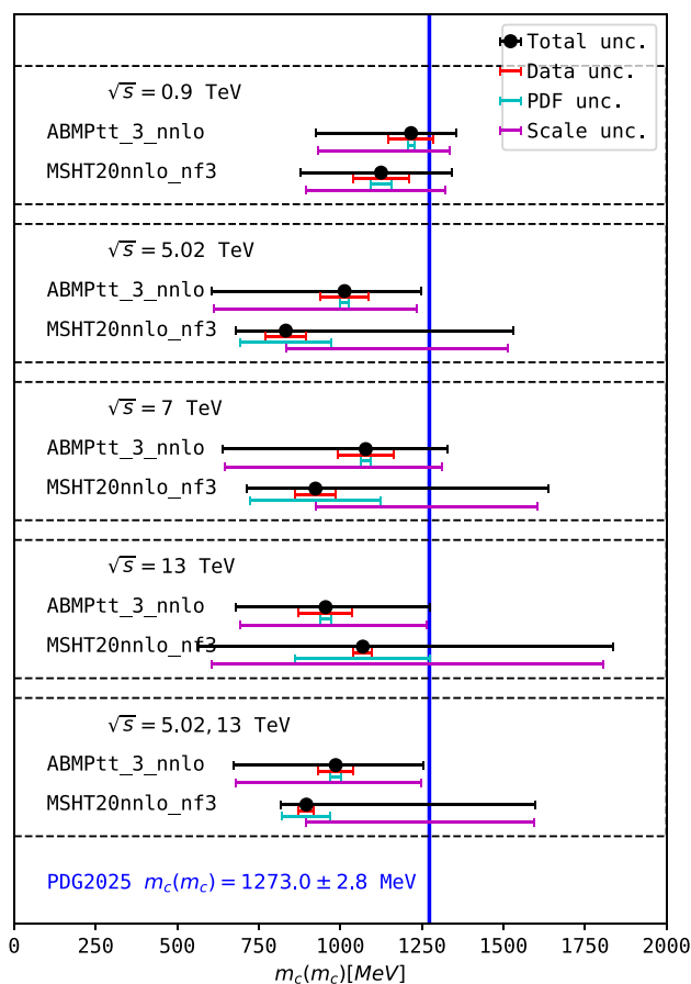
Fig. 18 The m_c(m_c) values extracted using various charm data points, together with their experimental, PDF and scale variation uncertainties. The world average value from Ref. [54] is shown as well
