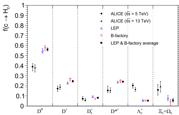
Fig. 1 Fragmentation fractions measured from the ALICE [20,31] and e^+e^- experiments [39]. The label \Xi_c + \Omega_c indicates \Xi_c^0 + \Xi_c^+ + \Omega_c^0
