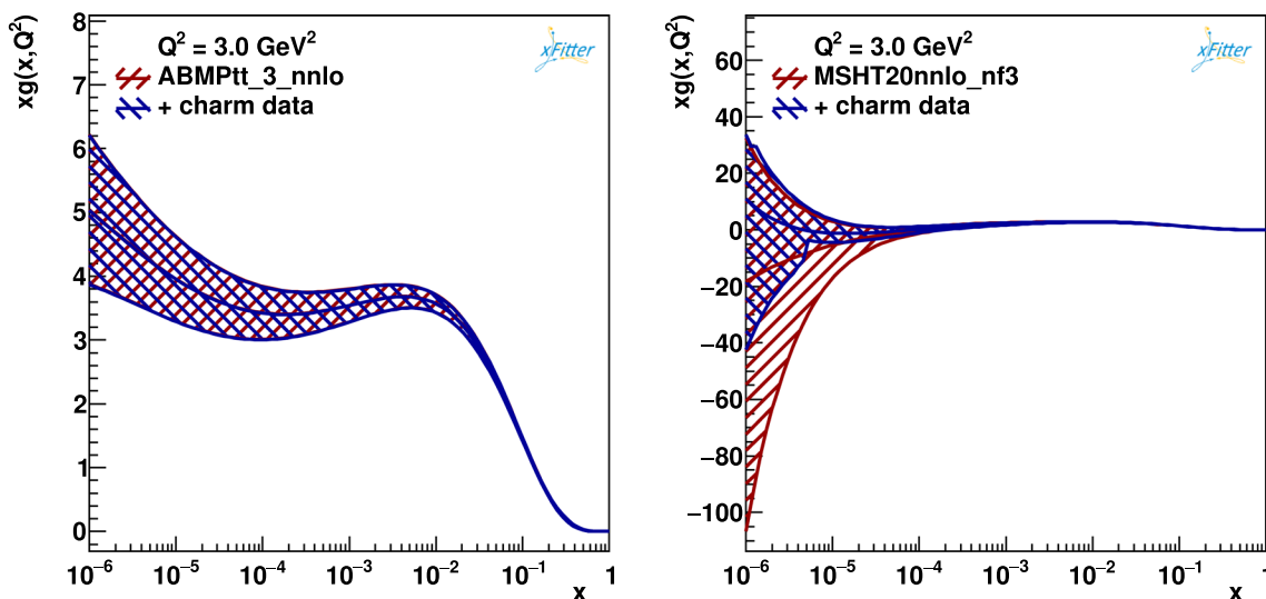
Fig. 17 The gluon distribution of the original and profiled ABMPtt_3_nnlo (left) and MSHT20nnlo_nf3 (right) PDF sets at the scale \mu_f^2 = 3 \text{ GeV}^2
