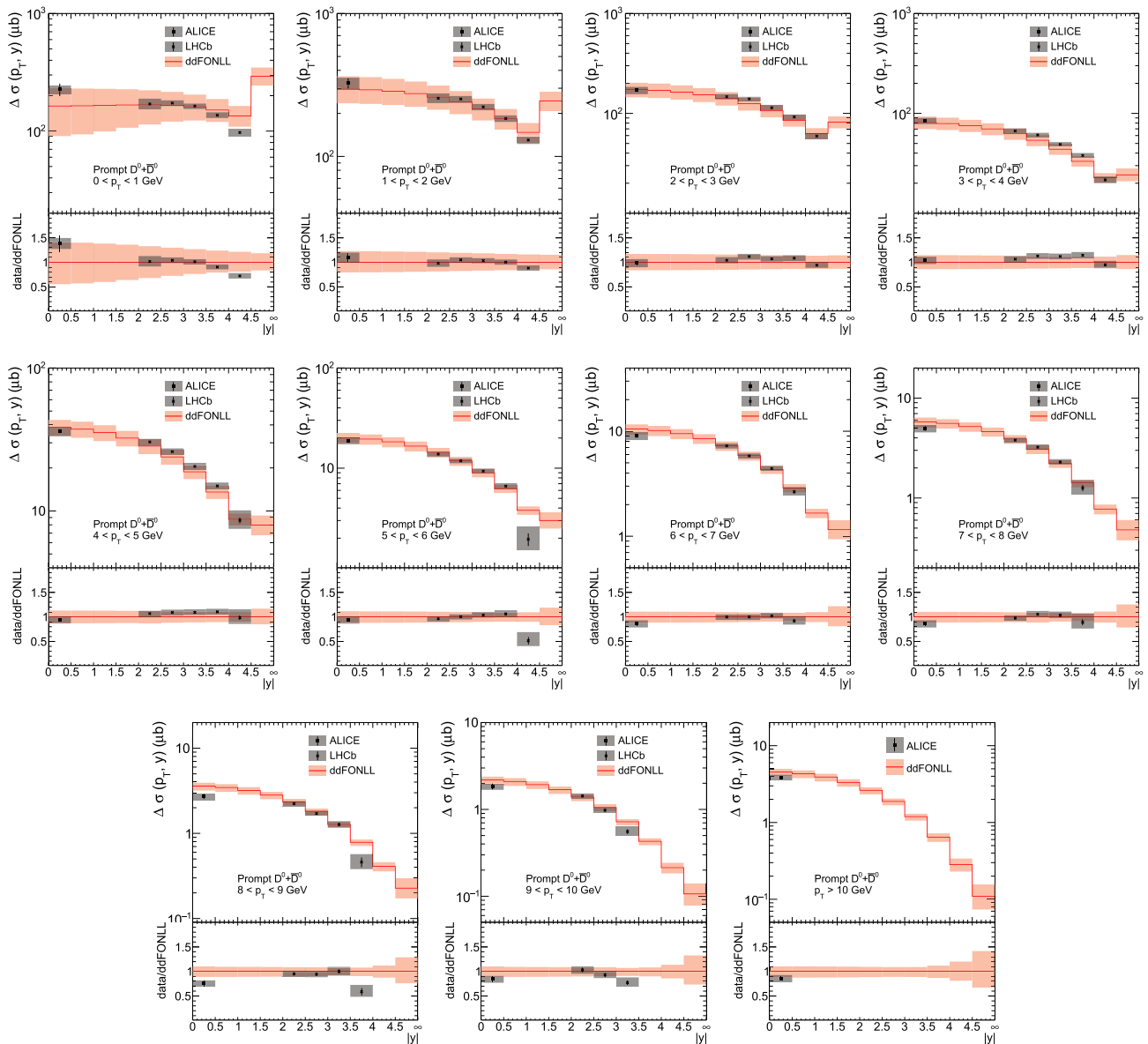
Fig. 8 D^0 + \bar{D}^0 cross sections at \sqrt{s} = 5 TeV as a function of |y| . The red bands of ddFONLL show the total uncertainty (CTEQ6.6 PDF \oplus \tilde{f} \oplus \chi^2 )
