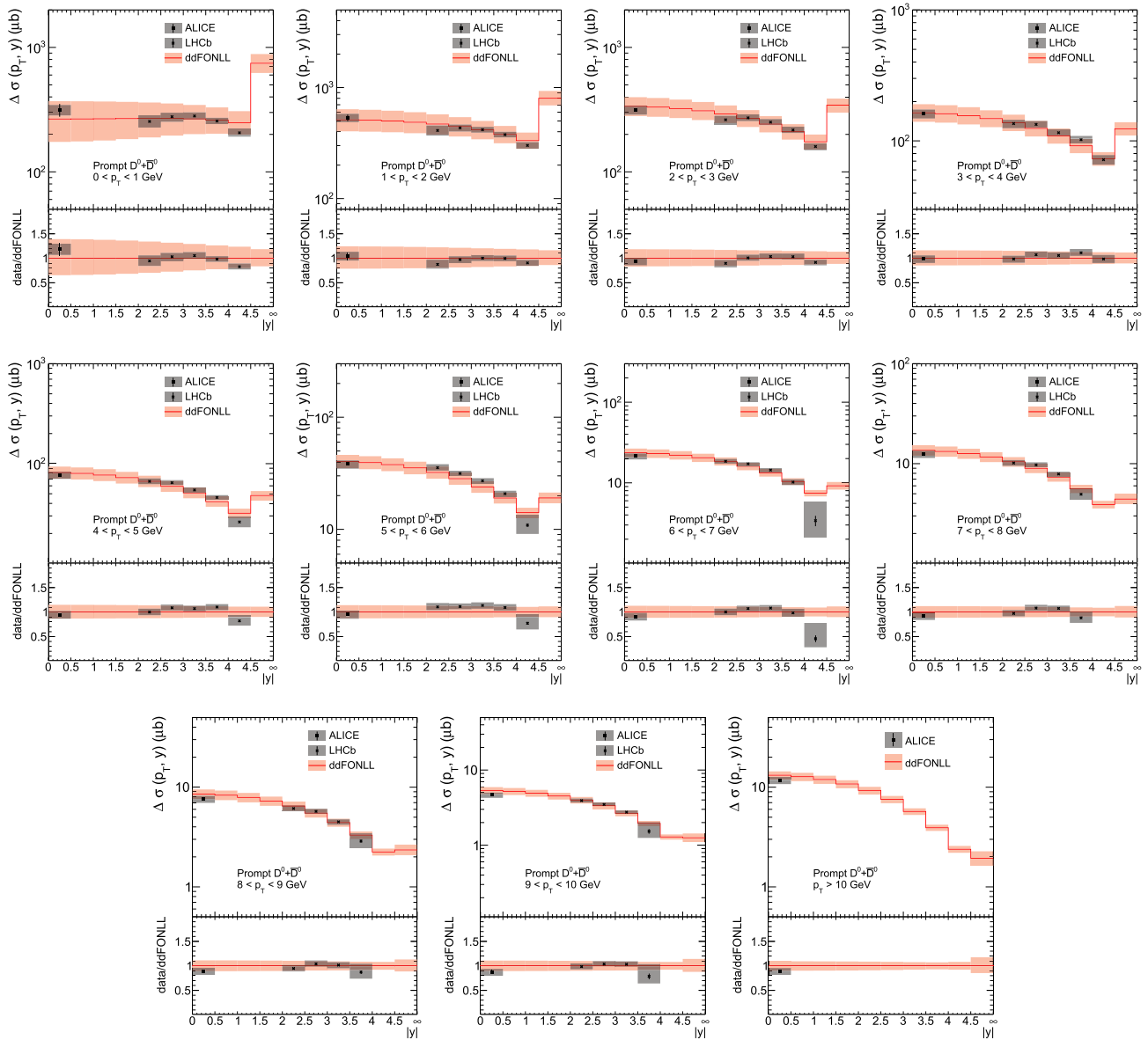
Fig. 9 D^0 + \bar{D}^0 cross sections at \sqrt{s} = 13 TeV as a function of |y| . The red bands of ddFONLL show the total uncertainty (CTEQ6.6 PDF \oplus \tilde{f} \oplus \chi^2 )
