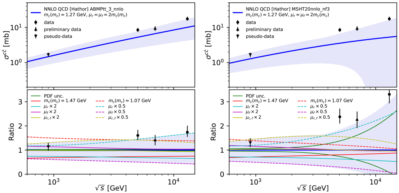
Fig. 15 The total charm cross sections at NNLO QCD computed using ABMPtt_3_nnlo (left) and MSHT20nnlo_nf3 (right) as a function \sqrt{s} . The lower panel displays the theoretical predictions and the data or pseudodata normalized to the central theoretical prediction
