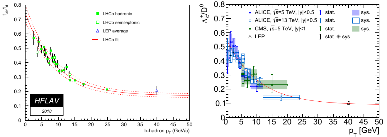
Fig. 2 Measurements of the ratio of \Lambda_b^0 to B^0 (left figure) and the ratio of \Lambda_c^+ to D^0 (right figure). The left figure is from [42], where the exponential fit to LHCb data gives consistent results to LEP at high p_T . In the right figure, the ALICE and CMS points are collected from [15, 20] and [27], respectively, and the LEP point is derived based on the numbers given in [39]. Apart from the LEP value, these points are
