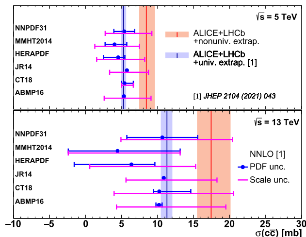
Fig. 14 The total charm cross sections at \sqrt{s} = 5 (top) and 13 TeV (bottom), with figures adapted from [30]. The vertical red bands are the total charm cross sections provided in this work
