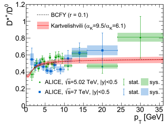
Fig. 13 D^*/D^0 comparison between ALICE measurements [12] at \sqrt{s} = 5 TeV (the green triangle points) and 7 TeV (the blue square points) and FONLL predictions (the black dashed and red solid line)
