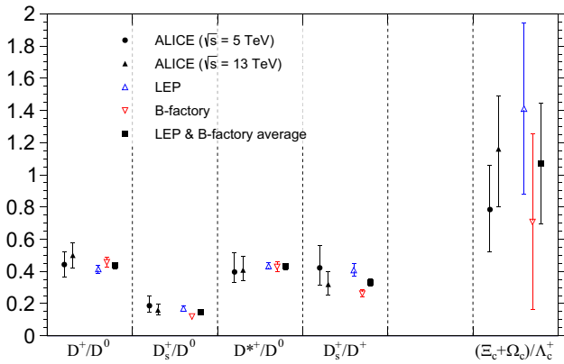
Fig. 3 Comparison of meson-to- D^0 , D_s^+ -to- D^+ and baryon-to- \Lambda_c^+ ratios of fragmentation fractions between e^+e^- and pp collisions. The label \Xi_c + \Omega_c indicates \Xi_c^0 + \Xi_c^+ + \Omega_c^0 . The uncertainties were derived under the simplifying assumption that the measurement uncertainties are fully uncorrelated
