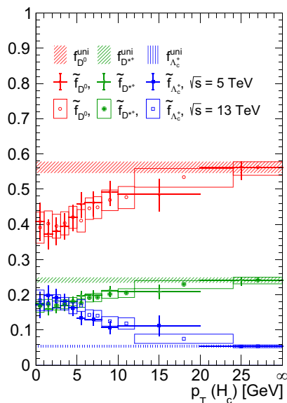
Fig. 5 \tilde{f}_{D^0}(p_T) , \tilde{f}_{\Lambda_c^+}(p_T) and \tilde{f}_{D^{*+}}(p_T) . The red, blue and green band are the D^0 , \Lambda_c^+ and D^{*+} fragmentation fractions with the uncertainties, respectively, measured from e^+e^- collisions
