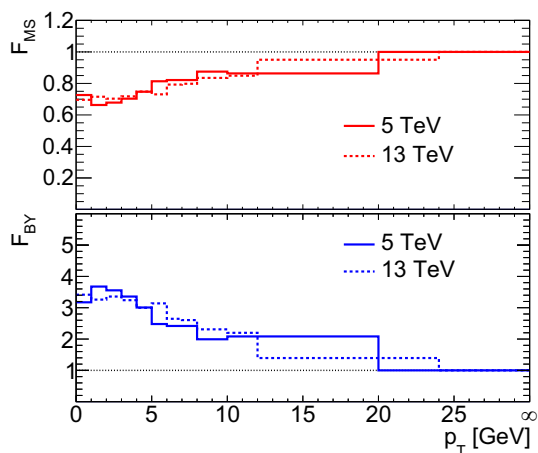
Fig. 4 F_{MS}(p_T) (red histogram) and F_{BY}(p_T) (blue histogram) at \sqrt{s} = 5 (solid line) and 13 (dashed line) TeV. These are asymptotically close to 1 at high p_T by definition, Eq. (9)
