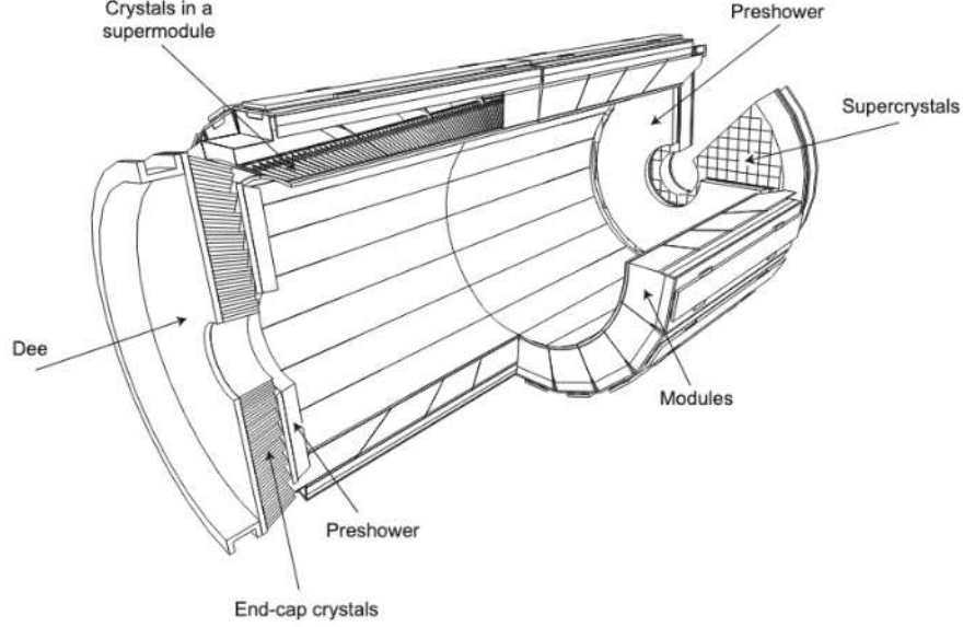
Figure 3.7: The CMS ECAL layout [36]
