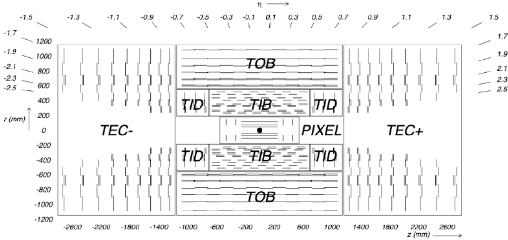
Figure 3.6: The CMS tracker sketch in r-z view [31]
