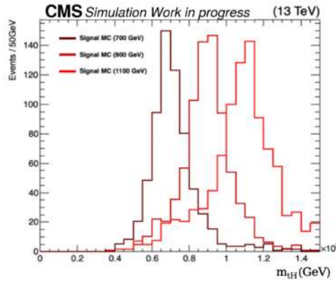
Figure 4.12: Reconstructed T mass from signal MC
