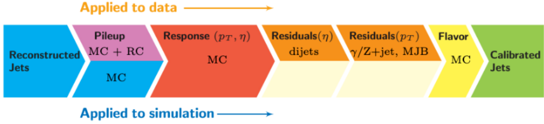
Figure 3.11: Jet energy scale corrections at CMS [56]
