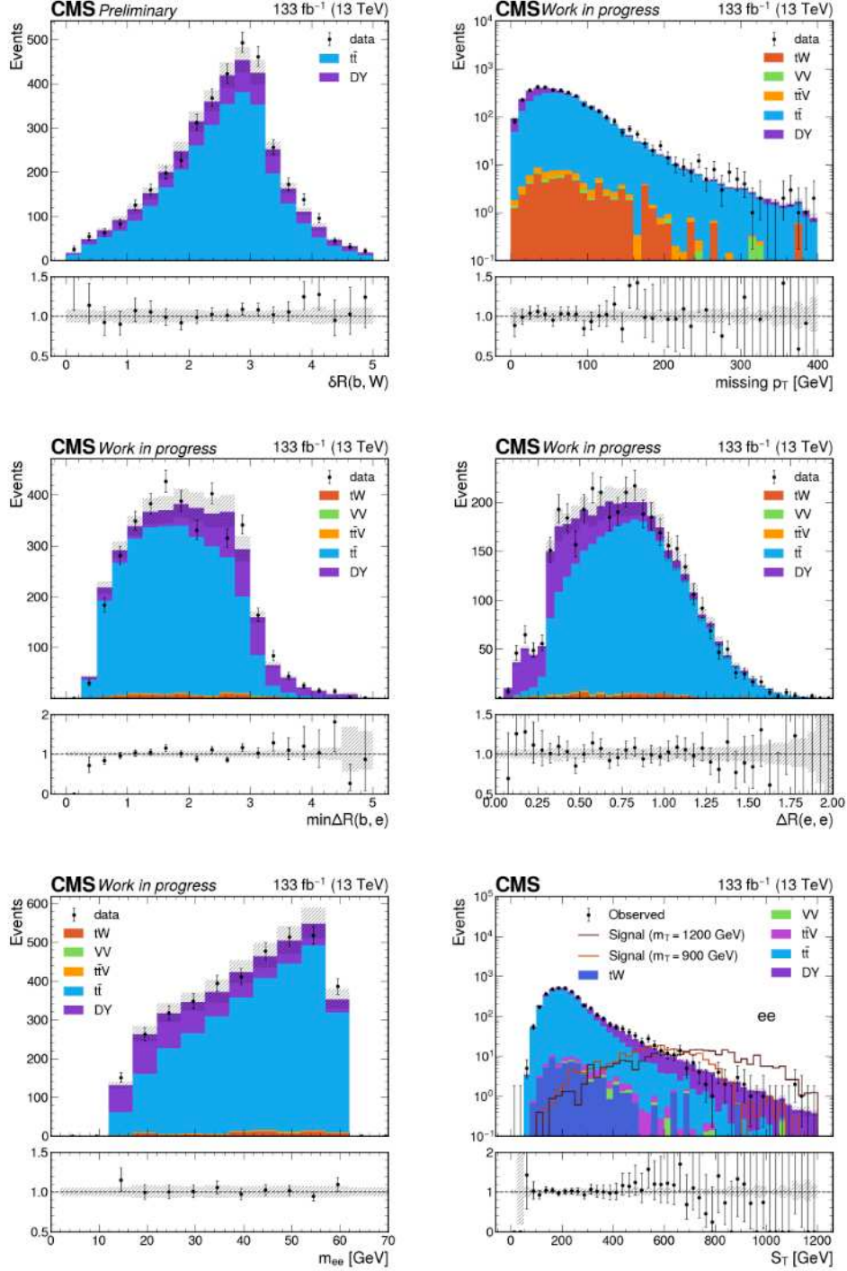
Figure 4.24: Data-MC comparison for the ee channel in full Run 2.
