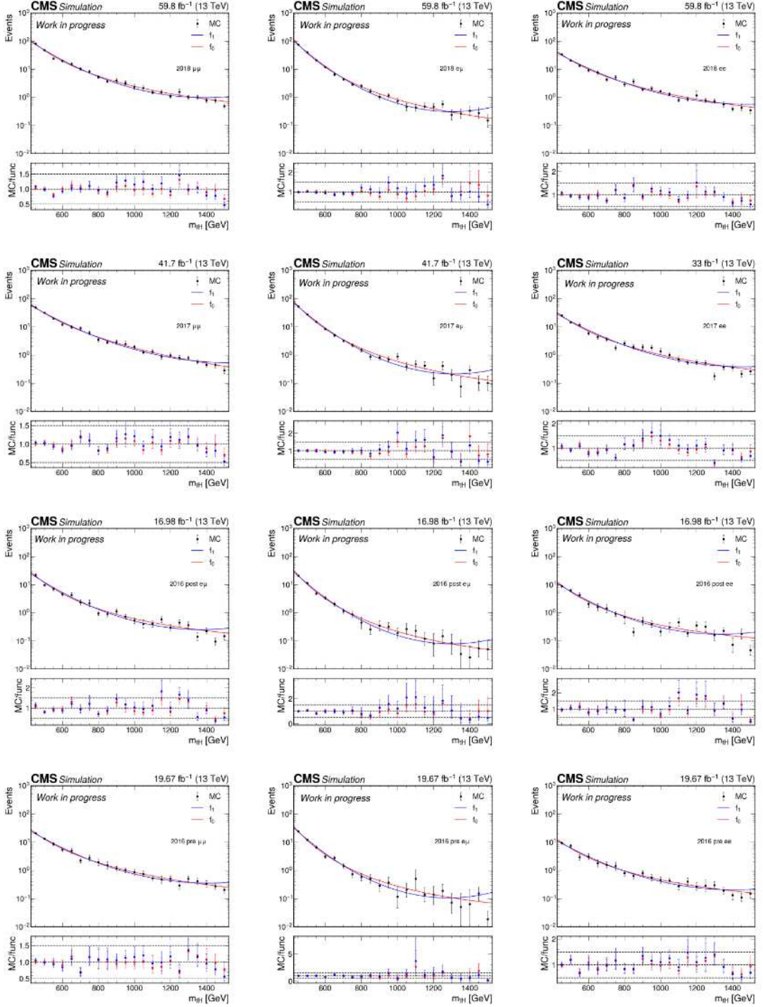
Figure 4.26: Fit background m_{tH} distributions with two PDFs.
