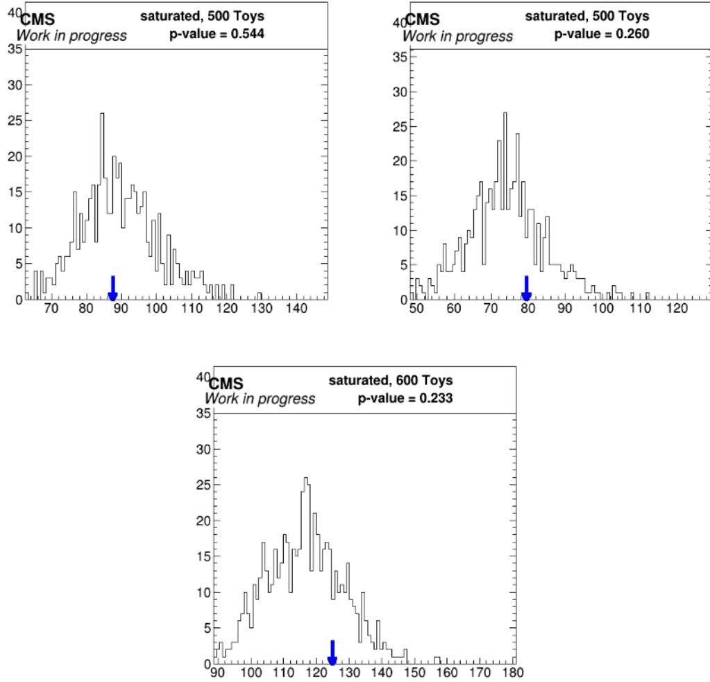
Figure 5.2: GOF tests with signal region data in Run 2, showing \mu\mu , e\mu , and ee channels from left to right.
