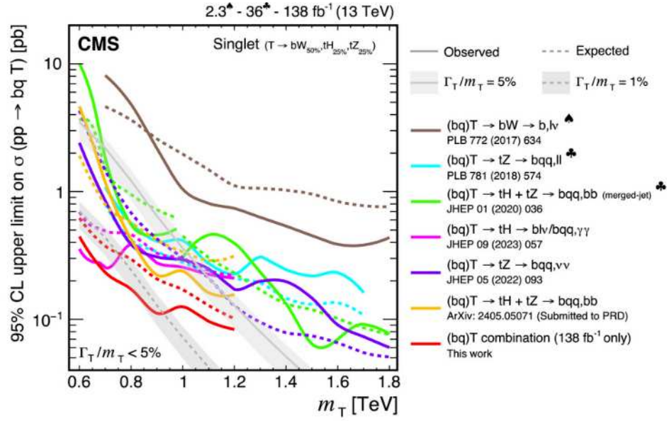
Figure 5.14: The 95% CL observed upper limits on the T single production cross section combining all channels in Run 2. The red curves show the combined results, the other curves show the individual results. Figures from Ref [10]
