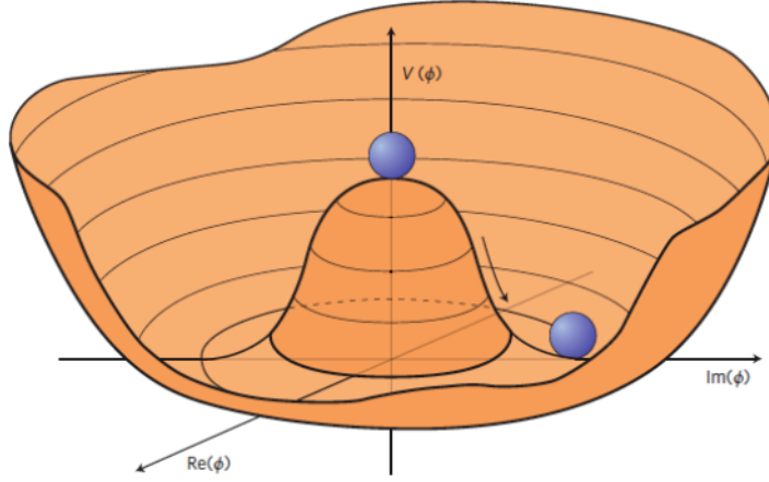
Figure 2.2: Higgs potential when \mu^2 < 0 [20].
