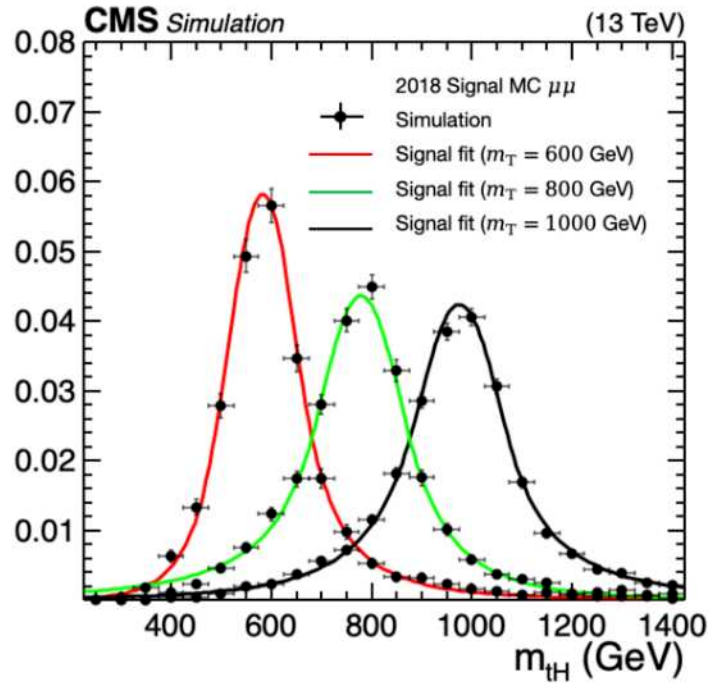
Figure 4.25: Signal models obtained from the m_{tH} distributions, taking the T mass points 600, 800 and 1000 GeV in the 2018 \mu\mu channel as examples.
