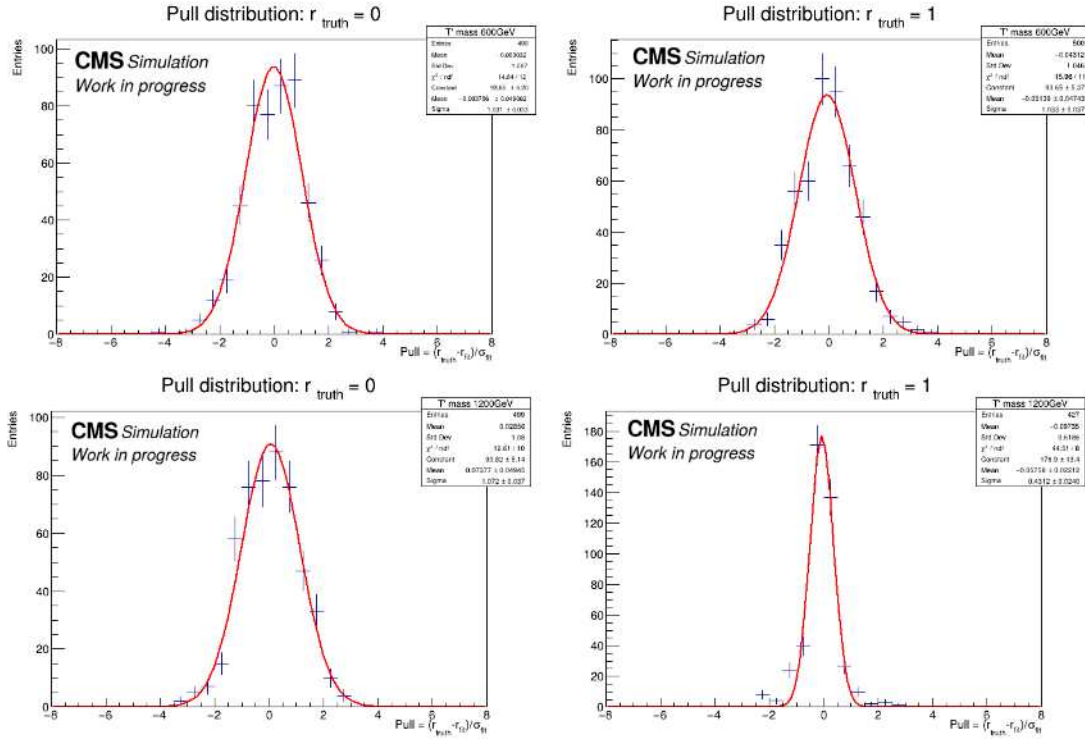
Figure 5.1: Bias test at m_{VLQ} = 600 and 1200 GeV combining all channels in Run 2 with r_{truth} = 1 or 0 assumptions.
