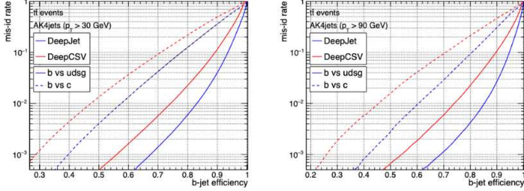
Figure 3.12: DeepJet performance curve: b-jet efficiency vs mis-identification rate [58]
