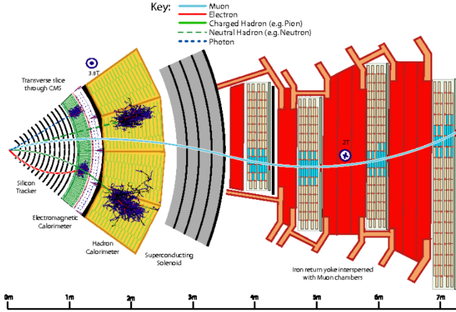
Figure 3.10: Particle interactions in a transverse slice of the CMS detector [45].
