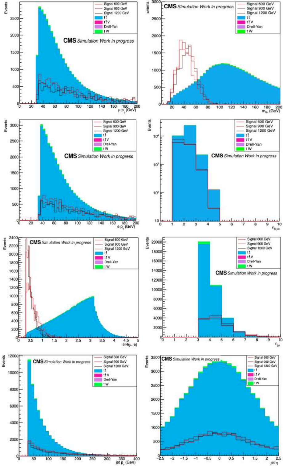
Figure 4.7: Distributions of kinematic variables in e\mu channel after the basic selection.
