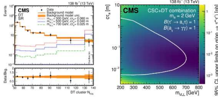
Figure 3: Left: Number of reconstructed hits in signal region of the drift tube category in signal region; Right: 95% CL observed upper limits on the VLL production cross section. Figures from Ref. [3].
