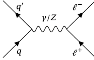
Figure 4.3: DY Z boson production in dilepton final state at LO
