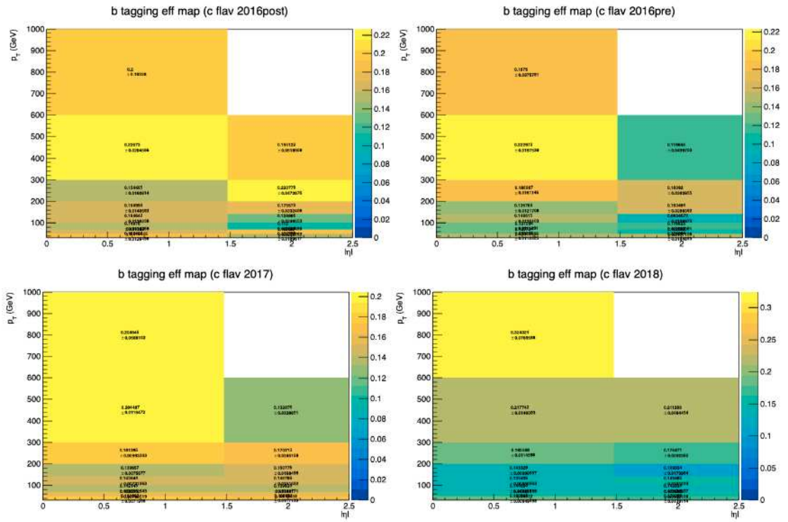
Figure 7.2: B-tagging efficiency maps for each data-taking era. Jets in the maps have hadron flavor 4.
