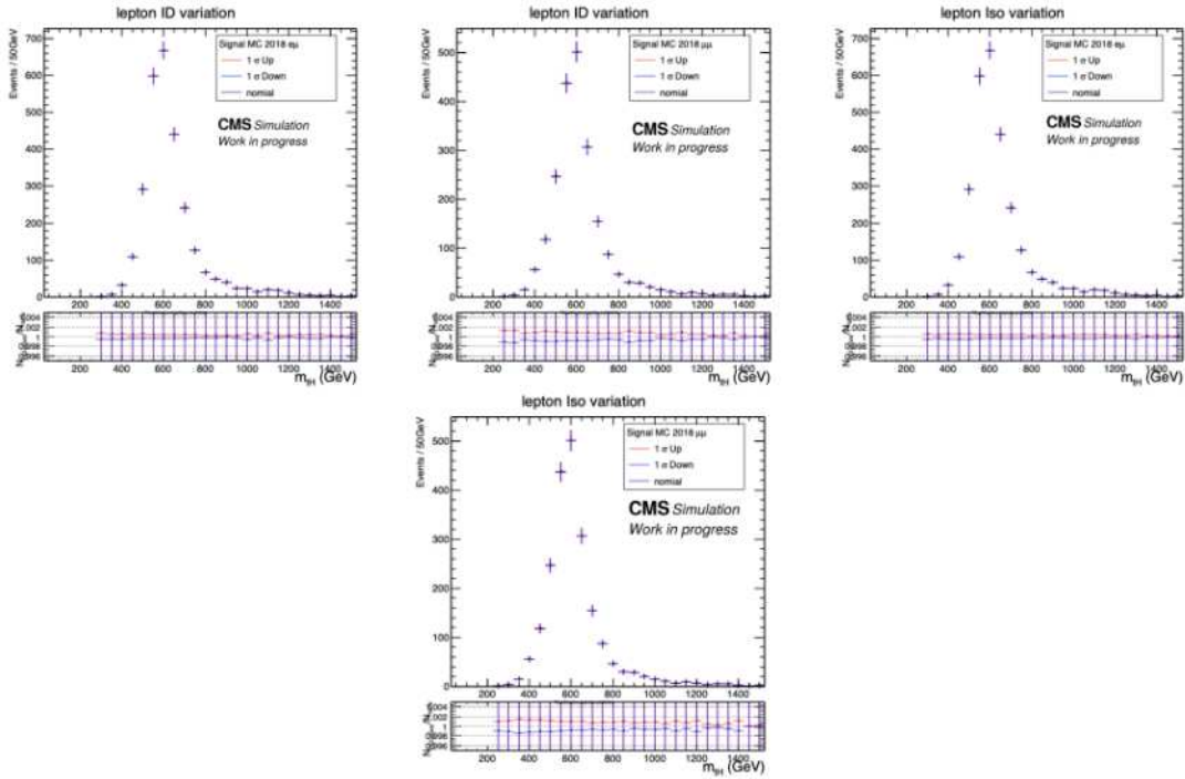
Figure 4.31: Systematic uncertainty study of the muon ID and isolation corrections with signal MC after all analysis cuts, taking 2018 e\mu and \mu\mu channels under m_T = 600 GeV hypothesis as examples.
