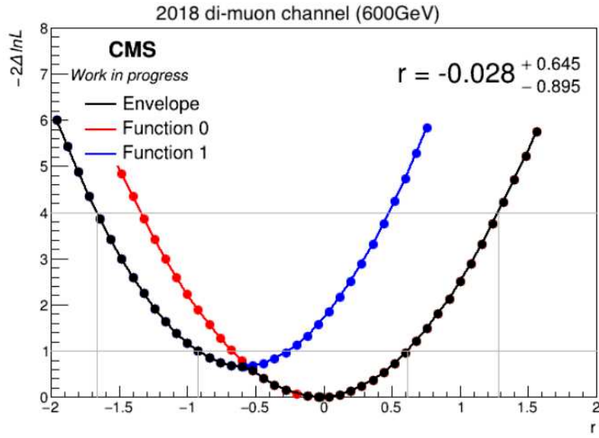
Figure 4.32: Profile scans for the two PDF fits and the envelope obtained from the fits. On the y-axis, -2\Delta\ln\mathcal{L} is twice the negative of the logarithm of the likelihood ratio function, and is equal to \Lambda defined by Equation 4.10. Note that the plot shows the fits to the MC background; thus, it is not used to extract systematic uncertainty. This is only an exercise to illustrate the discrete profiling method.
