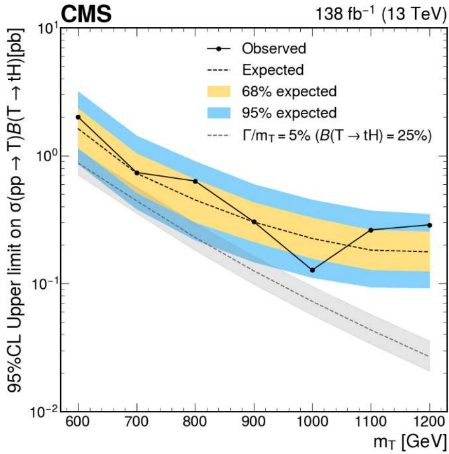
Figure 5.13: Observed upper limits at 95% CL on the production cross section \sigma(pp \rightarrow T)\mathcal{B}(T \rightarrow tH) , combining all OS dilepton channels in the Run 2 dataset.
