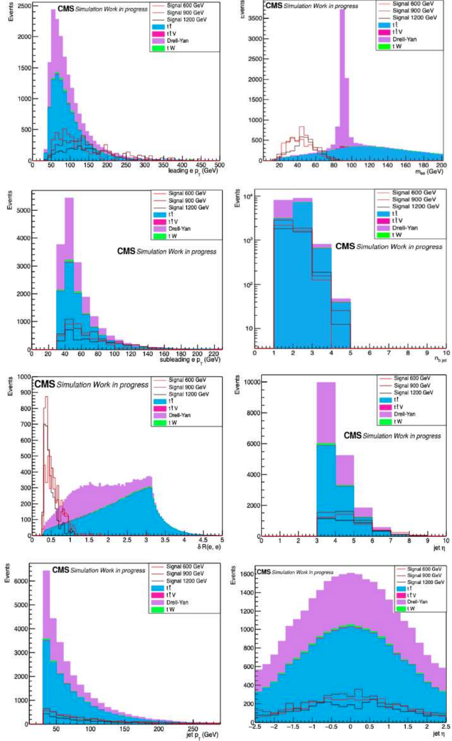
Figure 4.6: Distributions of kinematic variables in ee channel after the basic selection .
