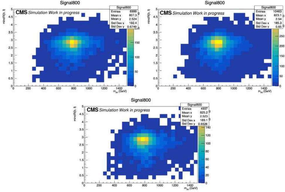
Figure 4.17: Two-dimensional distributions: \Delta R_{\min}(b^t, \ell) and m_{tH} , showing the \mu\mu (upper left), e\mu (upper right) and ee (bottom) channels.
