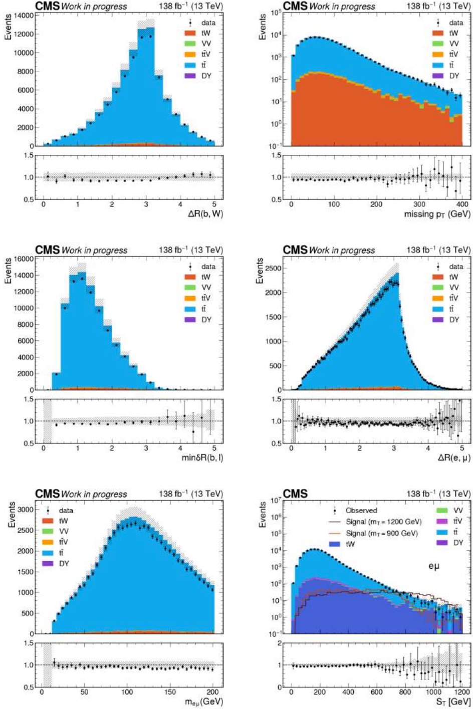
Figure 4.23: Data-MC comparison for the e\mu channel in full Run 2.
