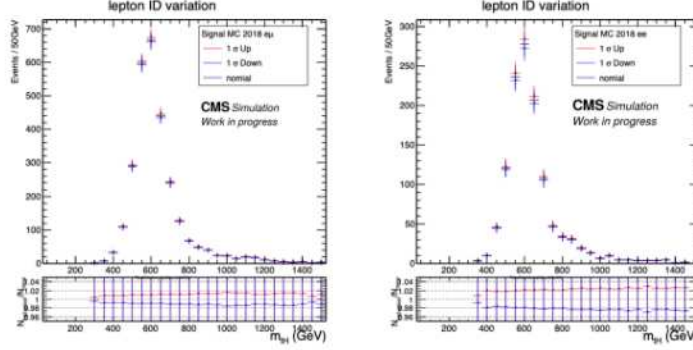
Figure 4.30: Systematic uncertainty study of the electron ID correction with signal MC after all analysis cuts, taking 2018 e\mu and ee channels under m_T = 600 GeV hypothesis as examples.
