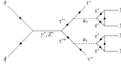
Figure 2: Feynman diagrams showing the productions of VLL, decaying into a_\tau and \tau . Figure from Ref. [3].
