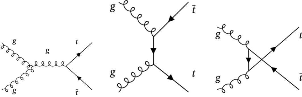
Figure 4.2: t\bar{t} production at LO
