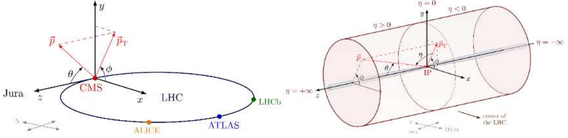
Figure 3.5: The CMS coordinate [33]
