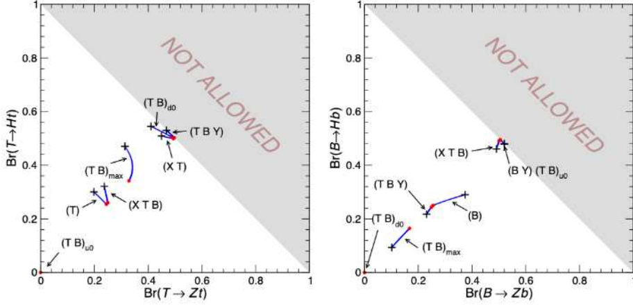
Figure 2.5: Allowed branching ratios for the decays of T and B. Plots are from [9].
