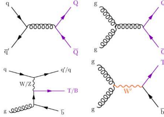
Figure 1: Feynman diagrams showing the productions of VLQ. Figure from Ref. [8].
