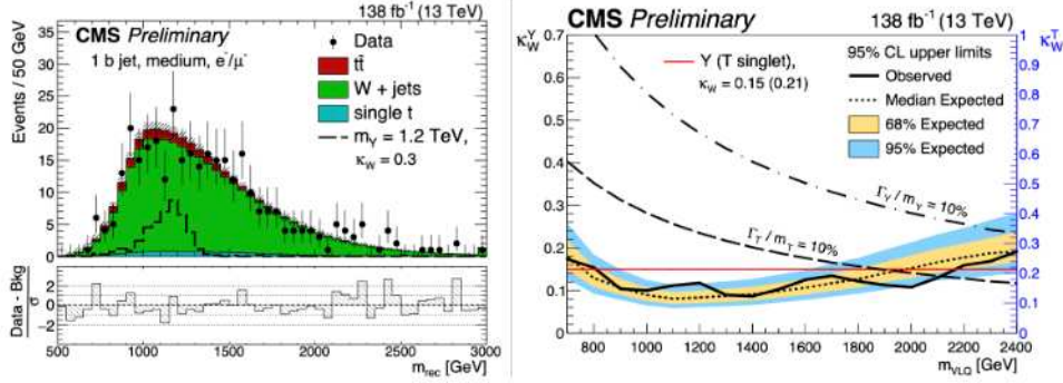
Figure 4: Left: m_{\text{rec}} distribution in signal region after the maximum likelihood fit; Right: The 95% CL observed upper limits on the VLQ coupling parameter. Figures from Ref. [4].
