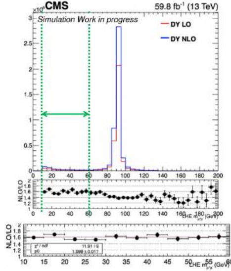
Figure 4.8: Estimate NLO-to-LO correction factor from DY MC
