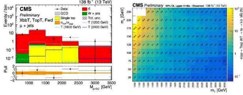
Figure 5: Left: Reconstructed mass of the T candidate in the signal region from one of the categories; Right: The 95% CL observed upper limits on the T production cross section as a function of the T and \phi masses. Figures from Ref. [6].
