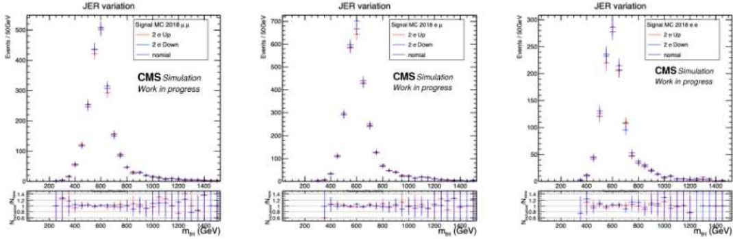
Figure 4.28: Systematic uncertainty study of the JER correction with signal MC after all analysis cuts, taking 2018 \mu\mu , e\mu , and ee channels under m_T = 600 GeV hypothesis as examples.
