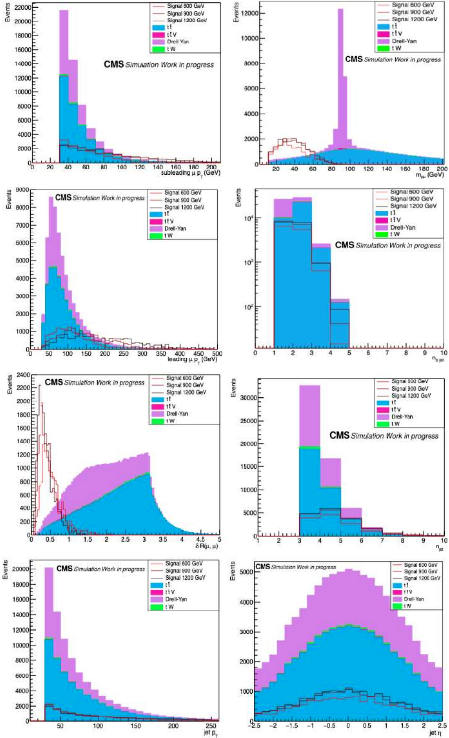
Figure 4.5: Distributions of kinematic variables in the \mu\mu channel after the basic selection.
