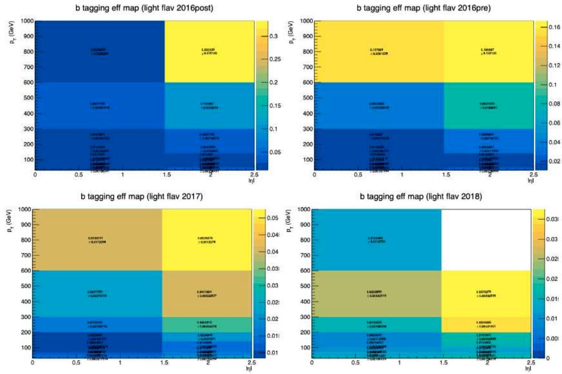
Figure 7.3: B-tagging efficiency maps for each data-taking era. Jets in the maps have hadron flavor 0.
