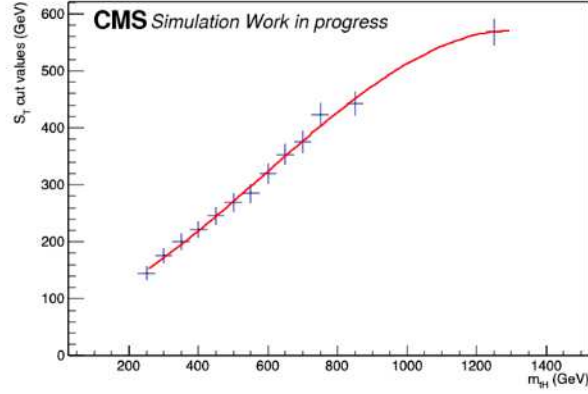
Figure 4.19: The fit used to obtain the f_{\text{cut4}}(m_{tH}) function in S_T cut.
