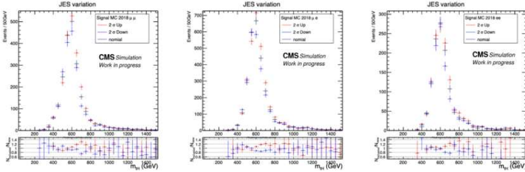
Figure 4.27: Systematic uncertainty study of the JES correction with signal MC after all analysis cuts, taking 2018 \mu\mu , e\mu , and ee channels under m_T = 600 GeV hypothesis as examples.
