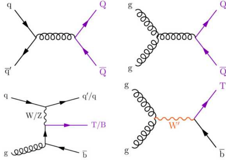
Figure 2.3: Feynman diagrams showing the productions of VLQ. Figure from [10].
