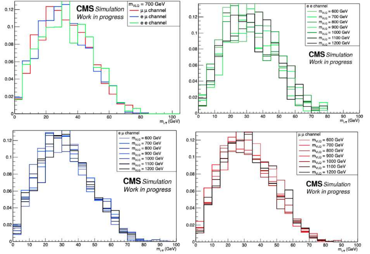
Figure 4.10: m_{\nu\bar{\nu}} distributions in the \mu\mu , e\mu and ee channels and T mass points
