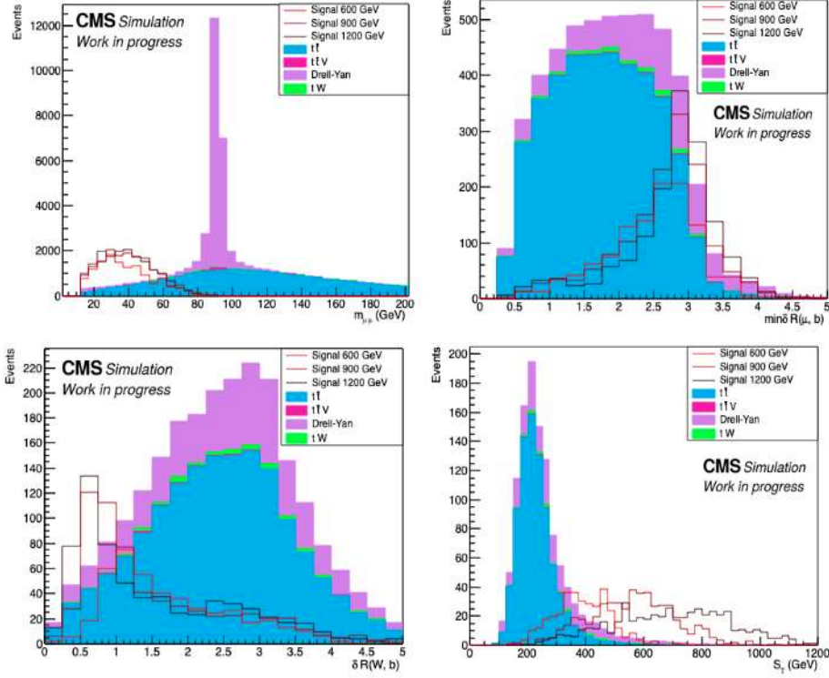
Figure 4.14: The variables used for main selections in \mu\mu channel. The plots show the distributions of m_{\ell\ell} , \delta R_{\min}(b^t, \ell) , \Delta R(b^t, W^t) and S_T before applying requirements on them.
