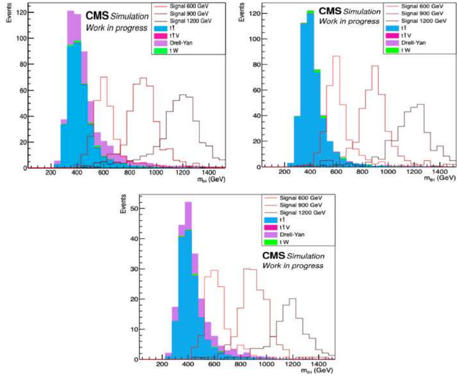
Figure 4.21: m_{tH} distributions of the the \mu\mu (upper left), e\mu (upper right) and ee (bottom) channels after all selections.
