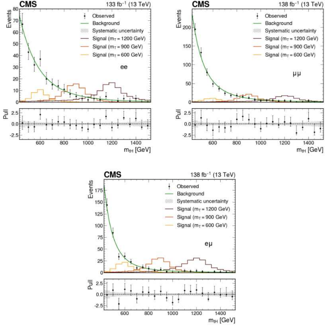
Figure 5.11: Post-fit distributions of the invariant mass m_{tH} in the ee (upper left), \mu\mu (upper right) and e\mu (bottom) channels in Run 2.
