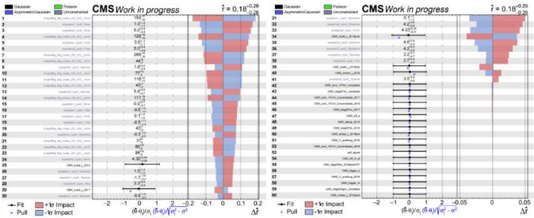
Figure 5.9: Impact plots after unblinding at 600 GeV mass point combining full Run 2.
