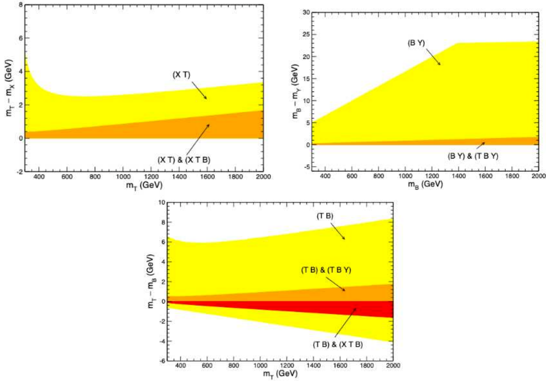
Figure 2.4: Allowed ranges for VLQ mass splittings. Plots are taken from [9].
