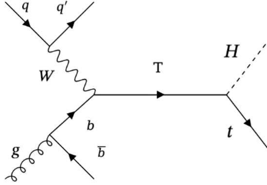
Figure 4.1: Single production of T at LO
