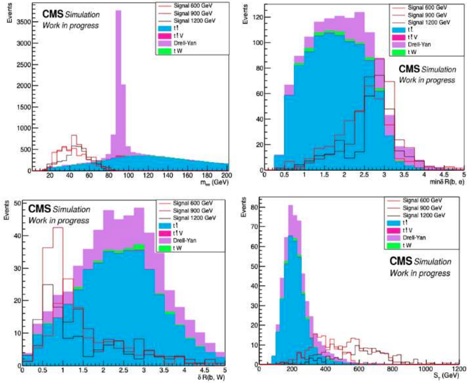
Figure 4.16: The variables used for main selections in ee channel. The plots show the distributions of m_{\ell\ell} , \delta R_{\min}(b^t, \ell) , \Delta R(b^t, W^t) and S_T before applying requirements on them.
