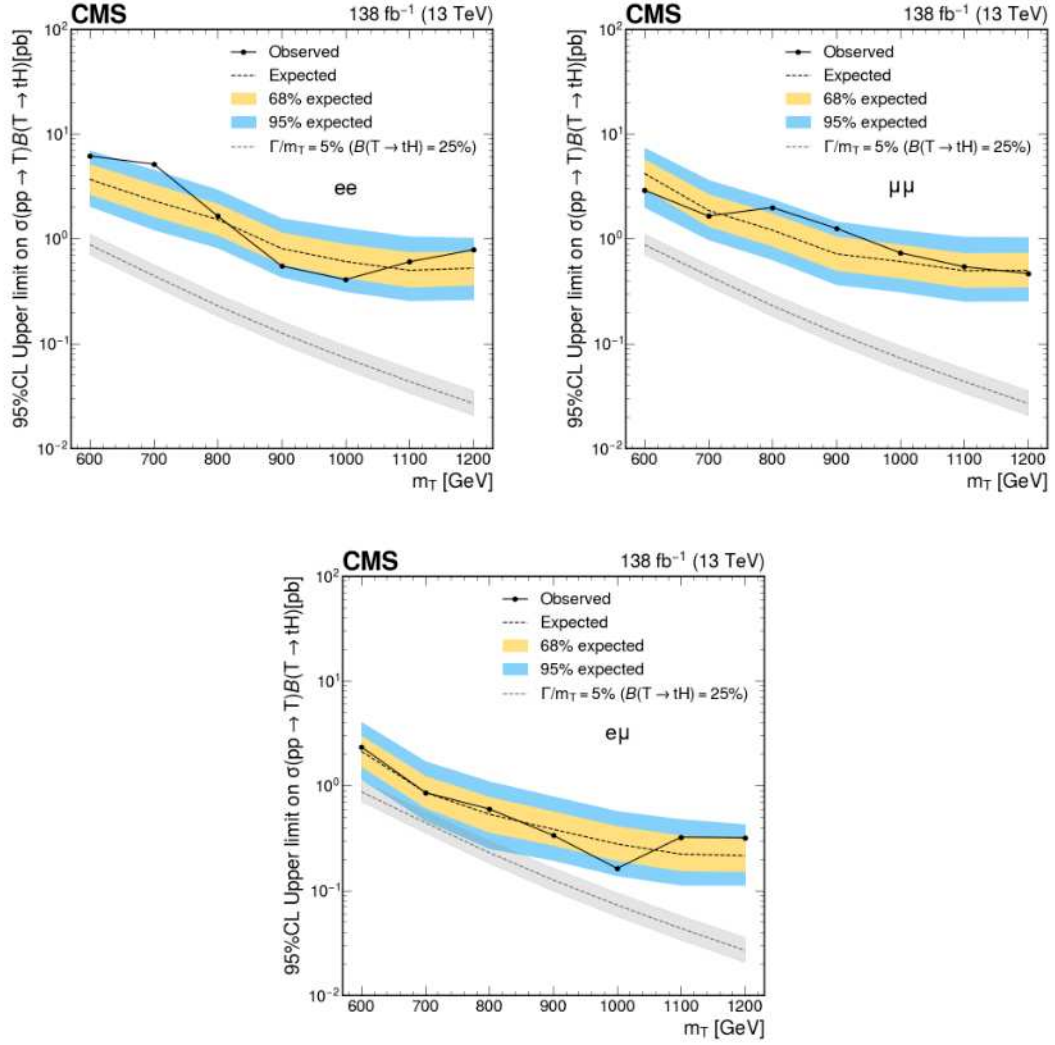
Figure 5.12: Observed upper limits at 95% CL on the production cross section \sigma(pp \rightarrow T)\mathcal{B}(T \rightarrow tH) , for the three OS dilepton channels ee (upper left), \mu\mu (upper right) and e\mu (bottom) in the whole Run 2 dataset.
