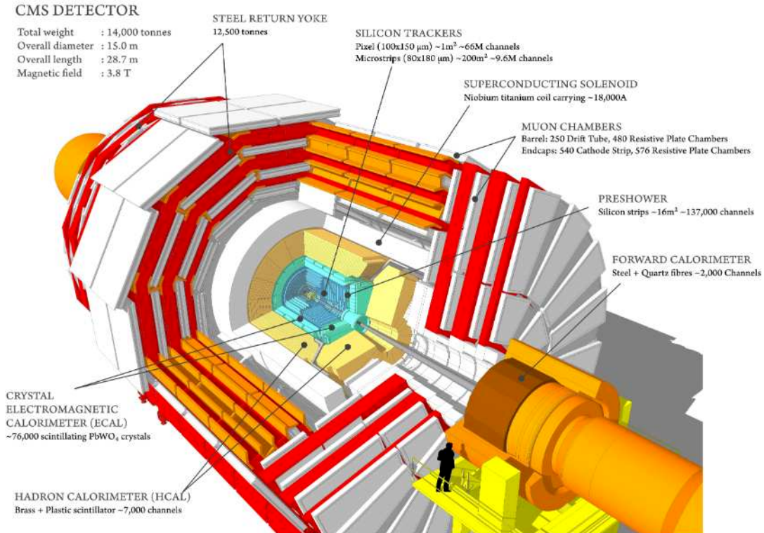
Figure 3.4: The CMS detector overview [32]
