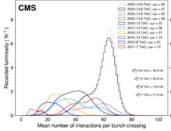
Figure 3.3: Interactions per crossing (pileup) for each year from 2011 to 2025 [30].
