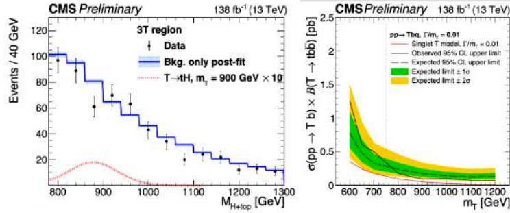
Figure 6: Left: Reconstructed mass of the T candidate in the signal region; Right: The 95% CL observed upper limits on the T production cross section combining all channels in Run 2. Figures from Ref. [7].
