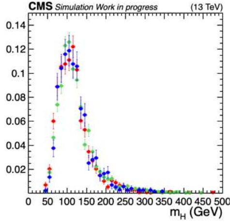
Figure 4.11: Reconstructed Higgs boson mass from signal MC
