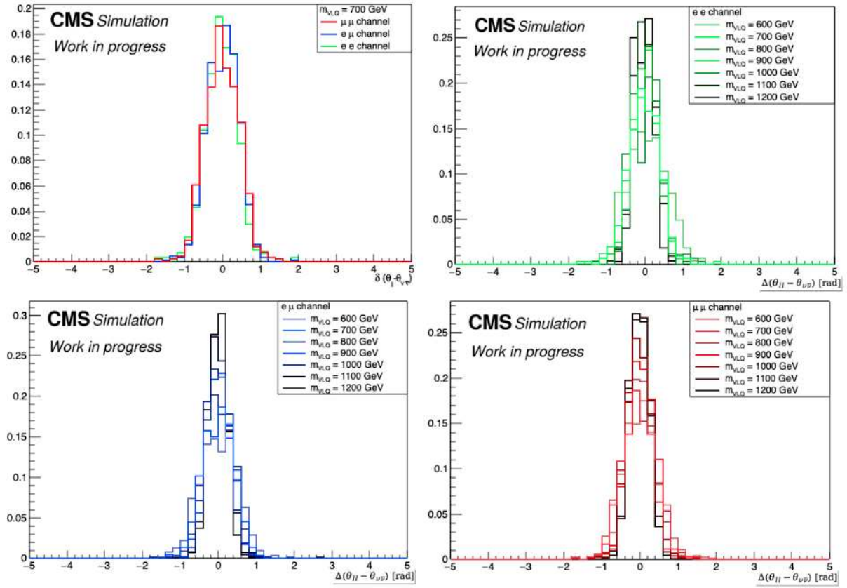
Figure 4.9: Distributions of \theta_{\ell\ell} - \theta_{\nu\bar{\nu}} in the \mu\mu , e\mu and ee channels for various T mass points. The unit on the abscissa is radians (rad).
