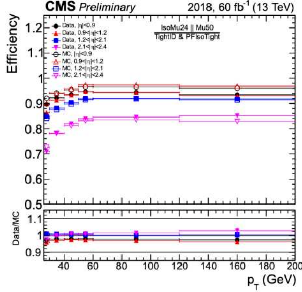
Figure 4.4: Single muon trigger efficiency plot from CMS [63].
