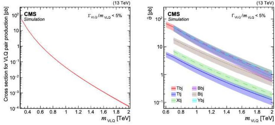
Figure 2.6: Theoretical cross sections of VLQs as a function of VLQ mass. Plots are from [10].
