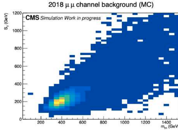
Figure 4.18: Two-dimensional distribution used to determine S_T cut function: S_T and m_{tH} in 2018 \mu\mu channel from the merged background MC.
