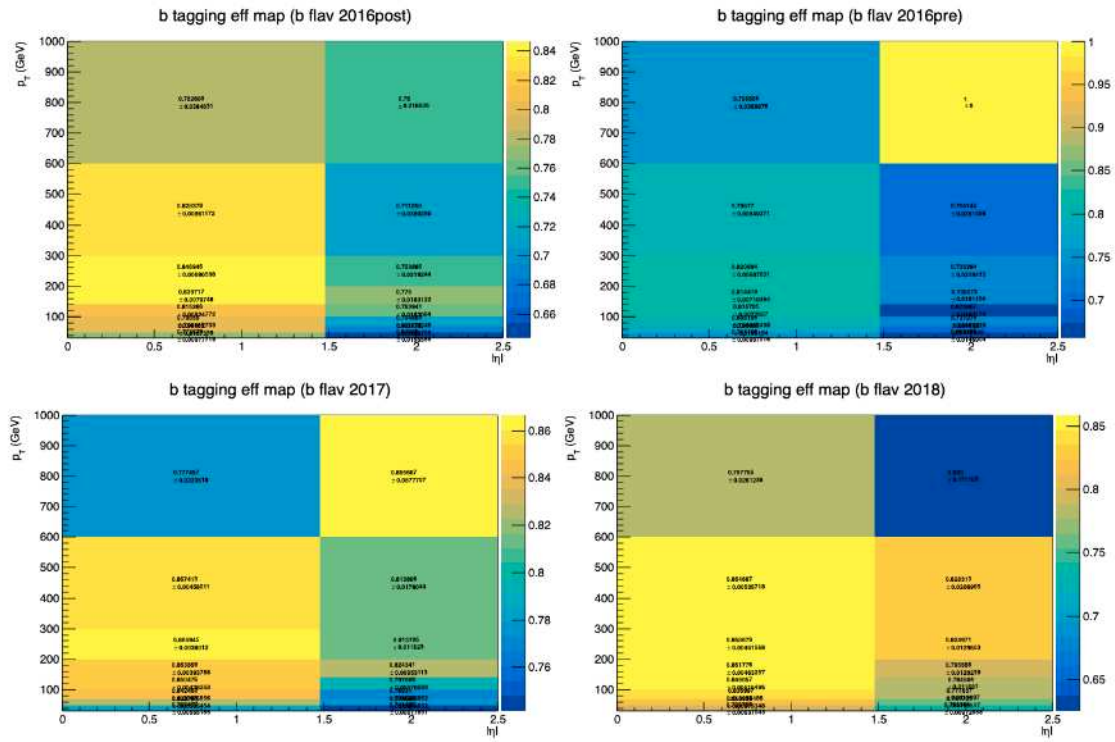
Figure 7.1: B-tagging efficiency maps for each data-taking era. Jets in the maps have hadron flavor 5.
