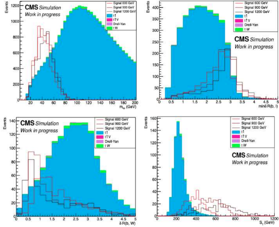
Figure 4.15: The variables used for main selections in e\mu channel. The plots show the distributions of m_{\ell\ell} , \delta R_{\min}(b^t, \ell) , \Delta R(b^t, W^t) and S_T before applying requirements on them.
