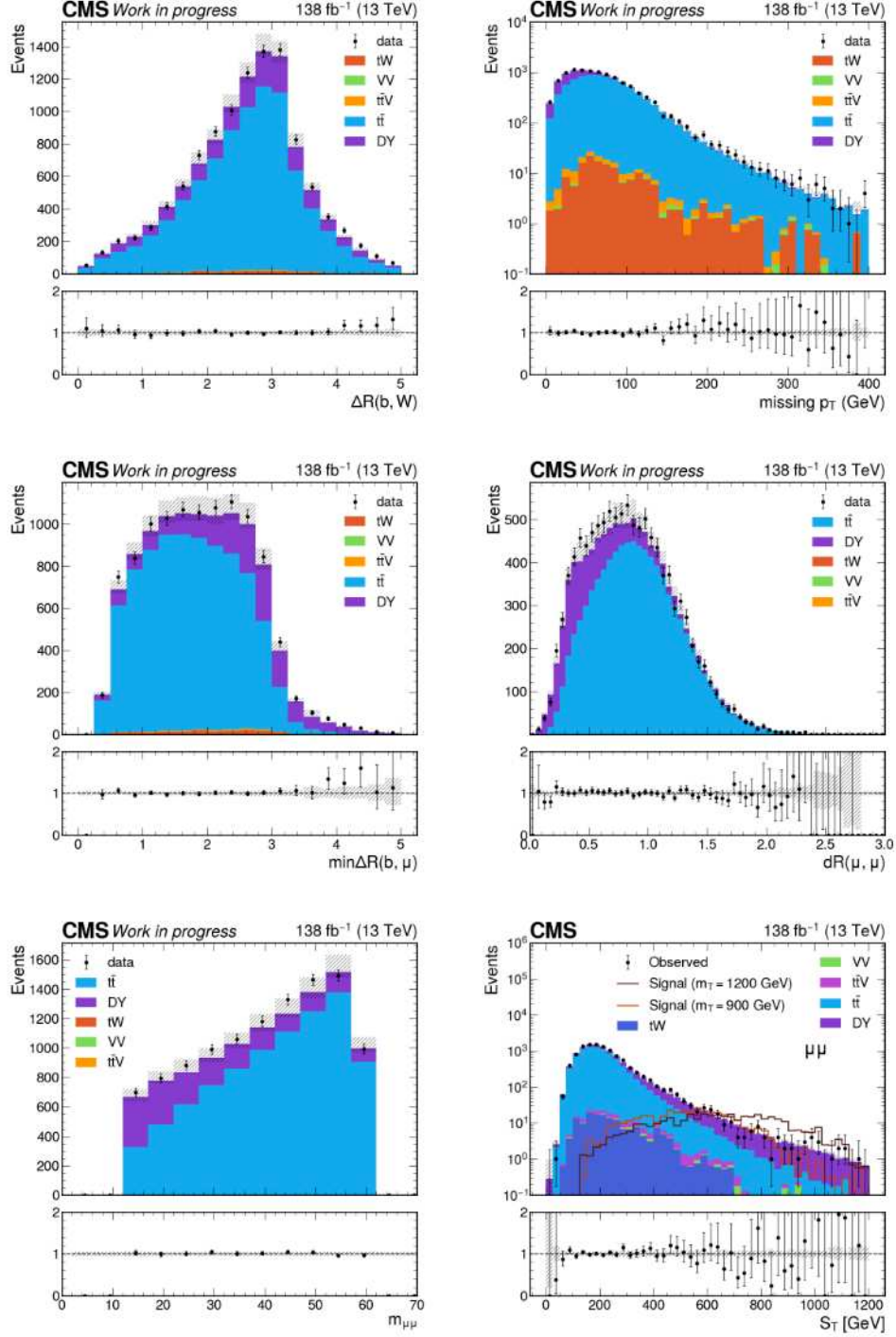
Figure 4.22: Data-MC comparison for the \mu\mu channel in full Run 2.
