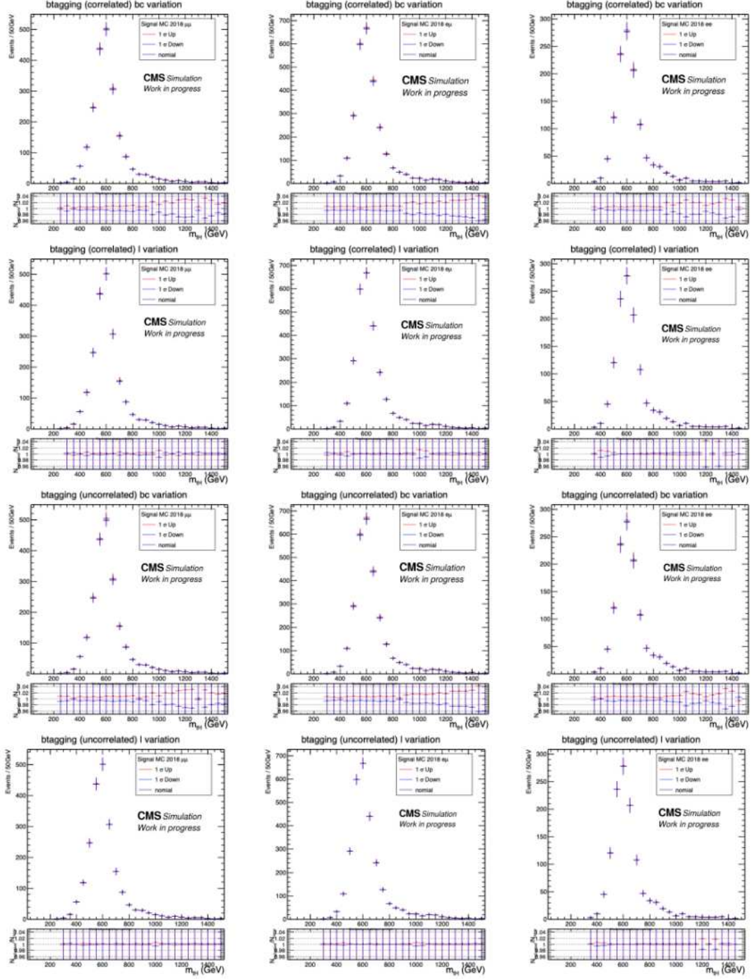
Figure 4.29: Systematic uncertainty study of b tagging corrections with signal MC after all analysis cuts
