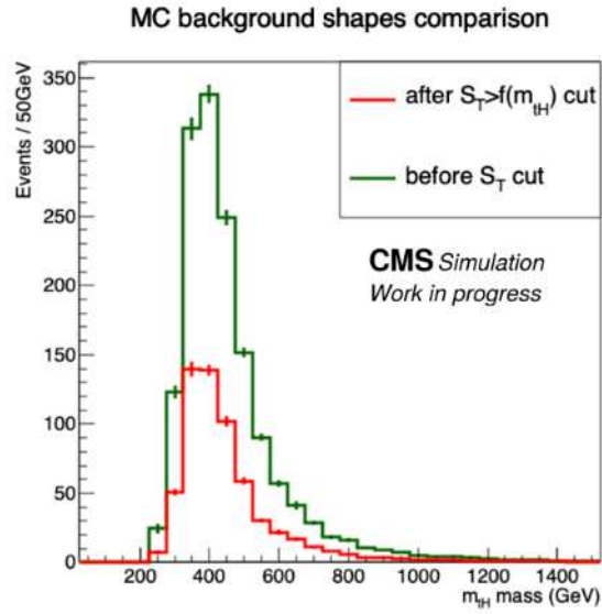
Figure 4.20: m_{tH} distributions of 2018 \mu\mu channel from background MC before and after the sliding S_T cut.
