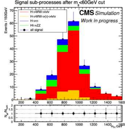
Figure 4.13: Combinations of sub-processes in the signal MC, shown for m_T = 800 \text{ GeV} .
