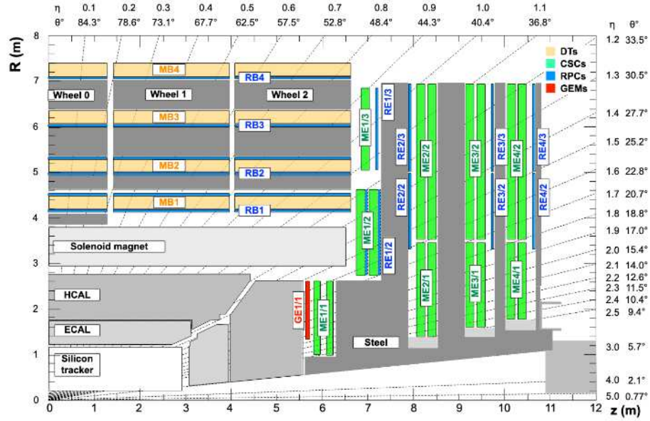
Figure 3.9: The CMS muon detector system [43].
