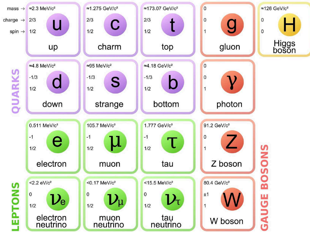
Figure 2.1: Summary of SM particles [17].
