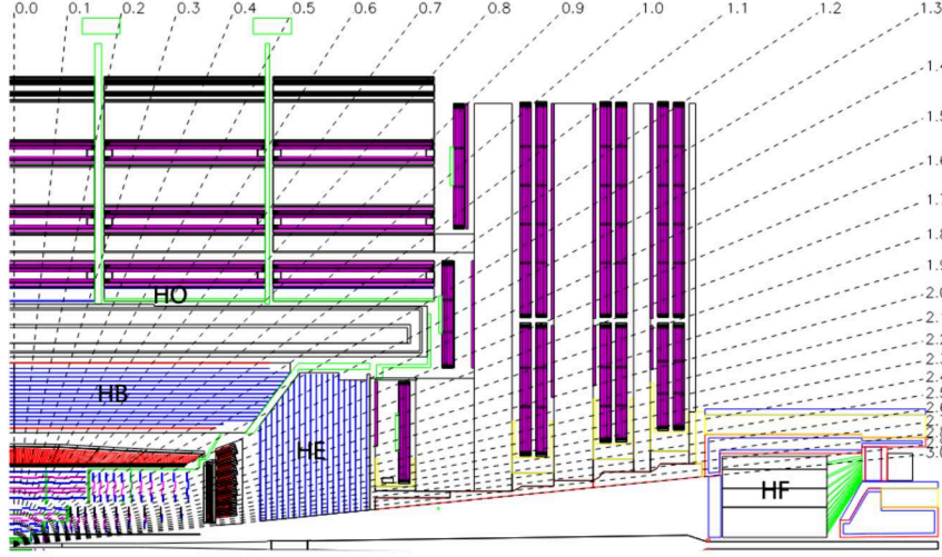
Figure 3.8: The CMS HCAL layout [40]
