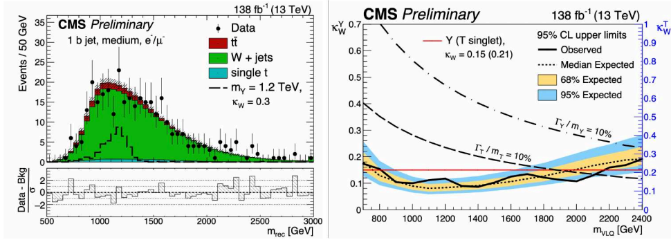
Figure 4: Left: m_{\text{rec}} distribution in signal region after the maximum likelihood fit; Right: The 95% CL observed upper limits on the VLQ coupling parameter. Figures from Ref. [4].
