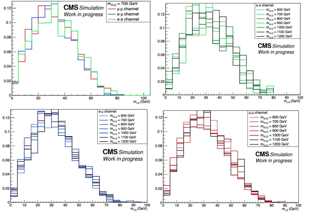
Figure 4.10: m_{\nu\bar{\nu}} distributions in the \mu\mu , e\mu and ee channels and T mass points
