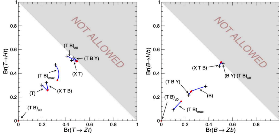
Figure 2.5: Allowed branching ratios for the decays of T and B. Plots are from [9].
