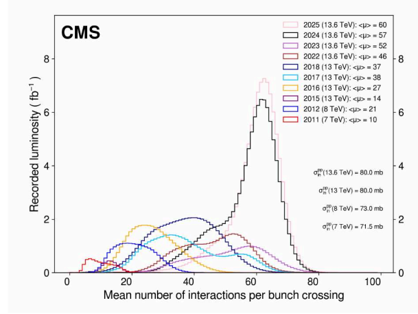
Figure 3.3: Interactions per crossing (pileup) for each year from 2011 to 2025 [30].
