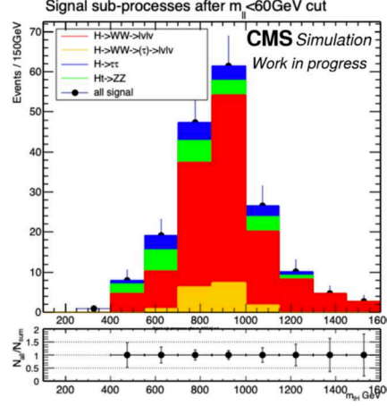
Figure 4.13: Combinations of sub-processes in the signal MC, shown for m_T = 800 GeV.
