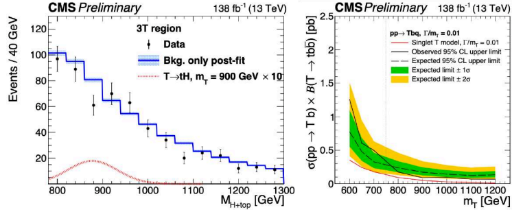
Figure 6: Left: Reconstructed mass of the T candidate in the signal region; Right: The 95% CL observed upper limits on the T production cross section combining all channels in Run 2. Figures from Ref. [7].
