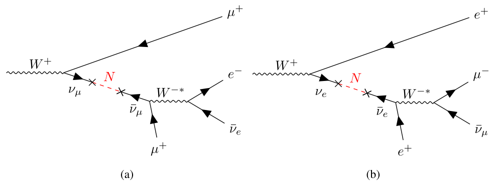
Fig. 1 Feynman diagrams for heavy neutral lepton ( N ) production and decay in the channels originating from: (a) \text{HNL}-\nu_\mu mixing and \mu^+e^-\bar{\nu}_e decay of the heavy lepton, and (b) \text{HNL}-\nu_e mixing and e^+\mu^-\bar{\nu}_\mu decay of the heavy lepton. Only lepton-number-violating processes are considered
