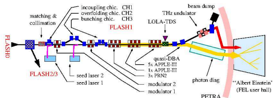
Figure 4: Schematic view of the FLASH1 design after the shutdown.
