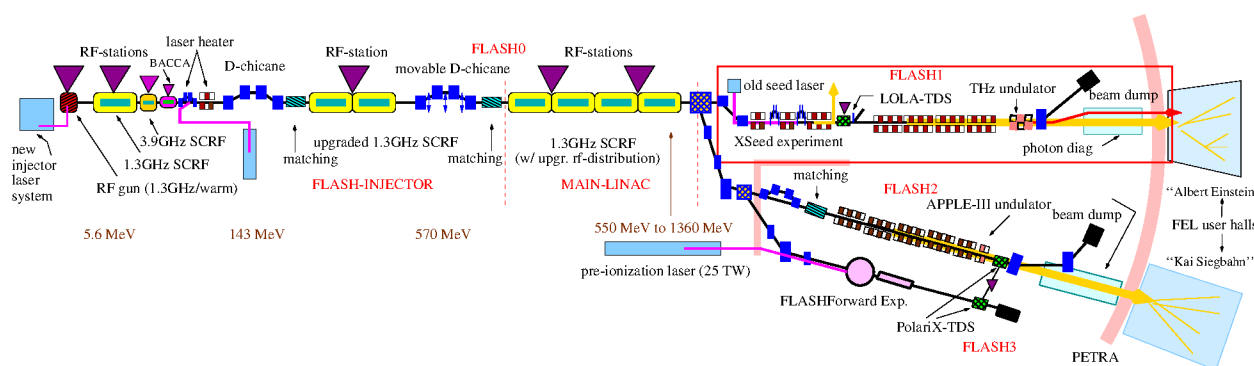
Figure 1: Schematic view of FLASH in 2024. The part in the red rectangle (FLASH1) was completely removed and is being rebuild during the ongoing shutdown.
