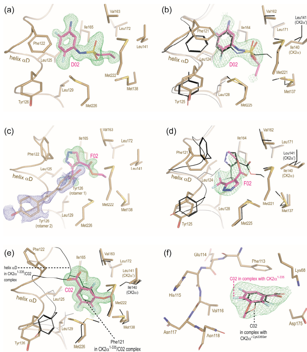
Figure 4. Fragments of the F2X-Entry screen [38] binding to the \alpha D pocket of CK2 \alpha^{\text{Cys336Ser}} . (a) Fragment D02 in the \alpha D pocket of CK2 \alpha^{\text{Cys336Ser}} . (b) Fragment D02 in the \alpha D pocket of CK2 \alpha^{1-335} ; for comparison, the equivalent part of the CK2 \alpha^{\text{Cys336Ser}} /D02 complex structure was drawn with black C-atoms. (c) Fragment F02 in the \alpha D pocket of CK2 \alpha^{\text{Cys336Ser}} . (d) Fragment F02 in the \alpha D pocket of CK2 \alpha^{1-335} ; for comparison, the equivalent part of the CK2 \alpha^{\text{Cys336Ser}} /F02 complex structure was drawn with black C-atoms. (e) Fragment C02 in the \alpha D pocket of CK2 \alpha^{\text{Cys336Ser}} ; for comparison, the equivalent part of the CK2 \alpha^{1-335} /C02 complex structure was drawn with black C-atoms. (f) Fragment C02 at the ATP/GTP cavity of CK2 \alpha^{1-335} ; for comparison, C02 as bound to the ATP/GTP cavity of CK2 \alpha^{\text{Cys336Ser}} .
