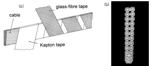
Figure 20: (a) Rutherford cable with Kapton and glass-fibre insulation such as used in the Tevatron and HERA magnets. The glass-fibre tape is pre-impregnated with B-stage epoxy which cures at temperatures above 120^\circ\text{C} . In the RHIC and LHC coils the second insulation layer is also made from Kapton. (b) Cross section of the cable.
