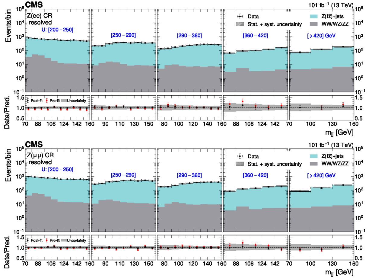
Figure 6: The dijet m_{jj} distributions after the simultaneous likelihood background-only fit sliced in five U bins, for the resolved-category Z(ee) (above) and Z(\mu\mu) (below) CRs. The black markers with statistical uncertainty bars show the observed data, the stacked colored histograms show the predicted background, and the gray shading shows the systematic uncertainty in the prediction. The lower panels show the ratios of the observed data to the background predicted before (pre-fit in red) and after (post-fit in black) the fit, with the gray bands indicating the post-fit uncertainty obtained from combining all statistical and systematic sources.
