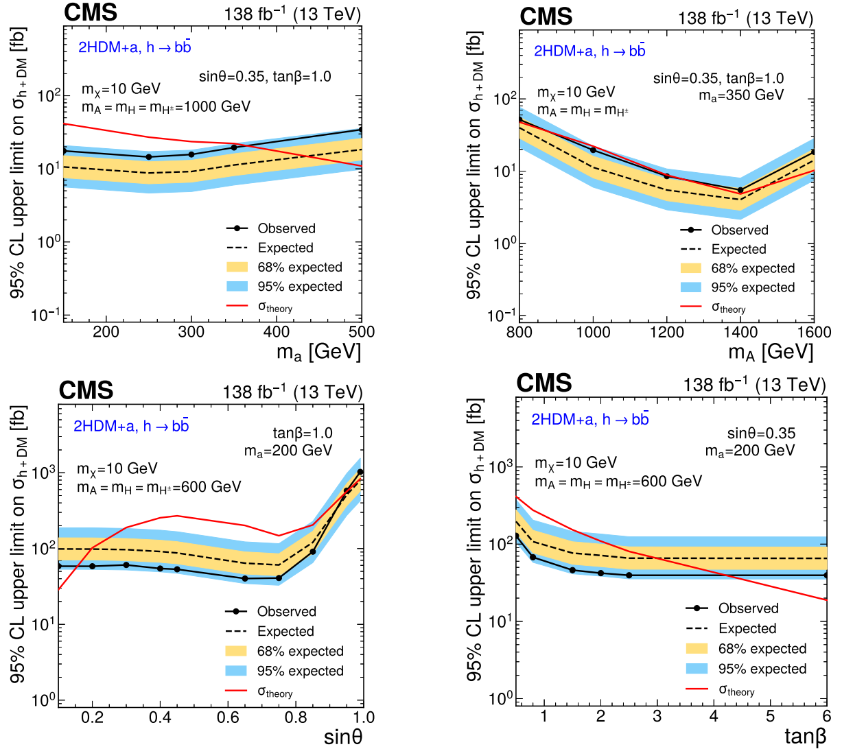
Figure 9: Observed and expected exclusion limits at 95% CL on the signal cross section \sigma_{h+DM} for the 2HDM+a model as a function of the model parameters: m_a (upper left), m_A (upper right), \sin \theta (lower left), and \tan \beta (lower right) while fixing the values of the other parameters, as indicated in the legends. Different sets of model parameters are tested to probe distinct regions of phase space. Mass points below the solid red line are excluded.
