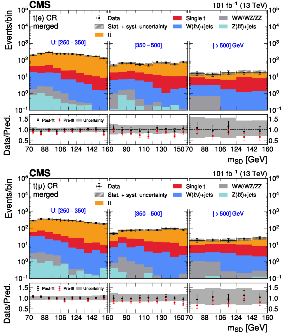
Figure 3: The AK8 jet m_{SD} distributions after the simultaneous likelihood background-only fit sliced in three U bins, for the merged-category t(e) (above) and t(\mu) (below) CRs. The black markers with statistical uncertainty bars show the observed data, the stacked colored histograms show the predicted background, and the gray shading shows the systematic uncertainty in the prediction. The lower panels show the ratios of the observed data to the background predicted before (pre-fit in red) and after (post-fit in black) the fit, with the gray bands indicating the post-fit uncertainty obtained from combining all statistical and systematic sources.
