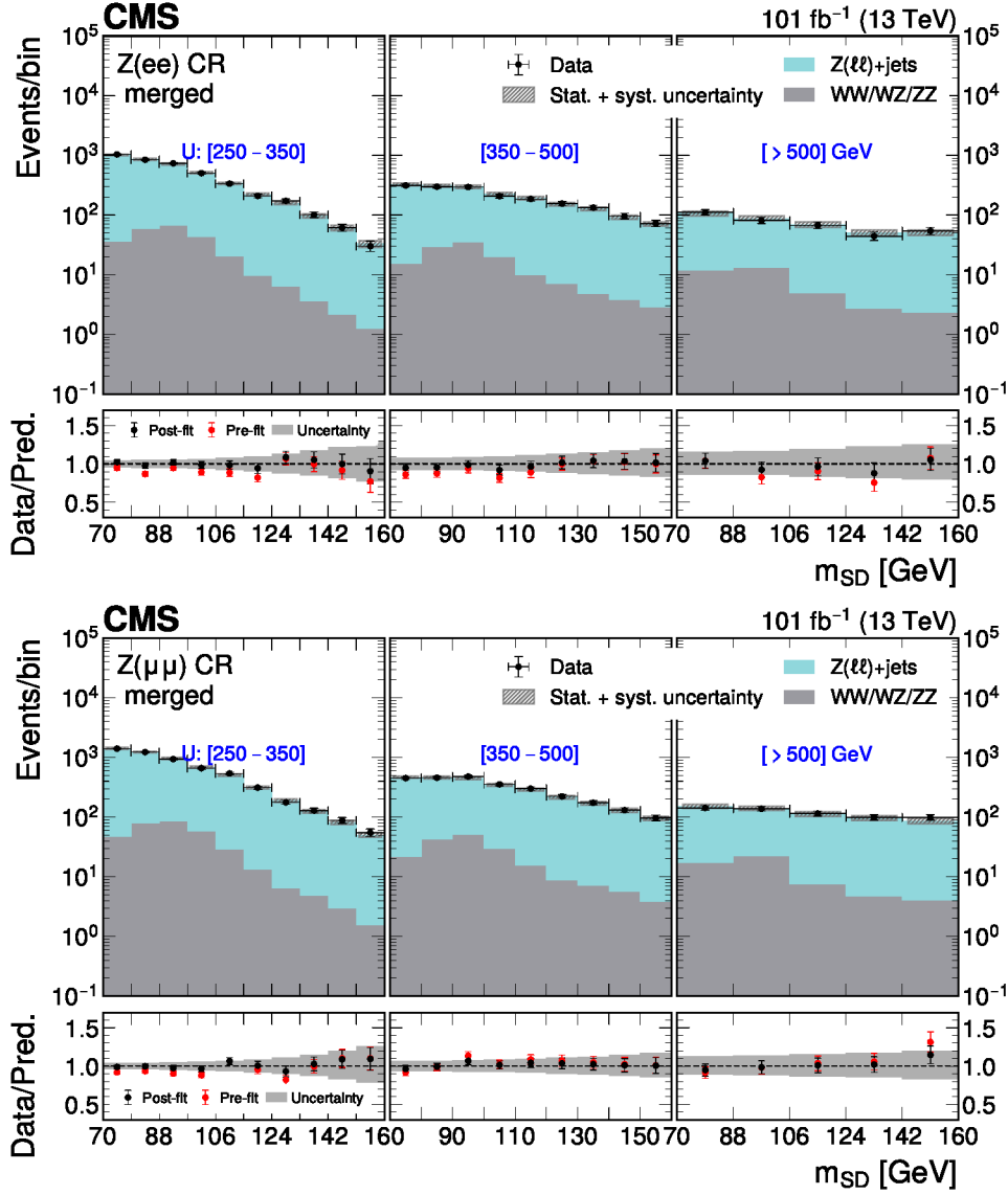
Figure 4: The AK8 jet m_{SD} distributions after the simultaneous likelihood background-only fit sliced in three U bins, for the merged-category Z(ee) (above) and Z(\mu\mu) (below) CRs. The black markers with statistical uncertainty bars show the observed data, the stacked colored histograms show the predicted background, and the gray shading shows the systematic uncertainty in the prediction. The lower panels show the ratios of the observed data to the background predicted before (pre-fit in red) and after (post-fit in black) the fit, with the gray bands indicating the post-fit uncertainty obtained from combining all statistical and systematic sources.
