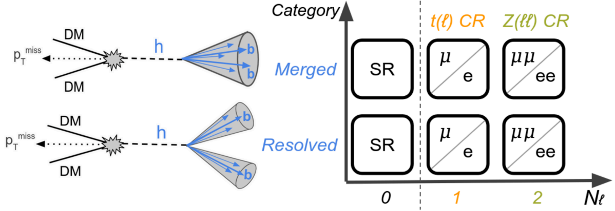
Figure 2: Schematic representation of the analysis regions.
