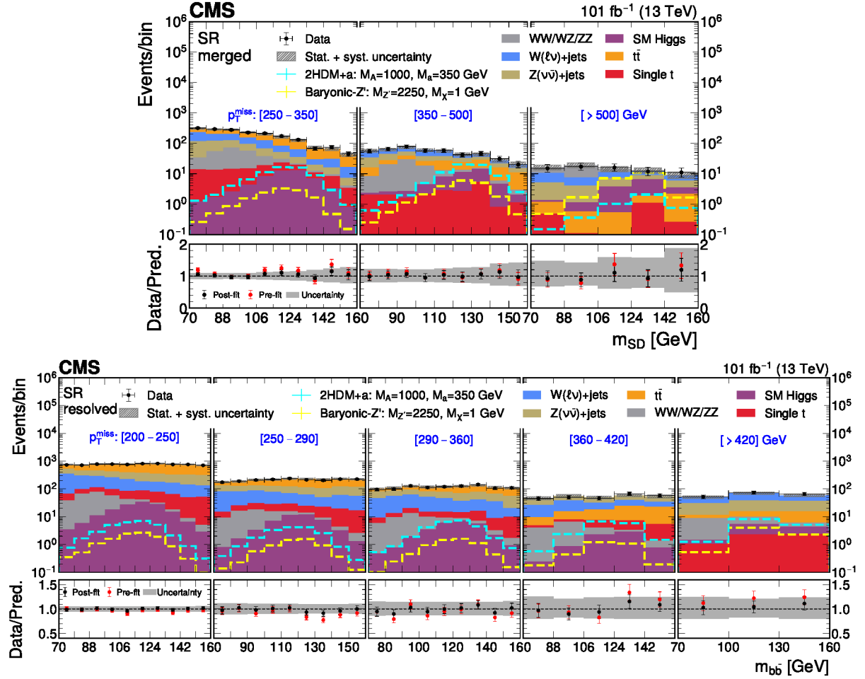
Figure 7: The AK8 jet m_{\text{SD}} (above) and dijet m_{b\bar{b}} (below) distributions after the simultaneous likelihood background-only fit sliced in three and five p_T^{\text{miss}} bins, for the merged- and resolved-category SRs respectively. The black markers with statistical uncertainty bars show the observed data, the stacked colored histograms show the predicted background, and the gray shading shows the systematic uncertainty in the prediction. The signal predictions are overlaid as cyan and yellow dashed lines, one for each benchmark model. The lower panels show the ratios of the observed data to pre-fit (red points) and post-fit (black points) background predictions, with the gray bands indicating the post-fit uncertainty obtained from combining all statistical and systematic sources.
