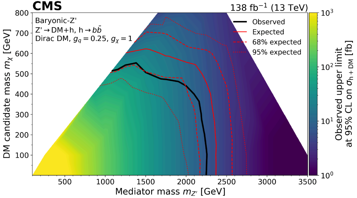
Figure 8: Exclusion limits at 95% CL on the signal cross section \sigma_{h+DM} for the baryonic- Z' model as a function of m_{Z'} and m_\chi . The coupling parameters are fixed to g_q = 0.25 and g_\chi = 1 . The areas within the solid black and red contours represent the exclusion regions where the theoretical cross sections are larger than the observed and expected experimental limits, respectively. The areas within the dashed and dotted red contours show the excluded regions at \pm 1 and \pm 2 standard deviations from the expected limits, respectively.
