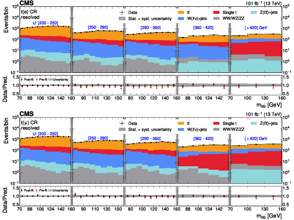
Figure 5: The dijet m_{b\bar{b}} distributions after the simultaneous likelihood background-only fit sliced in five U bins, for the resolved-category t(e) (above) and t(\mu) (below) CRs. The black markers with statistical uncertainty bars show the observed data, the stacked colored histograms show the predicted background, and the gray shading shows the systematic uncertainty in the prediction. The lower panels show the ratios of the observed data to the background predicted before (pre-fit in red) and after (post-fit in black) the fit, with the gray bands indicating the post-fit uncertainty obtained from combining all statistical and systematic sources.
