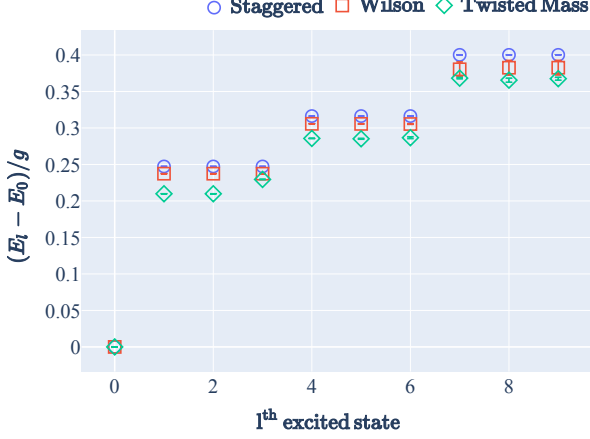
(a) Energy gap \Delta E = E_l - E_0 for the ten lowest-energy states.
