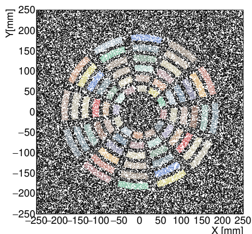
Figure 16. A dummy mask pattern illustrating the result of a RingMask and SpiderMask class built through the CombinedMask class. This illustration was produced using a Monte Carlo simulation. Different colors represent regions with unique IDs, while black dots represent areas where no region is found.
