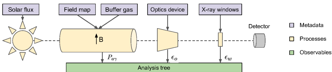
Figure 7. A schematic of the four main processes in the ray-tracing event processing chain: Generator , FieldPropagation , Optics , and Transmission . Metadata components correspond to those described in section 3. All processes, except for Generator , add observables to the analysis tree, such as the axion-photon conversion probability, P_{a\gamma} , the optics efficiency, \epsilon_o , and the windows transmission efficiency, \epsilon_w , for each event.
