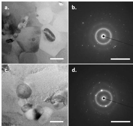
Fig. 10 TEM-BF images and the corresponding SAED patterns of MAPHEUS-10 \mu g-sample (a.-b.) and lab equivalent (c.-d.) near the interface of two layers. Scale bar of BF images (a., c.) is 100 nm and of SAED patterns (b., d.) 10 \text{ nm}^{-1}
