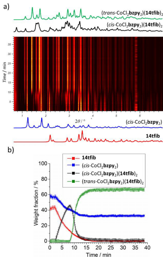
Figure 2. Results of in situ synchrotron PXRD ( \lambda = 0.20\ 709\ \text{\AA} ) monitoring of the reaction of equimolar amounts of \text{cis-CoCl}_2\text{bzpy}_2 and 14tfib : a) the time-resolved 2D PXRD plot, b) results of quantitative Rietveld analysis of the in situ obtained data.
