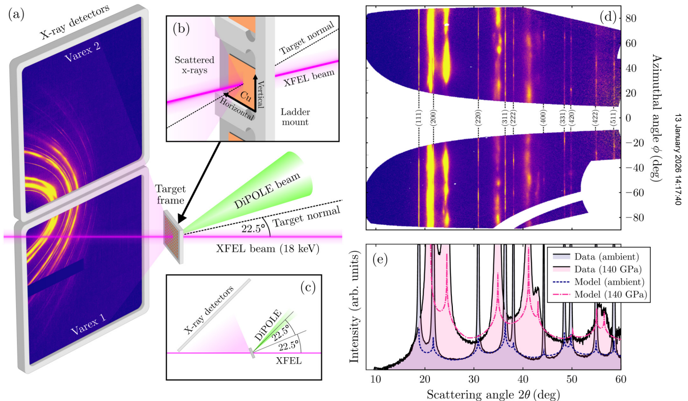
FIG. 4. X-ray thermal diffuse scattering (TDS) patterns obtained from shock-compressed Cu at the High Energy Density (HED) instrument of the European X-Ray Free-Electron Laser (EuXFEL). 36 (a) Experimental configuration. Copper foils are dynamically loaded using the DiPOLE 100-X laser and simultaneously probed by an 18 keV photon beam inclined at 22.5^\circ to the target normal. Diffraction is captured on a pair of symmetrically displaced megapixel Varex detectors in transmission geometry. (b) Close-up of an individual Cu target viewed downstream, indicating the sense of the “vertical” and “horizontal” directions. (c) Configuration viewed in the horizontal plane. (d) Full diffraction pattern from Cu shock-compressed to 140 GPa, presented in (2\theta, \phi) -space. White regions either fall outside detector coverage, were obscured by shadows, or failed to have data recorded. (e) Azimuthally averaged scattering from an ambient (blue) and a driven (pink) shot shown at the scale of the TDS. Data are normalized to the incident photon flux, corrected to exclude polarization, per-pixel solid angle, and all attenuation factors, and have had Compton scattering and scattering from the drive-side ablator layer subtracted. The inter-Bragg regions of each pattern are fitted to Warren’s TDS model for a perfectly random power (dashed lines).
