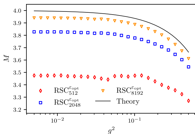
Fig. 6 The mass gap M as a function of the coupling g^2 for different fixed partitioning sizes. \varepsilon_{\text{Tr}} is chosen separately at each coupling according to the fits found in Fig. 5
