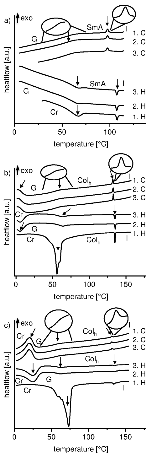
Figure 5: Representative DSC thermograms of c-DOPA(n) • KPF 6 with a) n = 12 b) n = 14 c) n = 16 , heating rate: 5 K/min.
