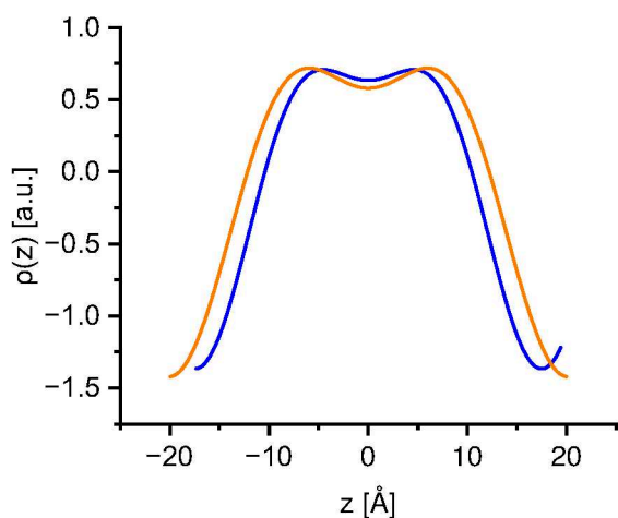
Figure 8: 1D electron density distribution of c-DOPA(12) • KI (blue) and c-DOPA(14) • KI (orange).
