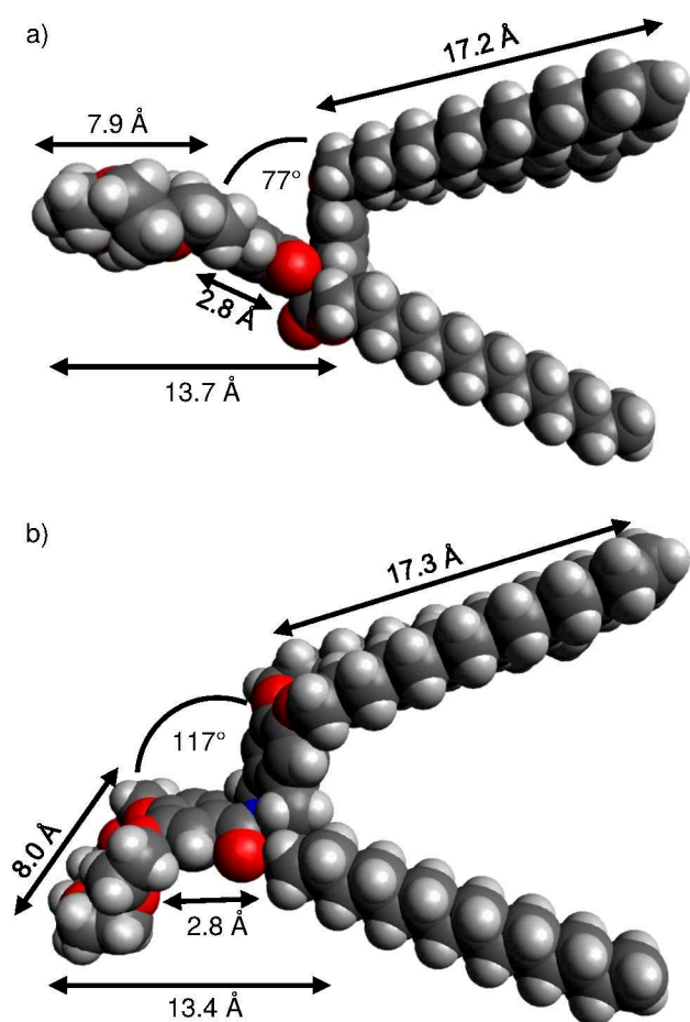
Figure 7: Optimized molecular geometry of a) c-DOPA(14) • KI and b) c-THIQ(14) • KI .
