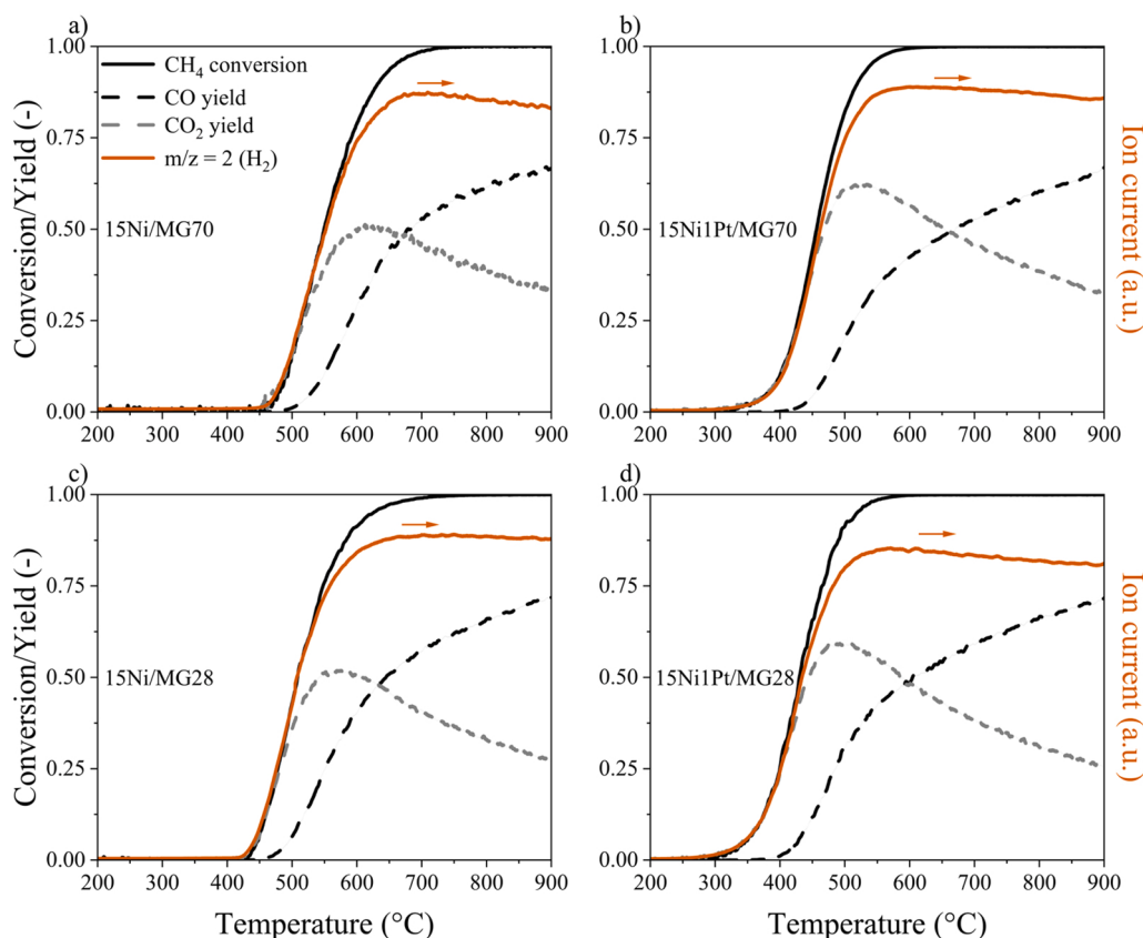
Fig. 4. Catalytic activity during light-off (LOff) in reaction mixture (RM, 0.66 vol% CH 4 , 2 vol% H 2 O, N 2 balance) after pre-reduction. a) 15Ni/MG70, b) 15NiPt/MG70, c) 15Ni/MG28, d) 15NiPt/MG28.
