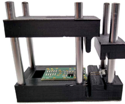
(b) Flasher in the jig used to bend the LED and solder it to the PCB.
