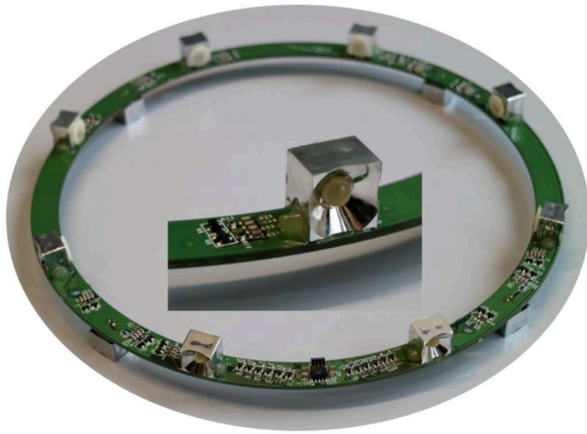
(a) The flasher daisy chain for each D-Egg is realized on one large, 115 mm outer diameter, annular PCB. Eight LEDs point horizontally outwards. Four LEDs point vertically down. The orientation of each LED is ensured via a commercial, cup-type LED housing.
