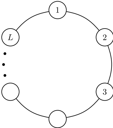
Figure 1: Diagrammatic representation of the circular quiver theory. Each node represents an \mathcal{N} = 2 vector multiplet in the adjoint representation of \text{SU}(N) . Each line connecting adjacent nodes gives rise to an \mathcal{N} = 2 hypermultiplet in the bifundamental representation of \text{SU}(N_i) \otimes \text{SU}(N_{i+1}) . In the case of L = 2 , an additional \text{SU}(2) symmetry arises among the two hypermultiplets connecting the only two gauge nodes.
