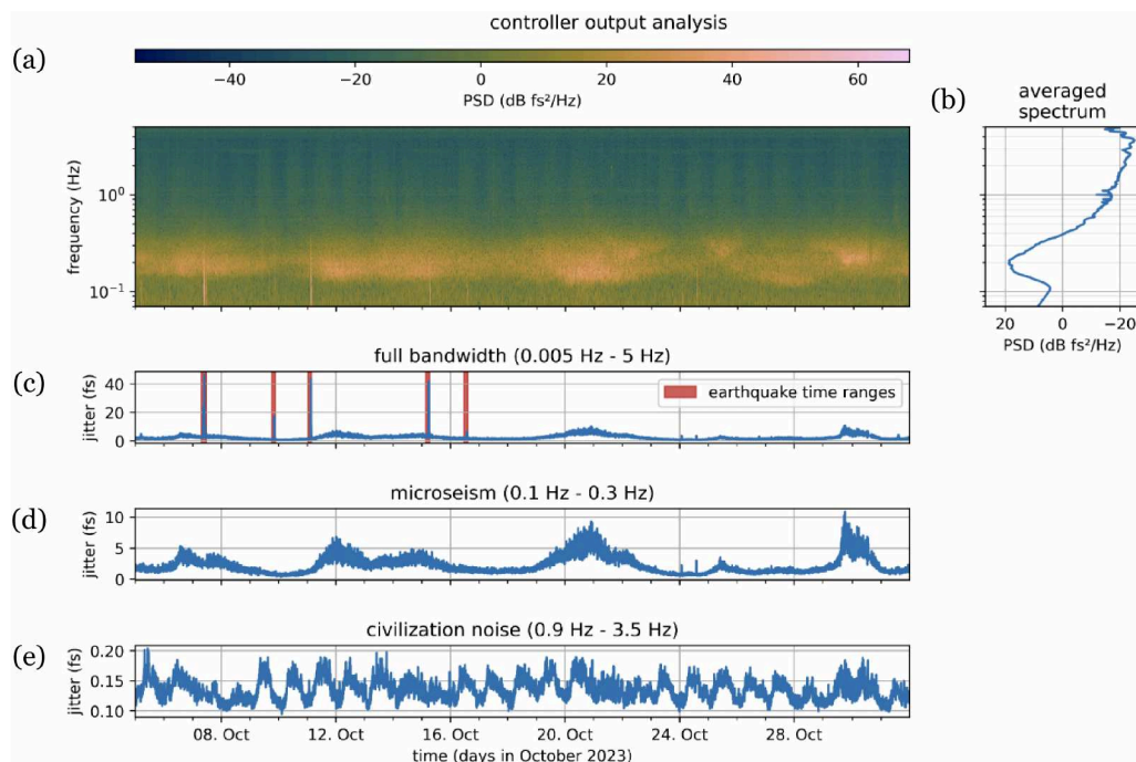
Figure 4: Results of analyzing controller output signal of the 3.5 km link. (a) Spectrogram as of October 2023. (b) Average power spectral density (PSD). (c) Integrated timing jitter over the frequency range 0.005 Hz to 5 Hz. (d) Integrated timing jitter over the frequency range 0.1 Hz to 0.3 Hz, with earthquake effects removed. (e) Integrated jitter over the frequency range 0.9 Hz to 3.5 Hz. Reproduced from [10].
