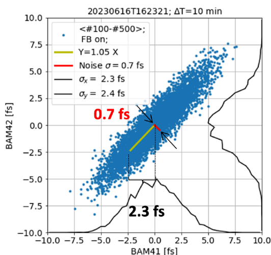
Figure 2: Correlation of electron bunch arrival time measured with two adjacent monitors downstream of the main linac of the European XFEL. The monitors are provided with an optical reference from the main laser oscillator of the facility, and the subsidiary reference laser oscillator of the facility, respectively, while the subsidiary reference laser oscillator is synchronized to the main one via another optical fiber link.
