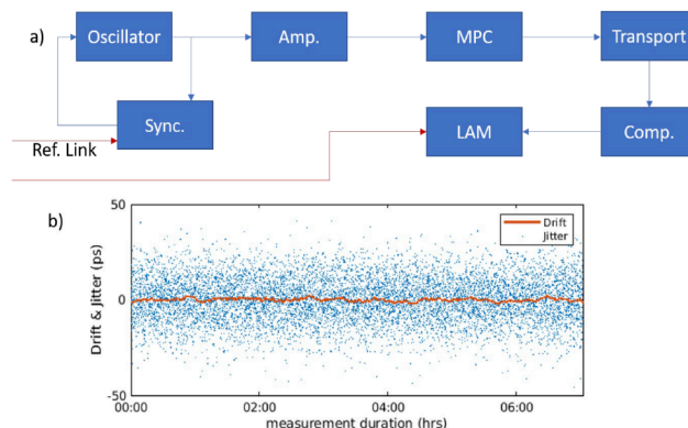
Figure 3: Laser pulse arrival time measurement at FLASH FL23. a) Schematics of the setup. The pump-probe laser's seed oscillator is synchronized (Sync.) to the optical reference (Ref. Link), while the laser amplifier, transport, compression scheme (MPC, transport, Comp.) may introduce timing jitter and drift, measured using a laser pulse arrival time monitor (LAM), which is also referenced to the optical reference. b) With a active feedback, the peak-to-peak arrival time drift (red line, moving average) is determined to be less than femtosecond over the measurement period of 7 hours. Reproduced from [7].
