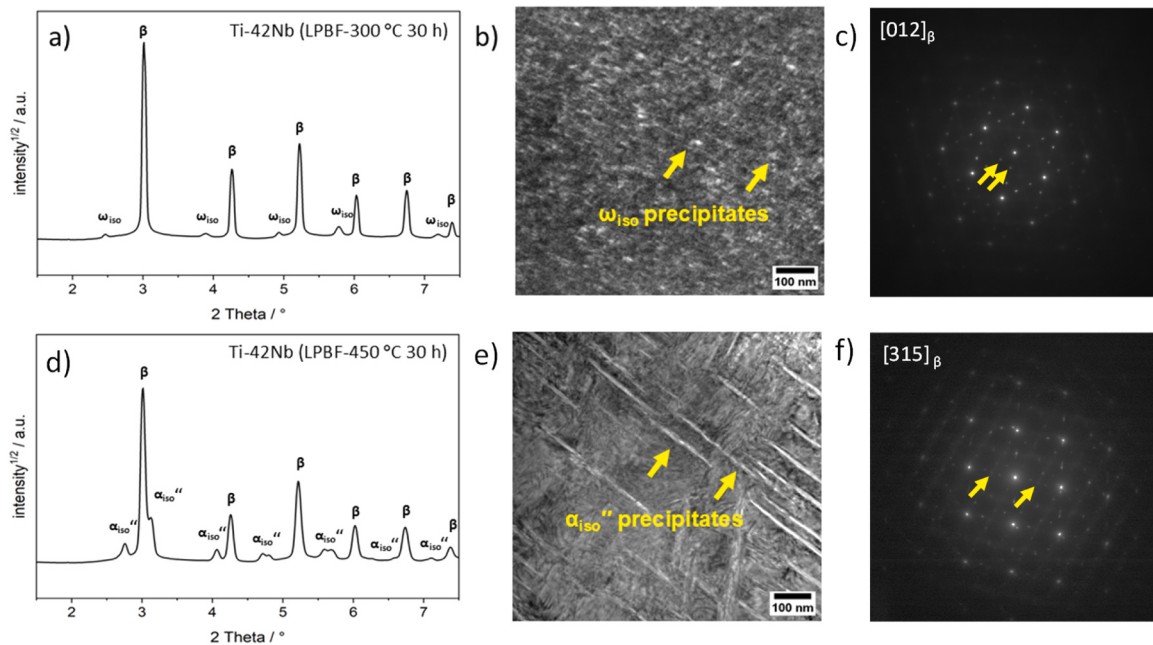
Fig. 1. X-ray diffraction (SXRD) analysis and corresponding TEM images for heat-treated LPBF-produced Ti-42Nb alloys. Images a) and b) belong to the Ti-42Nb (LPBF-300 °C 30 h), and d) and e) belong to the Ti-42Nb (LPBF-450 °C 30 h) alloy states. Additionally, the diffraction patterns for c) Ti-42Nb (LPBF-300 °C 30 h) and f) Ti-42Nb (LPBF-450 °C 30 h) alloy states are represented.
