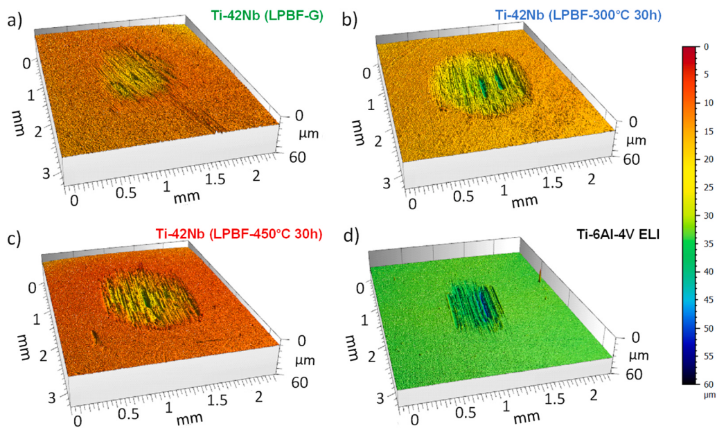
Fig. 8. 3D optical profilometry images of the wear tracks formed under OCP conditions for a) Ti-42Nb (LPBF), b) Ti-42Nb (LPBF-300 °C 30 h), c) Ti-42Nb (LPBF-450 °C 30 h), and d) Ti-6Al-4V ELI alloy states.
