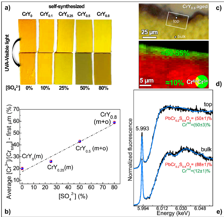
Fig. 31 a Photographs of oil mock-up paints made up of self-synthesized chrome yellow powders differing in sulfate content (CrY x denotes PbCr 1-x S x O 4 with 0 \leq x \leq 0.8 ) and crystalline structure [monoclinic (m) and/or orthorhombic (o)] before (top) and after (bottom) exposure to UVA-VIS light. b Cr 3+ -abundance percentage (averaged at the uppermost micrometer of the paint surface) vs. sulfate amount percentage obtained from the light-exposed mock-up paints. Dashed line shows the linear trend. c Photomicrograph of a thin section obtained from the self-synthesized CrY 0.8 paints aged by UVA-VIS light (top) and d corresponding RG composite Cr 6+ /Cr 3+ maps. e Result of the linear combination fit (cyan) of the \mu -XANES spectra of PbCr 0.2 S 0.8 O 4 and one/two Cr 3+ -references [namely: Cr(OH) 3 /Cr 2 O 3 and Cr 3+ -acetate/Cr 3+ -acetylacetonate] to the ones recorded from the surface of the uppermost alteration layer and the bulk paint of the CrY 0.8 thin section (black) shown in (e) (data of (e-e) were collected at ESRF-ID21). Adapted with permission from [38, 145, 548]
