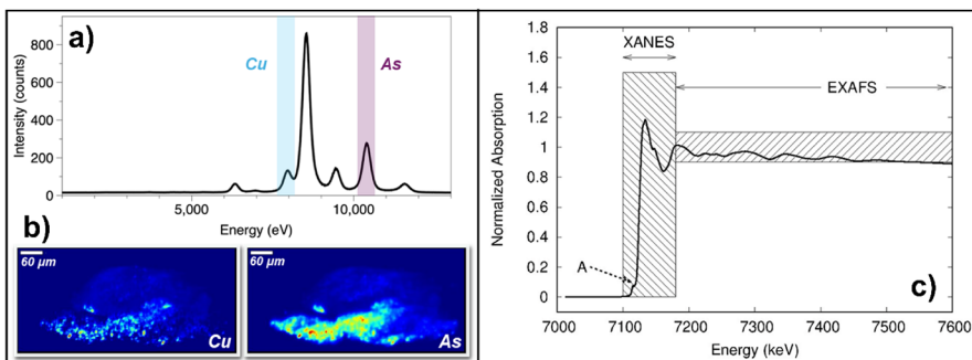
Fig. 4 Examples of a XRF spectrum, b 2D \mu -XRF maps (here the Cu and As maps of a paint cross-section), and c the EXAFS and XANES regions in a Fe _2 O _3 (hematite) XAS spectrum collected at ESRF-BM08-LISA beamline with a Si (111) monochromator
