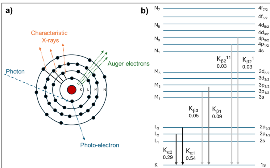
Fig. 3 a Excitation of an atom by an X-ray via the photoelectric effect. The ionization of the atom leads to the decay from the excited state by an electron from a higher energy level, leading to the emission of either a fluorescent X-ray or Auger electron. b Diagram of K shell radiative decays and their respective X-ray emission lines and rate
