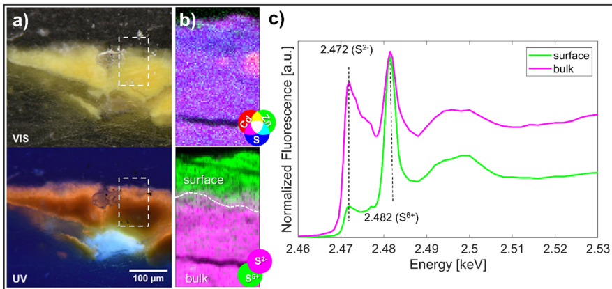
Fig. 29 a Visible and UV light micrographs of a cross-section taken from an unaltered painting by Joan Miró. The surface of the paint layer shows the orangish emission sometimes observed in altered cadmium yellow paints. b RGB composite SR \mu -XRF maps of Cd/Zn/S (top) and S^{2-}/S^{6+} . c Average S K-edge XANES spectra extracted from S^{2-} and S^{6+} rich areas of (b) (data collected at ESRF-ID21). Adapted from [135]
