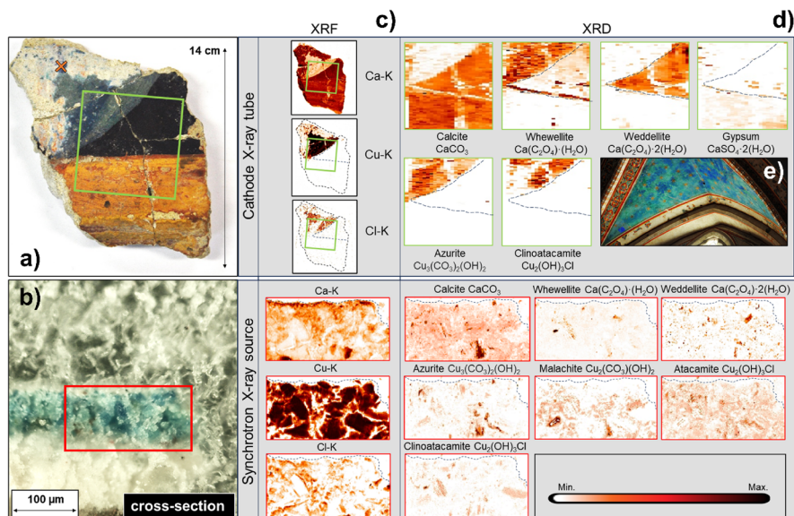
Fig. 21 a Painted fragment CA26 from the one of the discolored vault of the upper Basilica di San Francesco in Assisi (late thirteenth century, Italy) shown in (e) . The orange cross indicates the spot of the sample used to obtain the paint cross-section illustrated from the photomicrograph of (b) . c XRF maps of selected key elements. Top, MA-XRF: area ( h \times v ) = 50 \times 50 \text{ mm}^2 , step size ( h \times v ) = 0.3 \times 0.3 \text{ mm}^2 , exposure time = 0.3 s/pt, reflection geometry, energy = 20.04 keV. Bottom, SR \mu -XRF: area ( h \times v ) = 290 \times 100 \mu\text{m}^2 , step size ( h \times v ) = 1 \times 1 \mu\text{m}^2 , exposure time = 1 s/pt reflection geometry, energy = 21 keV. d XRD maps of selected primary compounds and secondary products (weddellite, whewellite, atacamite, clinoatacamite). Top, MA-XRD: area ( h \times v ) = 25 \times 24 \text{ mm}^2 , step size = 1 \times 0.3 \text{ mm}^2 , exposure time = 10 s/pt, reflection geometry, energy = 8.04 keV. Bottom, SR \mu -XRD: area ( h \times v ) = 290 \times 100 \mu\text{m}^2 , step size ( h \times v ) = 1 \times 1 \mu\text{m}^2 , exposure time = 1 s/pt, transmission geometry, energy = 21 keV
