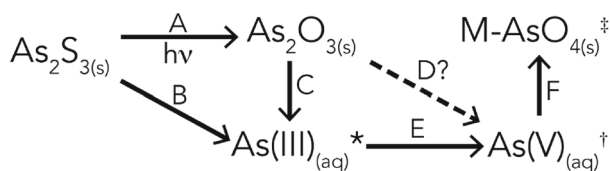
Fig. 24 Overall degradation pathways of orpiment in paintings. *As(III): arsenites in various species in solution (e.g., \text{AsO}_3^{3-}(\text{aq}) , \text{HAsO}_3^{2-}(\text{aq}) , \text{H}_2\text{AsO}_3^-(\text{aq}) , or \text{H}_3\text{AsO}_3(\text{aq}) ). † As(V): arsenates with different forms in solution ( \text{H}_3\text{AsO}_4(\text{aq}) , \text{H}_2\text{AsO}_4^-(\text{aq}) , \text{HAsO}_4^{2-}(\text{aq}) , or \text{AsO}_4^{3-}(\text{aq}) ). ‡ Metal arsenates. Adapted from [183]
