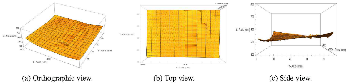
Figure 4. Tilt corrected surface map of a barrel module. The tilt corrected data yields a shape coefficient of +51 \mu\text{m} . The tilt correction generally has a negligible effect on the calculated shape coefficient, suggesting that the placement of the modules during measurement does not distort the calculated shape coefficients.
