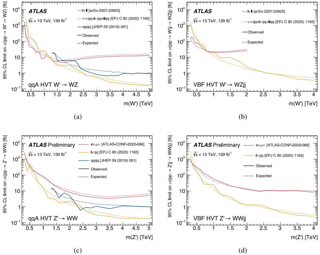
Fig. 27. Upper limits on the production cross section of new gauge bosons, (a, b) W' or (c, d) Z' decaying into a (yellow) VV semileptonic final state [164], (red) leptonic final state [166,167], or (blue) hadronic final state [165]. The HVT model is used to define the signal hypothesis. The qqA and VBF production modes are considered separately.
