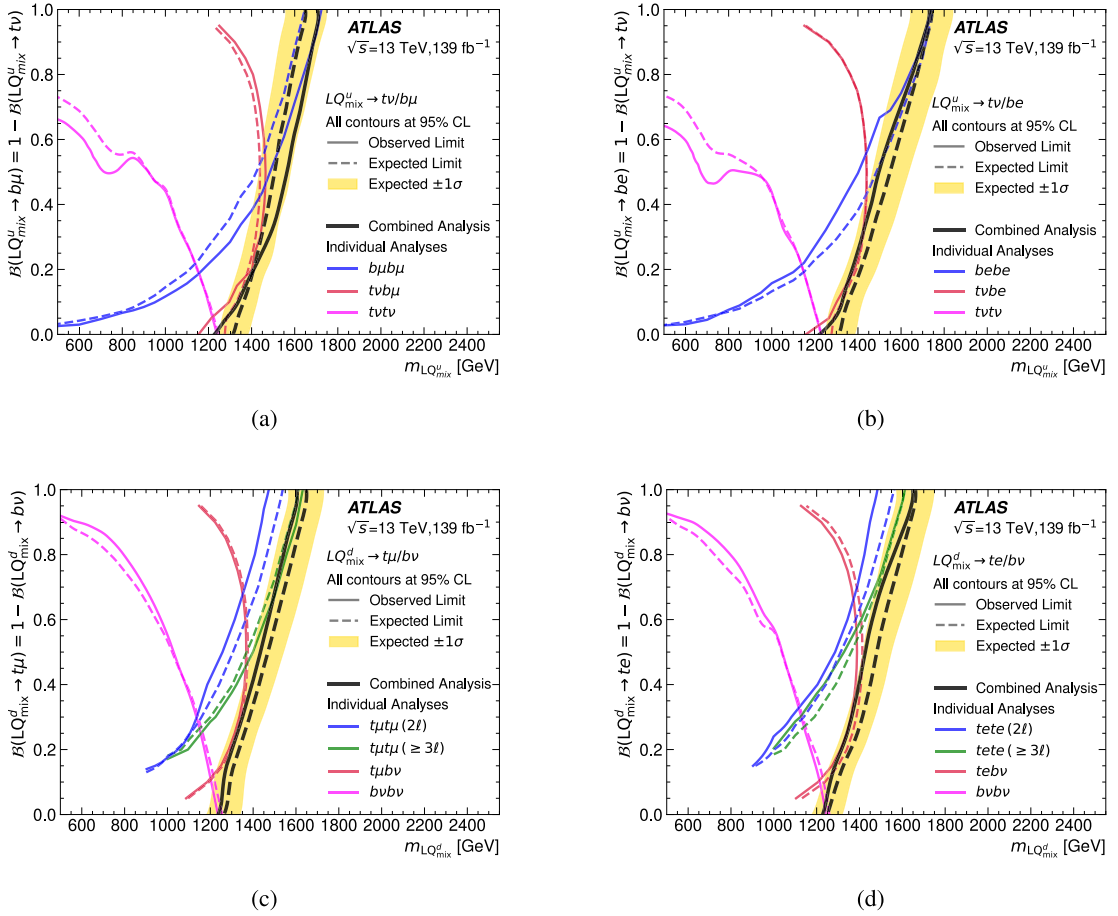
Fig. 24. Two-dimensional limits (a, b) on the production of up-type scalar leptoquarks with cross-generational couplings as a function of the mass of the LQ and the BR to b\ell from the search of up-type LQs in final states with (blue) two leptons [145], (red) only one lepton [147], (pink) no leptons [140] and (black) their statistical combination [146], and (c, d) on the production of down-type scalar leptoquarks with cross-generational couplings as a function of the mass of the LQ and the BR to t\ell from the search of down-type leptoquarks in final states with (blue) two leptons [144], (green) multiple leptons [148], (red) only one lepton [147], (pink) no leptons [140] and (black) their statistical combination [146]. Electron and muon final states are considered separately.
