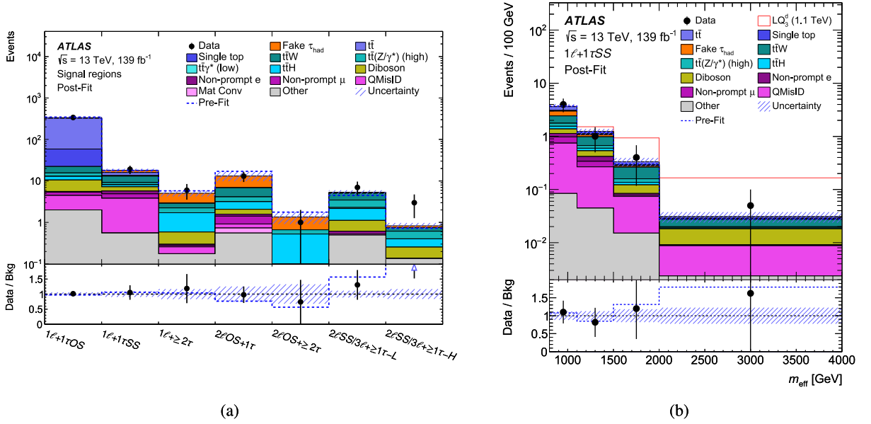
Fig. 17. (a) Event yields in all signal regions and (b) the distribution of m_{eff} in one of the signal regions used in the search for LQLQ \rightarrow tt\tau\tau [136]. The distributions are shown after a background-only fit.
