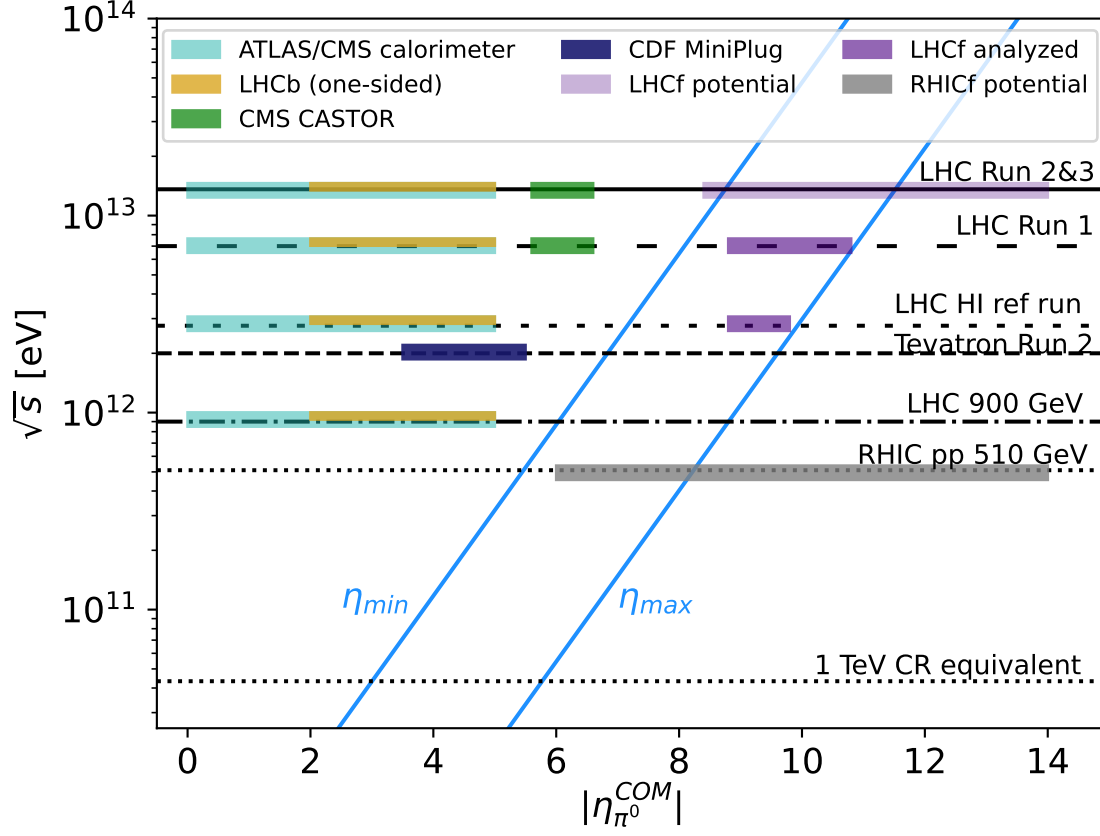
FIG. 4. Relevant |\eta_{\pi^0}^{\text{COM}}| region in the center of mass frame for gamma-ray like air showers from cosmic rays (light blue lines). The black horizontal lines correspond to available data in terms of center of mass energy and the colored boxes indicate the |\eta| coverage of the corresponding experiments. The label “potential” refers to LHCf and RHICf data that has already been recorded but not published.
