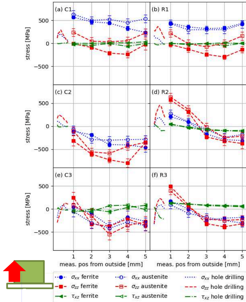
Figure 4: Residual stresses determined on the six positions of the additively manufactured sample.
