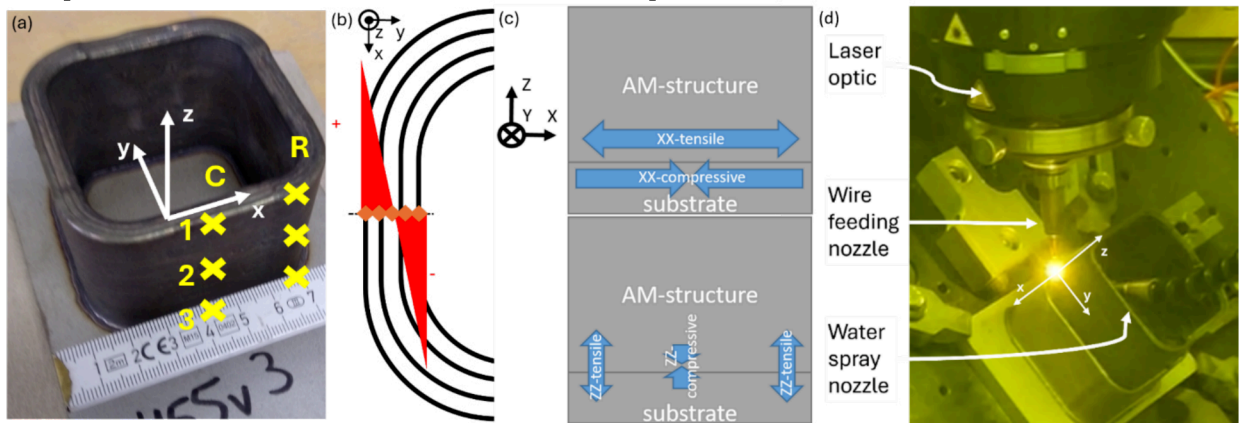
Figure 1 (a) Sample geometry with strain measurement locations, (b) expected residual stress distribution in a single layer, (c) global residual stress distribution in the whole part and (d) Cladding build strategy.
