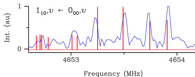
Fig. 6 Comparisons between the observed spectrum and a calculated stick spectrum, plotted as a function of the frequency in MHz, for the hyperfine structure of the transitions 1_{10,v} \leftarrow 0_{00,v} , with v = 0 and 1. These transitions being forbidden, their hyperfine components gain strength through mixings due to the hyperfine coupling Hamiltonian. The lists of predicted hyperfine transitions are given in Table S2 of the ESI.†
