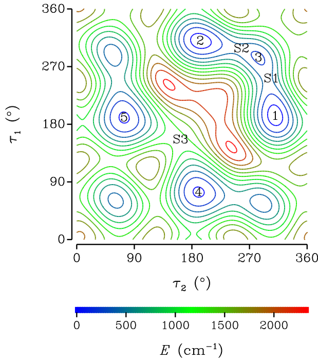
Fig. 2 The relaxed two-dimensional potential energy surface of CDA as a function of the dihedral angles \tau_1 and \tau_2 . Contour lines corresponding to equally spaced energy values with a spacing of 200 \text{ cm}^{-1} are drawn from 100 to 2300 \text{ cm}^{-1} . 5 minima numbered 1 through 5; and 3 saddle points labeled S1, S2, and S3 can be seen.
