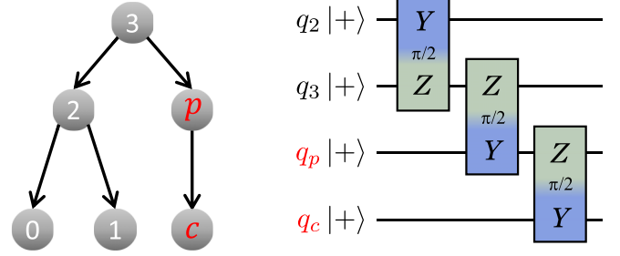
FIG. 10. Illustration for the proof of Theorem 1. The rightmost ZY exponential e^{-i(\pi/4)Z_pY_c} on the parent node p and the child node c rotates the state |\phi\rangle = \frac{1}{\sqrt{2}}(|10\rangle_{23}|1\rangle_p + |01\rangle_{23}|0\rangle_p)|+\rangle_c|++\rangle_{01} to \frac{1}{\sqrt{2}}(|10\rangle_{23}|1\rangle_p|0\rangle_c + |01\rangle_{23}|0\rangle_p|1\rangle_c)|++\rangle_{01} . This circuit is a subcircuit of the one shown in Fig. 3(a).
