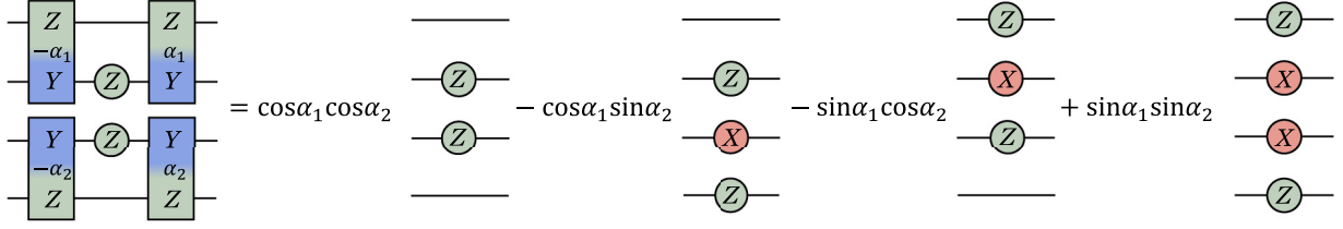
FIG. 17. Schematic calculation of the observable Z_i Z_j conjugated by two ZY gates. Each circle denotes a single-qubit Pauli operator and each rectangle denotes a matrix e^{-i\alpha ZY/2} with the value of \alpha shown at the center of the rectangle.
