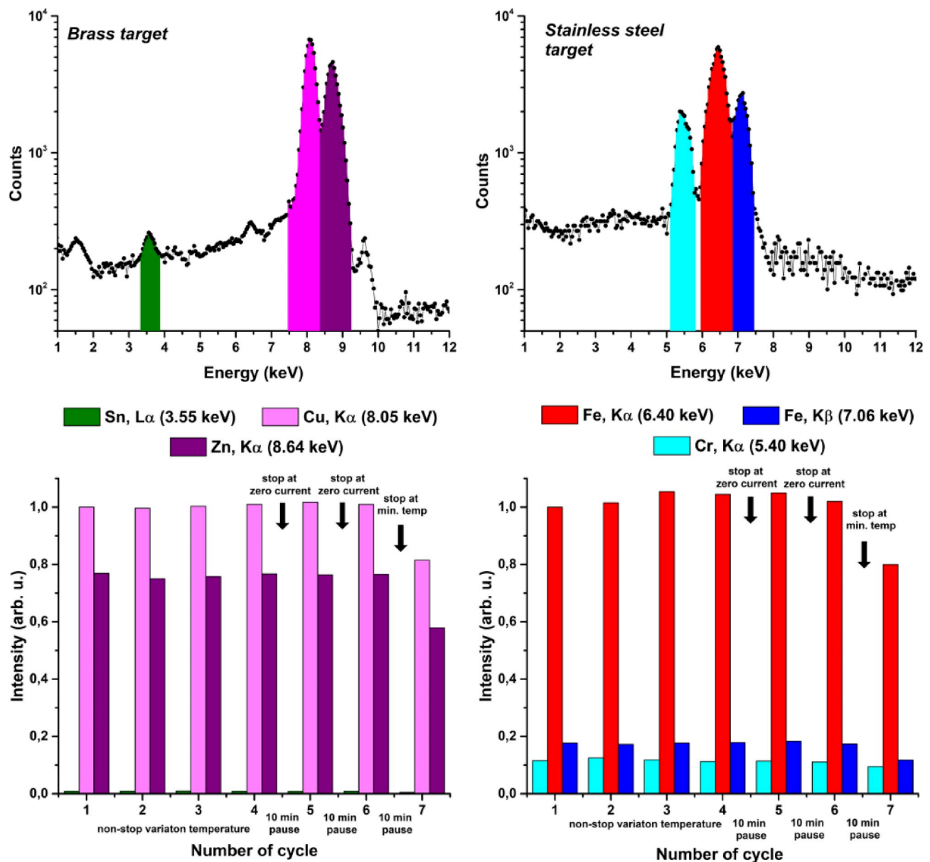
Fig. 5. Stability of Energy-Dispersive X-ray Spectroscopy. (a) and (b) present typical X-ray spectra from brass and stainless steel targets respectively. Marked areas confine photon counts corresponding to characteristic X-rays lines of target elements. (c) and (d) present a histogram of dynamic change of intensity of highlighted regions in X-ray spectra for brass and stainless-steel targets respectively. The unity in intensity scale is 6.4 \cdot 10^4 counts (c) and 6.35 \cdot 10^4 counts (d). The horizontal scale represents the thermal cycle number. The fifth and sixth cycles were observed after the measurement were stopped at zero current in the circuit and paused for 10 min. The seventh cycle was observed after the measurements were stopped at minimum temperature and paused for 10 min. The background count during the measurements was a small fraction of a percent.
