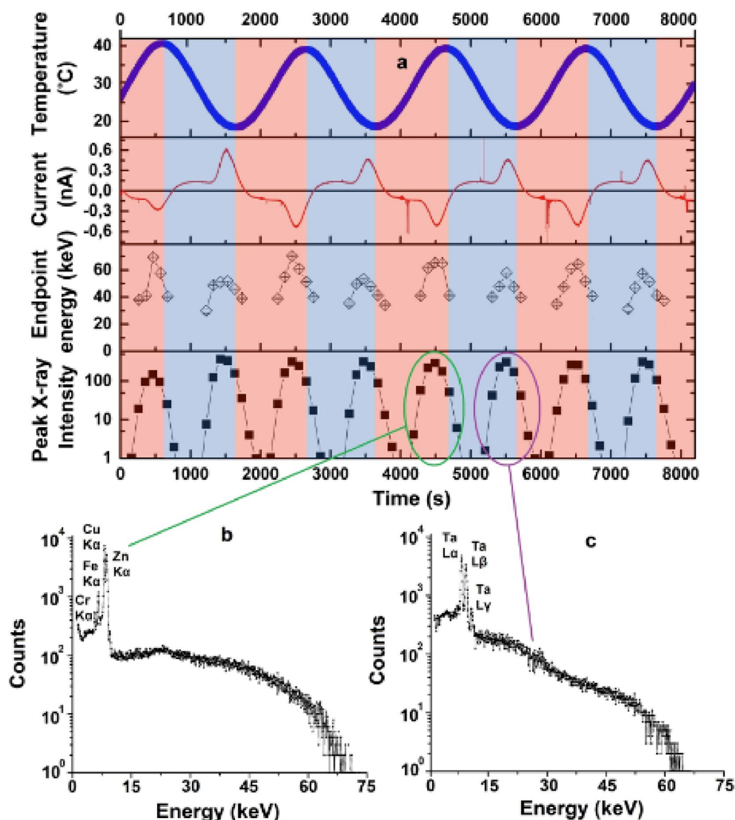
Fig. 1. Results of the measurements for 0.5 mHz temperature variation frequency and 1.0–2.5 mTorr pressure range. (a) Four graphs from top to bottom: temperature in the close vicinity of the top surface of the crystal; current in the circuit; endpoint energy of the X-ray spectrum; X-ray intensity integrated over 100 s. Blue areas correspond to the cooling phase, red areas correspond to heating phase. Two lower graphs present the X-ray spectra accumulated over a half cycle at negative (b) and positive (c) polarities. The characteristics X-ray lines are marked in the graphs.
