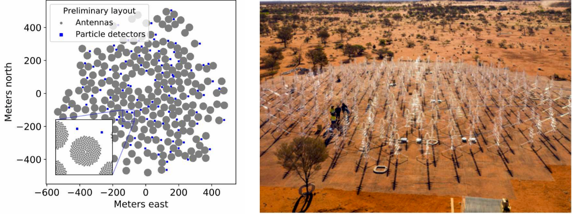
Figure 1: Left: The SKA-Low core plus satellite stations. Each gray circle indicates a station of 256 antennas. The squares indicate foreseen positions of the SKA-Low particle detectors consisting of a dense core, a ring around the core, and additional detectors near the satellite stations. Exact locations are still subject to discussion. Right: Picture of the first SKA-Low station with 256 antennas (SKAO Observatory).
