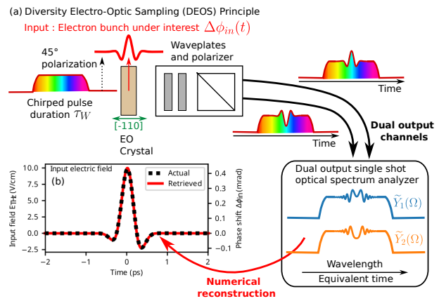
Figure 2: Conceptual validation of the DEOS strategy for electron beam diagnostics.
